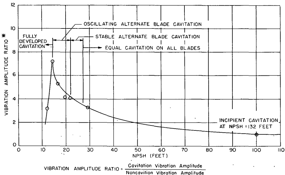
Fig. D2 - Cavitation vibration data of 14.6-degree helical inducer (amplitude measurements with vibration pickup on test section)
