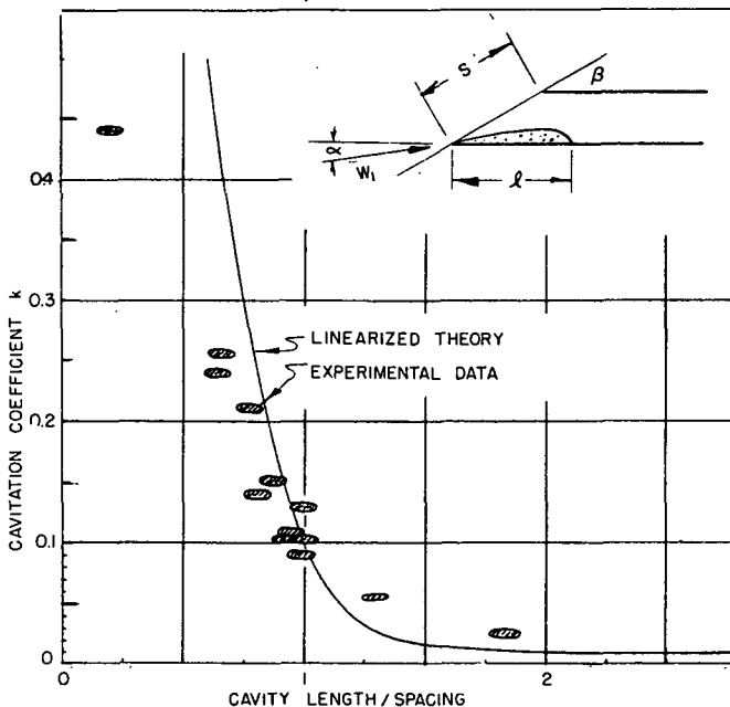
Fig. 17 - Growth of a partial cavity in a cascade as a function of cavitation number. The angle of attack and blade angle correspond to the mean radius of the 90^\circ impeller at a flow coefficient of \phi = 0.093 .
