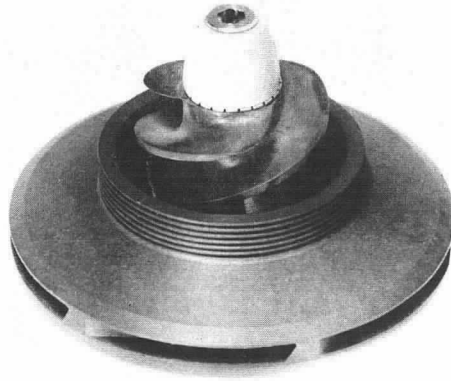
Fig. 1 - A typical inducer installation on a centrifugal pump for liquid oxygen. (Courtesy of Mr. T. Carter, Turbocraft Corp., Pasadena.)
