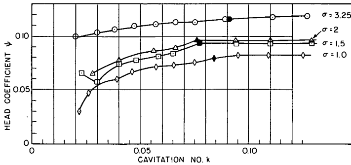
Fig. 15 - The effect of solidity on the cavitating performance of a 9^\circ helical inducer at a flow coefficient of \phi = 0.093 . The solid symbols denote inception of oscillating cavitation.
