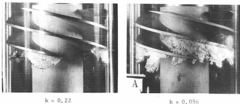
Fig. 11 - Cavitation on the 12° inducer at a flow coefficient of \phi = 0.10 . The confused flow pattern at the lower cavitation number is typical of nonsteady oscillating cavitation.
