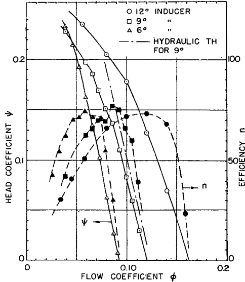
Fig. 6 - Noncavitating efficiency and head coefficient vs flow coefficient for a 6°, 9°, and 12° helical inducer (impellers 12, 3, and 2) and solidity of 2.5
