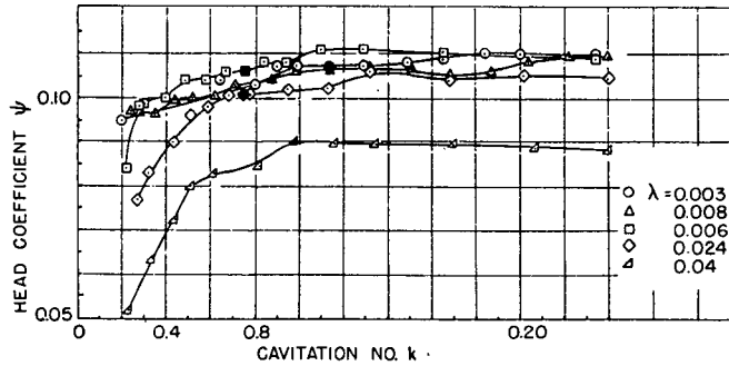
Fig. 14 - The effect of tip clearance on the cavitating performance of a 9^\circ inducer with a solidity of 2.5 at a flow coefficient near the best efficiency point ( \phi = 0.093 ). The solid symbols indicate inception of oscillating cavitation.
