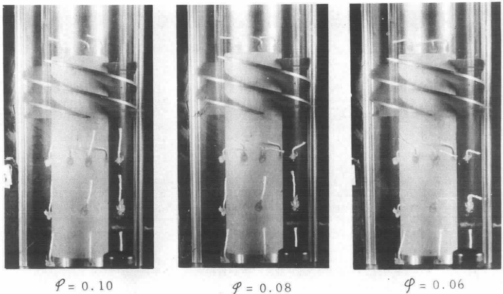
Fig. 5 - Sequence of tuft photographs on a 12^\circ impeller at various flow rates. The rotation is from left to right and flow approaches the rotor from below.
