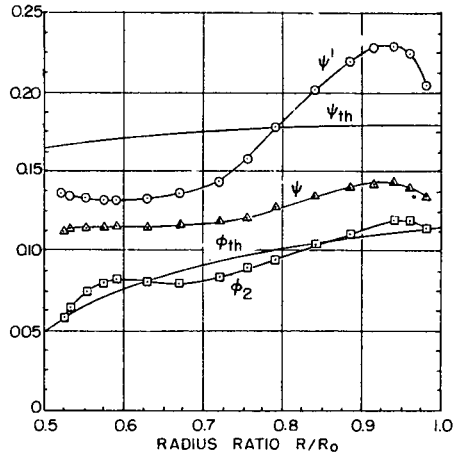
Fig. 7 - Measured axial velocity profile \phi_2 , measured head coefficient \psi , measured input head coefficient \psi_{th} , theoretical axial velocity, and theoretical head coefficient distributions across the annulus of a 9° helical inducer at a mean flow coefficient of \phi = 0.093
