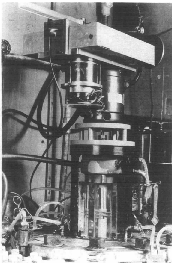
Fig. 4 - View of test facility showing the Lucite working section and the drive motor. The discharge piping and manometers are not visible.
