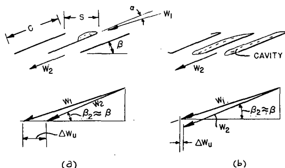
Fig. 16 - Velocity triangles in a flat plate cascade (a) without and (b) with extensive cavitation
