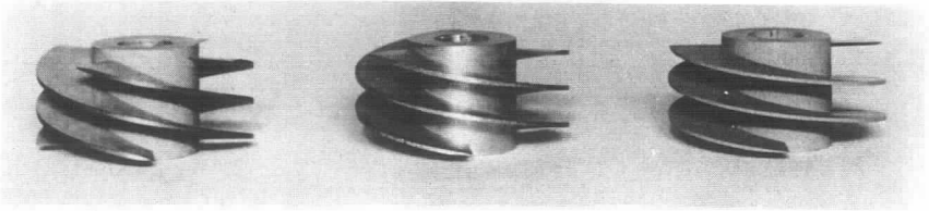
Fig. 2 - The 6°, 9°, and 12° experimental inducers. The tip diameter is 2 inches.
