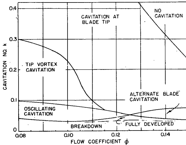
Fig. 13 - The various modes of cavitating flow in a 12° helical inducer as a function of cavitation number and flow coefficient
