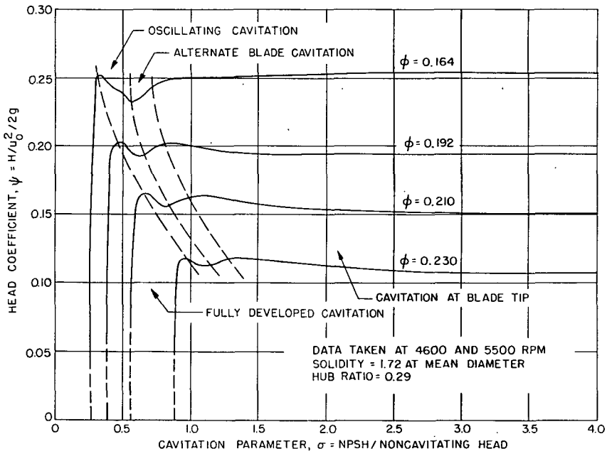
Fig. D1 - Cavitation performance of 16.2-degree (at tip) four-bladed helical inducer
