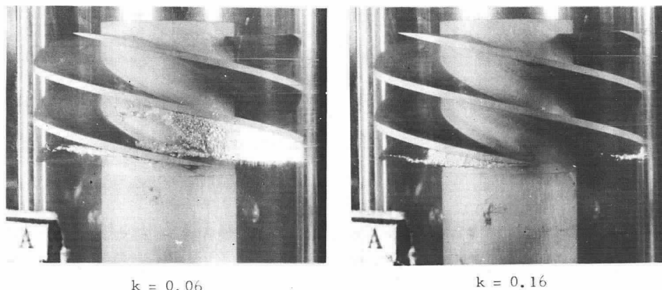
Fig. 10 - Cavitation on the 12° inducer at a flow coefficient of \phi = 0.14 , showing the occurrence of alternate blade cavitation
