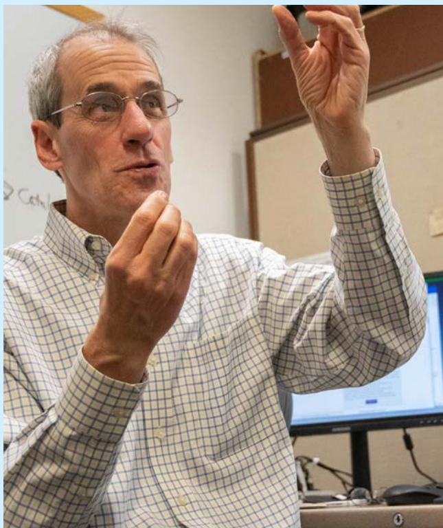
U.S. Naval Research Laboratory Research physicist Liam Healy explains a model for a velocity distribution of fragmenting satellite debris. Photo by Emanuel Cavallaro
