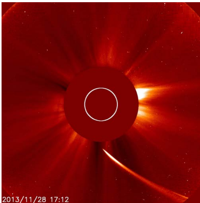
This image from NRL's Large Angle Spectrometric Coronagraph (LASCO) telescope onboard the Solar and Heliospheric Observatory (SOHO) spacecraft shows comet ISON as it approaches the sun. The sun is blocked by LASCO's central occulting disk with a white circle indicating the Sun's position and scale. ISON reached perihelion, its closest approach to the Sun, on 28 November 2013, at 18:45 UT. The comet passed just over 1 million kilometers above the solar surface. Image by NASA/ESA/NRL
