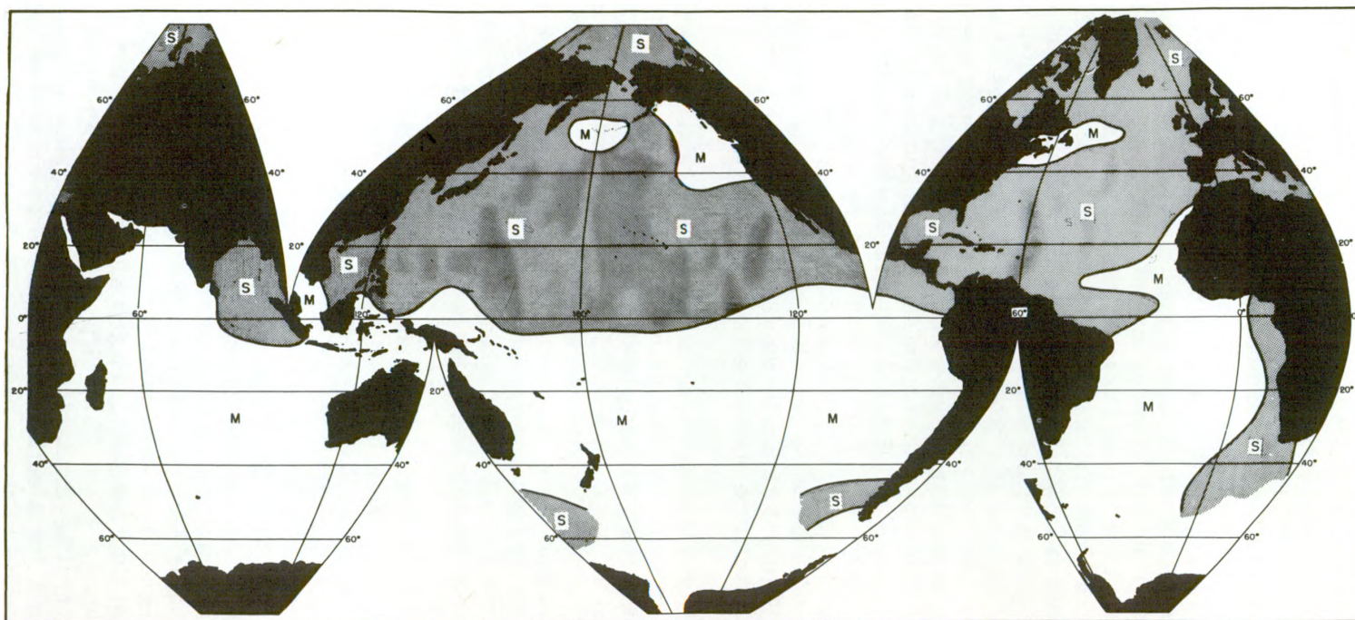
Figure 2--Mean sea level deviation during spring and fall. Areas are shaded and labeled "S" if sea level is higher than average during September, unshaded and labeled "M" if higher than average values are observed in March.
