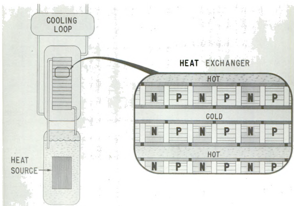
Figure 4--Thermoelectric power source.
