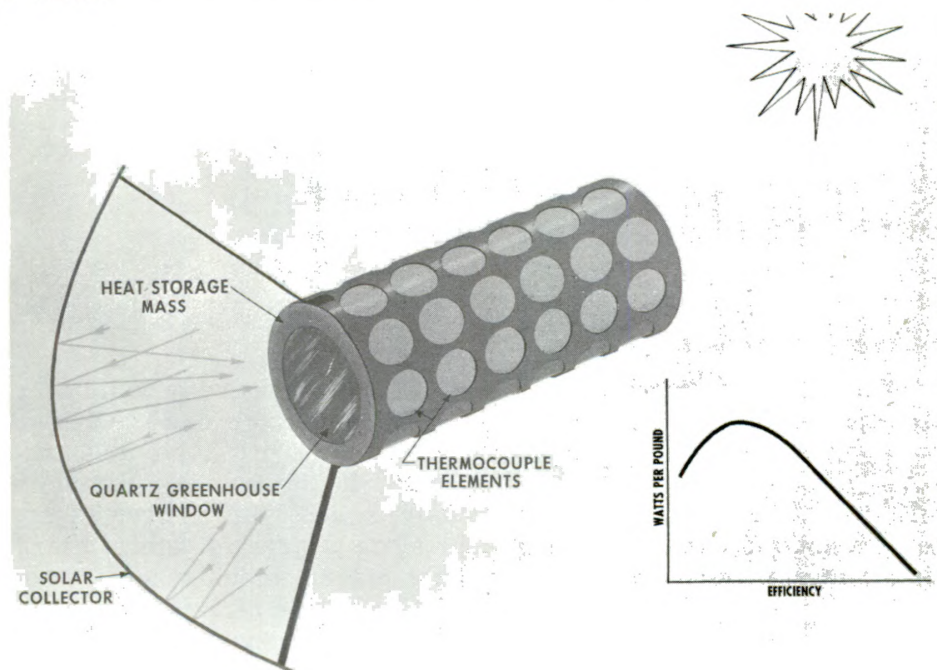
Figure 2--Solar thermal power supply.
