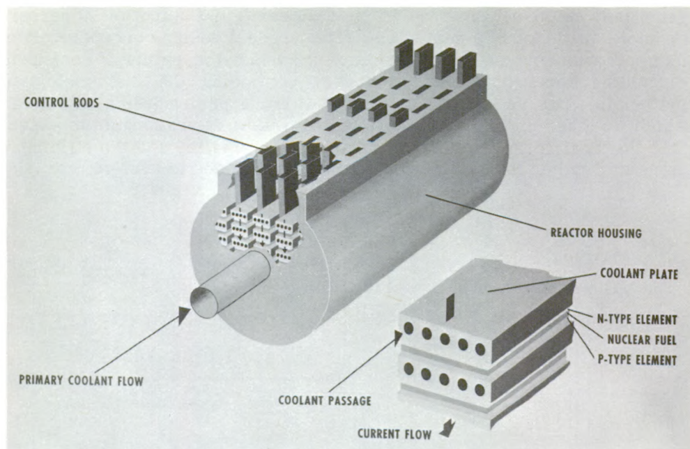
Figure 5--In-pile thermoelectric generator.
