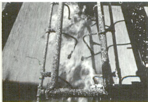
Figure 7 and 8--Evidence that the foam works: two motion picture frames of a drag-run through foam and immediately afterwards on dry concrete. Ignition occurred 2-1/2 seconds after leaving the foam.
