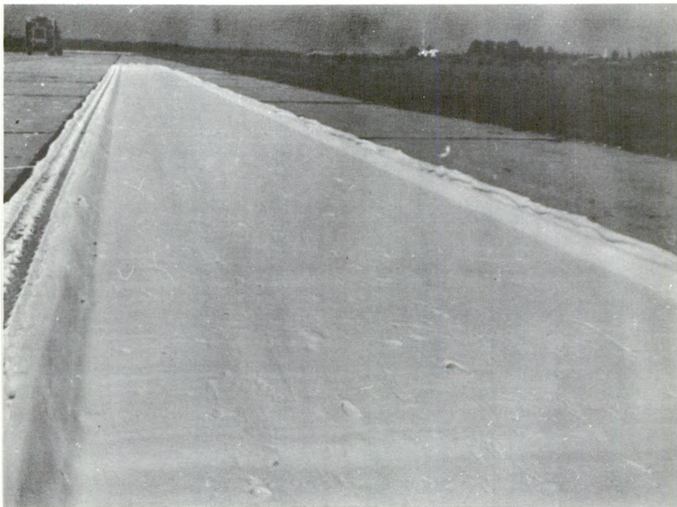
Figure 5--A finished foam test strip, 4 feet wide by 400 feet long, laid on a concrete runway.
