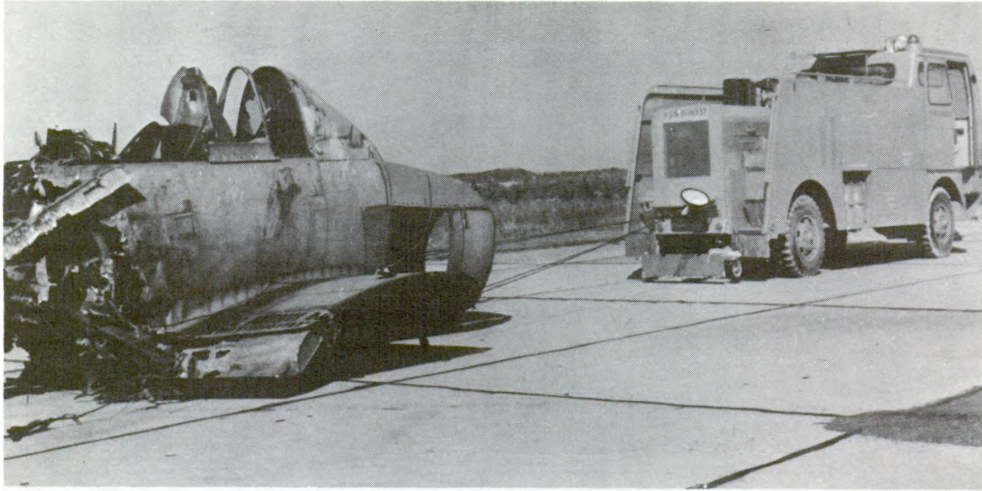
Figure 3--Aircraft towing tests showing hydraulic scale for measuring drag resistance
