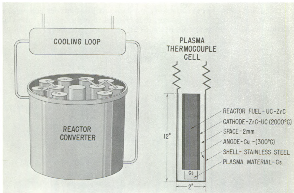
Figure 6--Nuclear thermionic converter.
