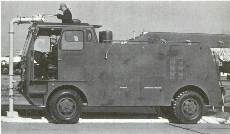
Figure 4--The MB-5 vehicle rigged for laying a foam strip, showing the spreader at the rear for smoothing the foam to a uniform depth. This vehicle loads 400 gallons of water and foams 4000 square feet of runway in 2 minutes. The MB-1, a similar vehicle with larger tanks, loads 1000 gallons (10,000 square feet).
