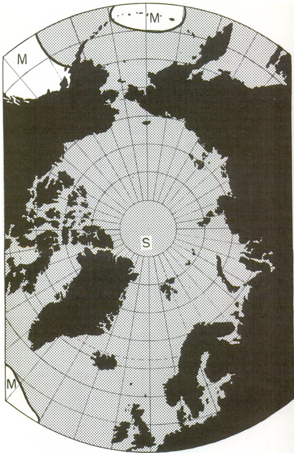
Figure 4--Sea level deviation in the Arctic during spring and fall.
