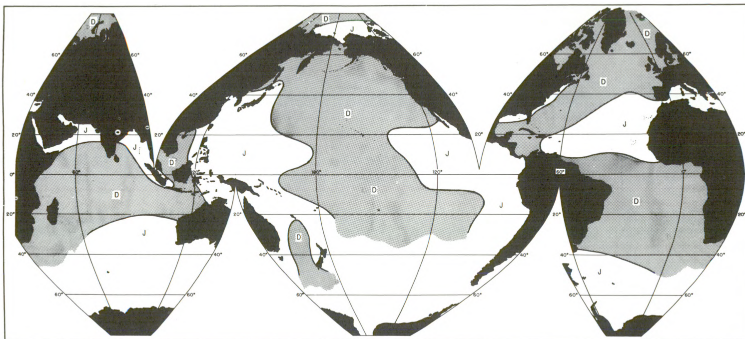
Figure 3--Mean sea level deviation during summer and winter. Areas are shaded and labeled "D" if sea level is higher than average during December, unshaded and labeled "J" if higher than average values are observed in June.
