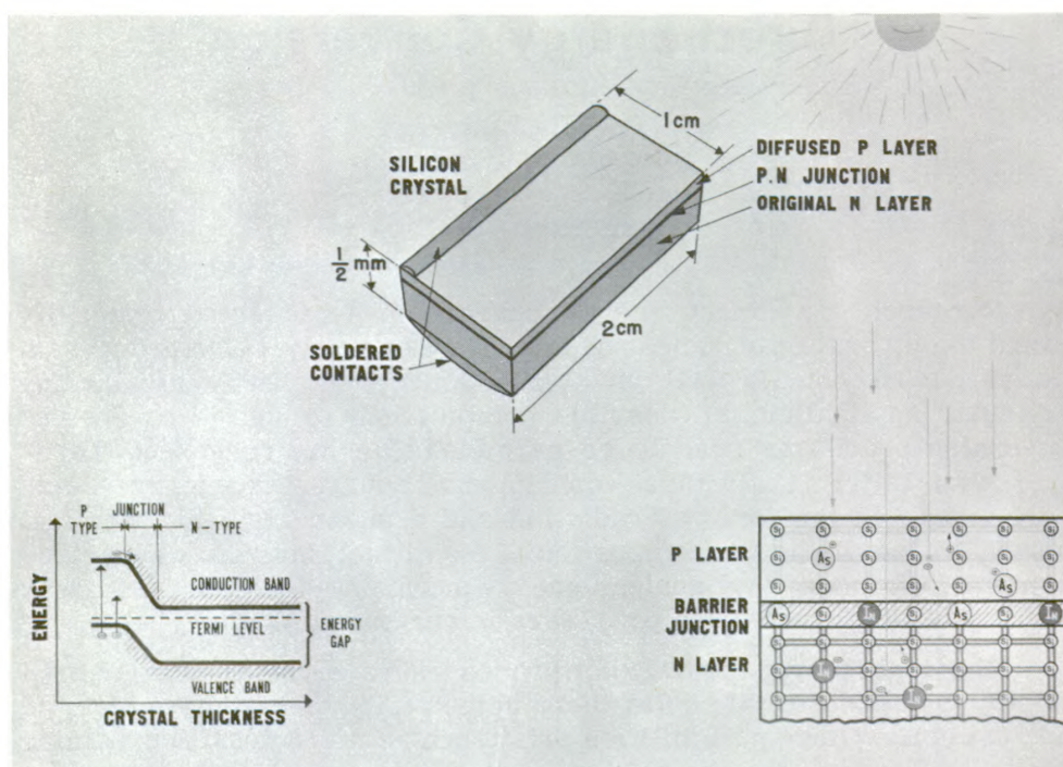
Figure 1-- Solar cell.
