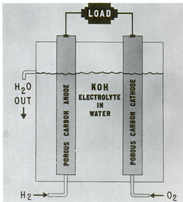
Figure 7--Hydrox fuel cell.
