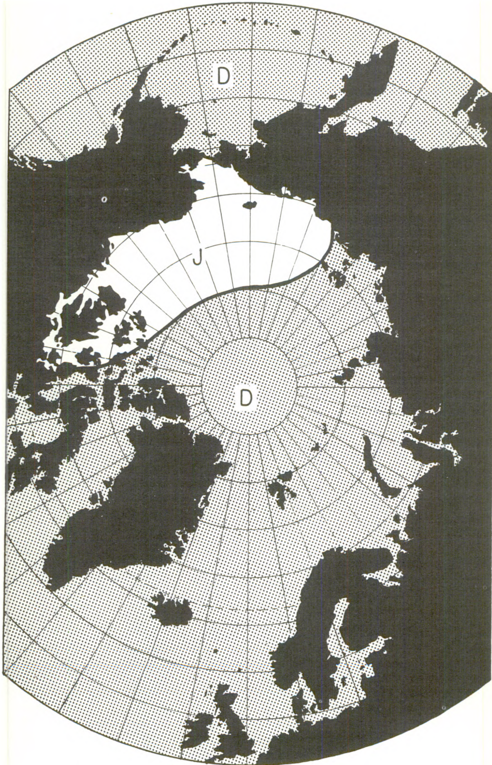
Figure 5--Sea level deviation in the Arctic during summer and winter.
