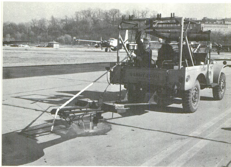
Figure 1--Rig for dragging metal specimens (or "shoes") along a runway showing metal "shoes," gasoline nozzles, and hot-wire probe for measuring ignition temperatures.
