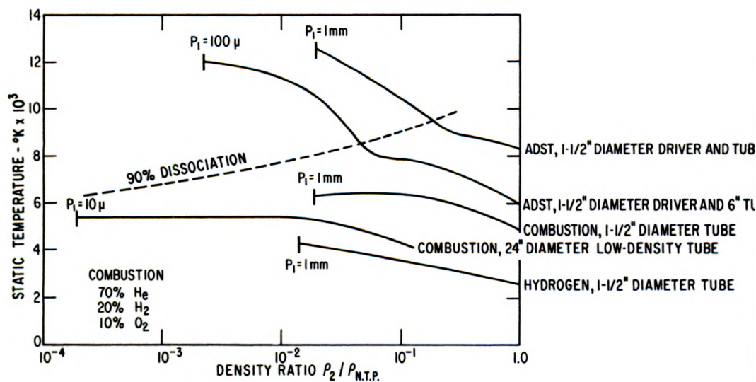
Figure 1 — Temperatures and densities (after equilibration) obtainable in air behind the incident shock for various types of diaphragm shock-tube drivers. The driver pressure is limited to 10,000 pounds per square inch for the ADST (arc driven shock tubes) and the combustion drivers and to 2000 psi for the hydrogen driver. The dotted line marked "90% Dissociation" denotes region above which 90 percent of gas molecules are dissociated into atoms.
