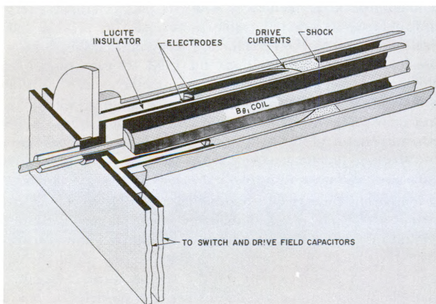
Figure 6 — Schematic drawing of the Magnetic Annular Shock Tube (MAST). This device consists essentially of two coaxial cylinders between which a radial electric field is imposed suddenly by switching on a condenser bank. The gas at the left and adjacent to the lucite is preionized, the switch is closed, and, ideally, a radial-drive current sheet is formed uniformly around the annulus. The magnetic field generated by this current sheet drives the gas in the shock tube. A shock wave moves ahead of the driver currents. The tilting of the current sheet is caused by the higher magnetic pressure at smaller radii. The rod down the centerline can be used to produce an azimuthal magnetic field ( B_\theta ), which serves to contain the plasma that has been compressed and heated by the shock. Provision is made also for placing solenoids around the MAST to make possible the use of axial containing fields.
