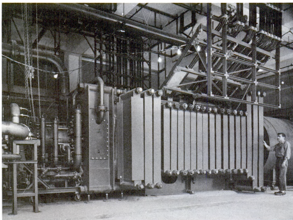
Figure 5 — Mark V 20-megawatt self-excited magnetohydrodynamic generator that employs a modified rocket engine to produce high-temperature ionized gas.
