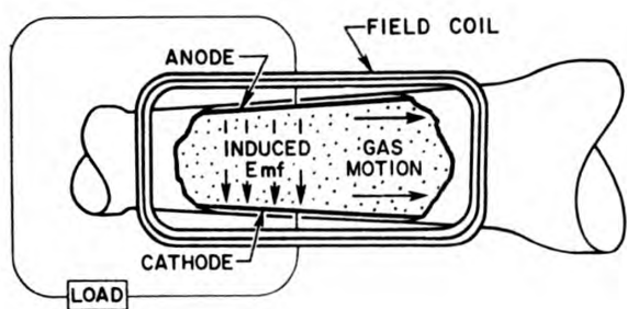
Figure 4 — Schematic of a D.C. magnetohydrodynamic generator. Note that the magnetic field, gas flow, and induced electromotive force (emf) are mutually perpendicular.
