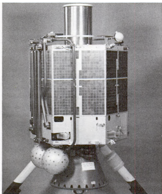
INJUN V spacecraft jointly sponsored by NASA Langley and ONR. Spherical objects are part of folding beam dipole antennas used for VLF (Very Low Frequency) detection experiment.
