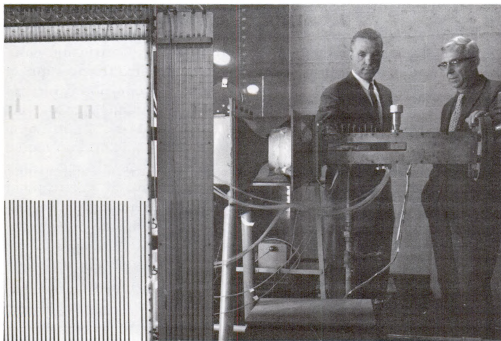
Dr. E. R. G. Eckert (right) and Dr. Richard Goldstein run "film cooling" experiment using supersonic wind tunnel and manometer bank
