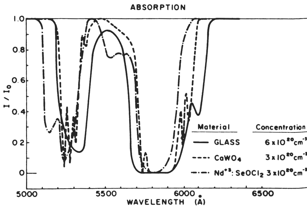
Figure 4 — Absorption spectrum of Nd 3+ in three different host materials
