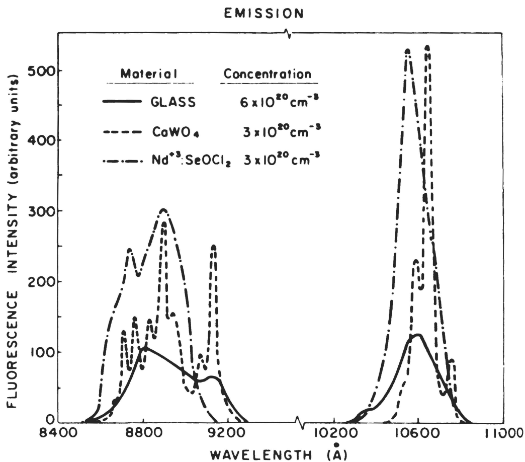
Figure 3 — Fluorescence spectrum of Nd 3+ in three different host materials
