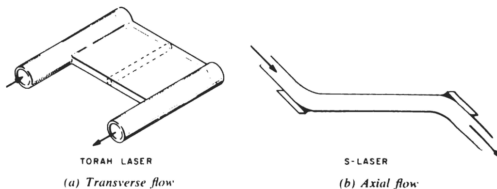
Figure 8 — Schematic drawings of cells with improved hydrodynamic properties. These are now in the design stage.
