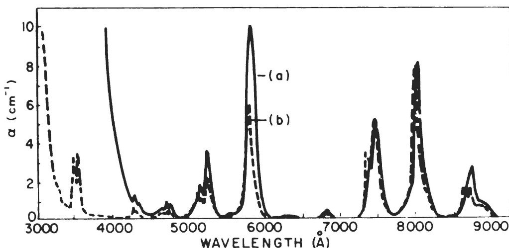
Figure 2 — Absorption spectrum of \text{Nd}^{+3} in: (a) \text{SeOCl}_2 and (b) \text{POCl}_3
