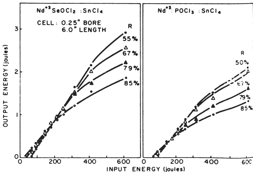
Figure 6 — Output energy as a function of output energy for various output mirror reflectivities R
