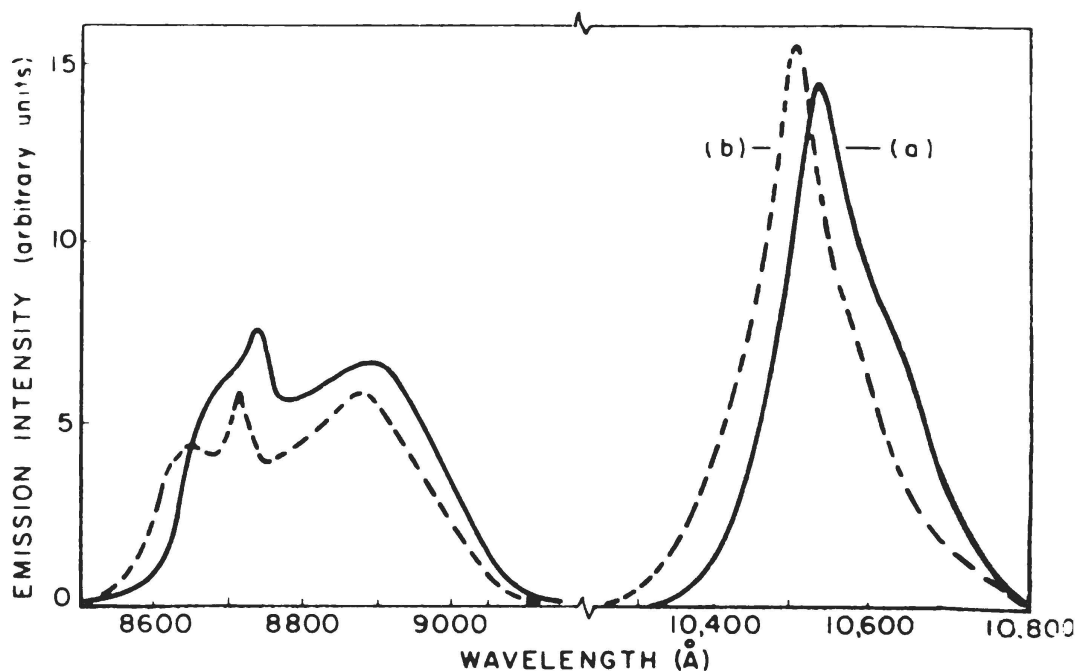
Figure 1 - Fluorescence spectrum of \text{Nd}^{3+} in: (a) \text{SeOCl}_2 and (b) \text{POCl}_3
