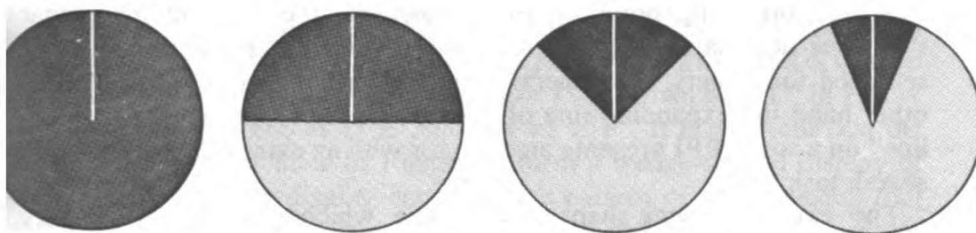
Figure 11 — A conventional PPI and three Continuous Sector Scan displays, of 180°, 90°, and 45° respectively.
