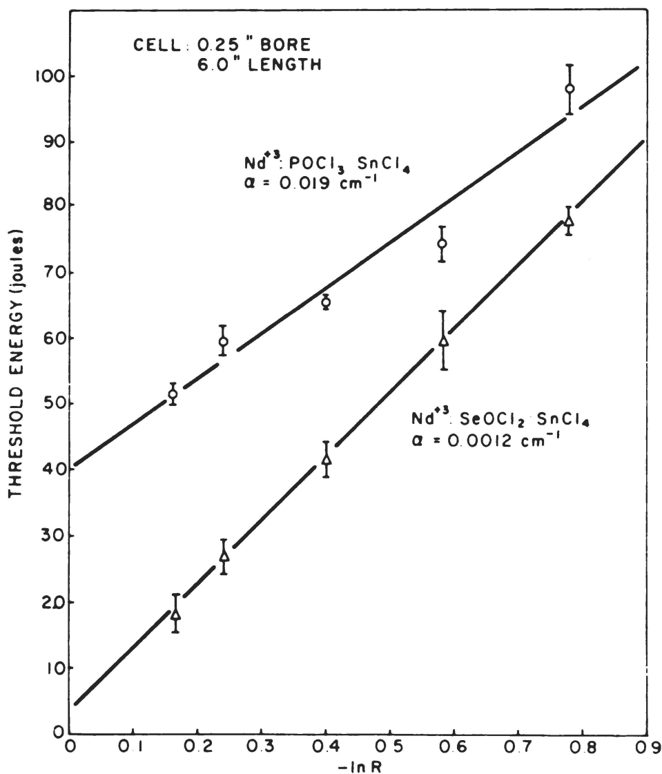
Figure 7 — Threshold energy as a function of output mirror reflectivity. The values of \alpha are the dynamic loss coefficients obtained from these data.
