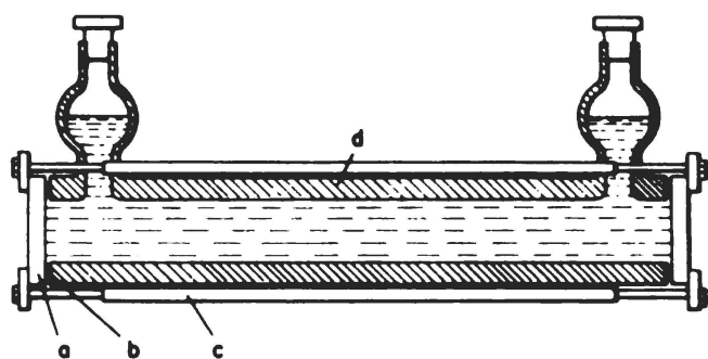
Figure 5 — Demountable liquid laser cell.
