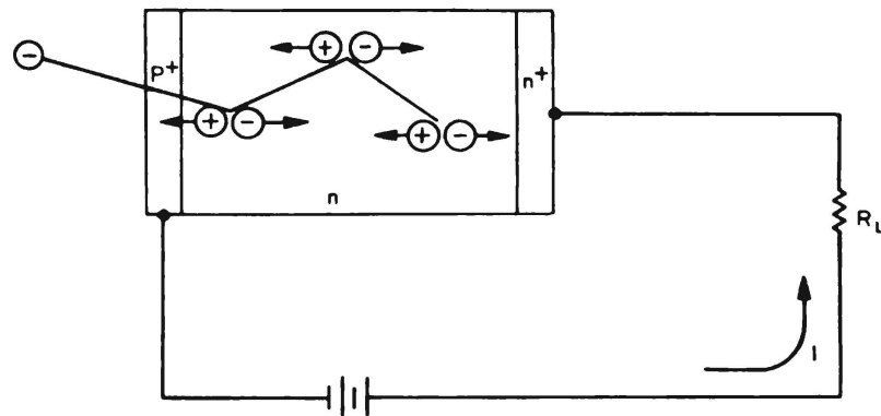
Figure 4 – Electron-hole pair creation
