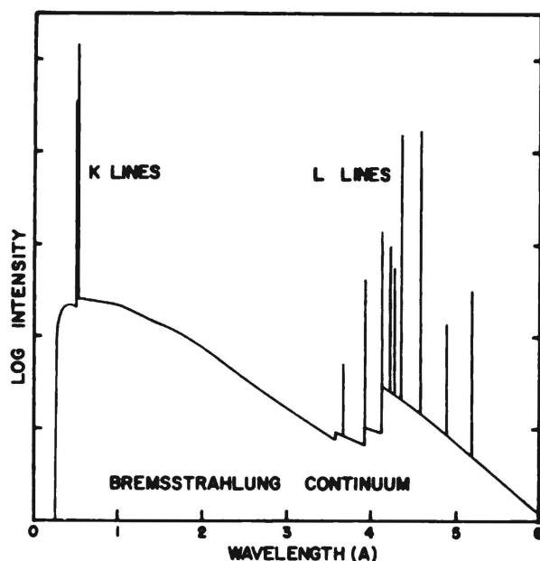
Figure 3 — X-ray spectrum from a rhodium target x-ray tube operated at 45 keV (1)
