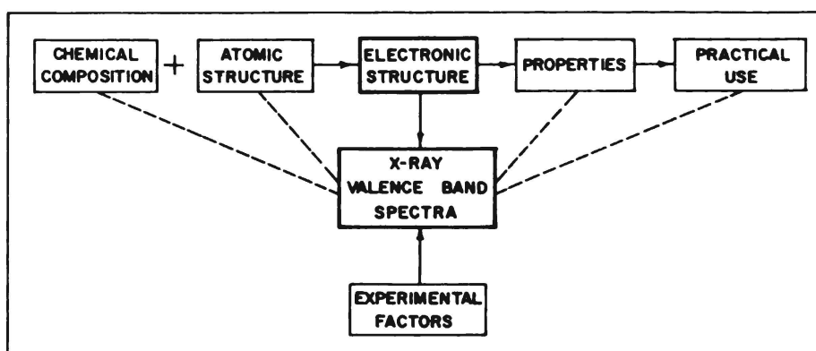
Figure 16 — Relation of material characteristics (top row) to the factors important in the generation and measurement of valence band x-ray spectra (center column). Observed correlations between x-ray spectra and material characteristics are indicated by dashed lines.
