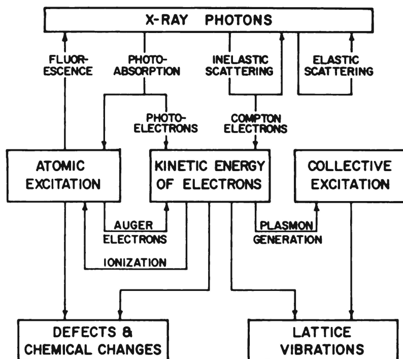
Figure 5 — Flow diagram for the conversion of x-ray photon energy first to electronic excitations and then to defects, chemical changes, and lattice vibrations
