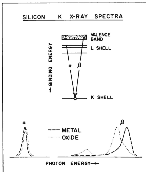
Figure 13 — Energy levels, electron transitions and normalized Si x-ray spectra from pure Si and SiO 2 . The K \beta valence band spectrum is strongly dependent on the bonding of the Si atoms.
