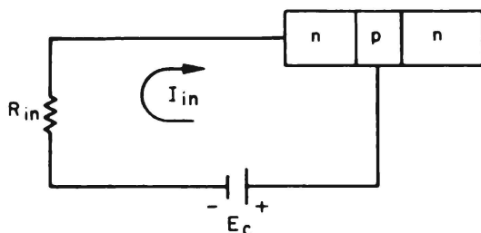
Figure 10 – Forward biased emitter-base junction
