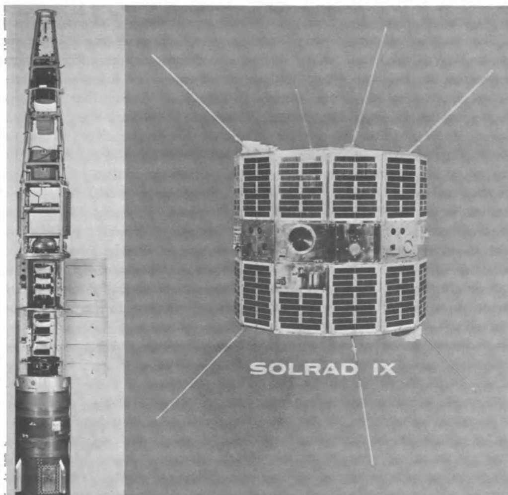
Figure 20 — Aerobee rocket payload (15 in. diameter) and SolRad 9 satellite (30 in. diameter) used for measurement of cosmic x-ray sources
