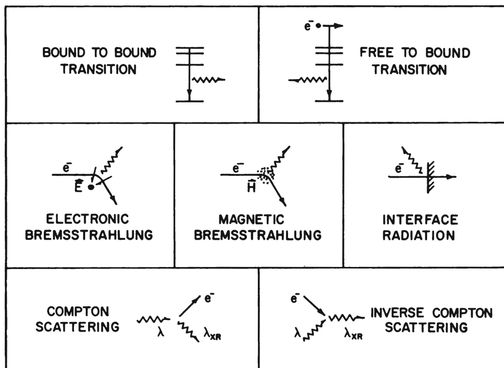
Figure 2 — X-ray generation processes: photon creation by electron transitions to bound states (top row) and between free states (center row), and photon conversion during inelastic scattering (bottom row).
