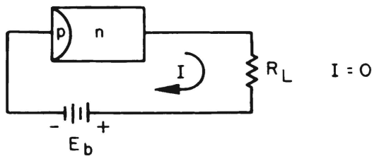
Figure 1 – Reversed biased diode
