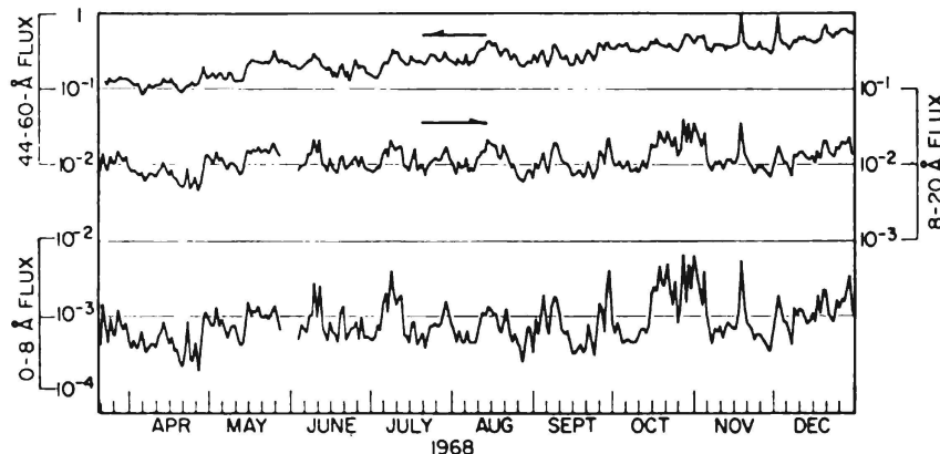
Figure 25 — Intensity variation in three x-ray bands measured during the first months of the SolRad 9 satellite operation. Intensity is given in \text{ergs/cm}^2/\text{sec} (47).
