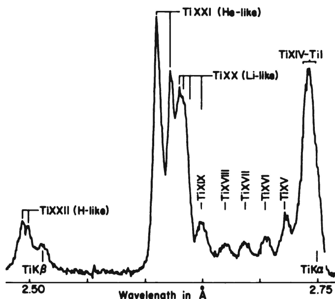
Figure 19 — Densitometer tracing of the time integrated x-ray spectrum from the plasma formed during a vacuum discharge with a Ti anode. Radiation is observed from several highly ionized states, including Ti stripped of 21 of its 22 electrons (41).
