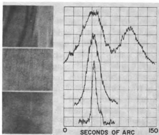
Figure 12 — X-ray topographs and diffraction profiles from synthetic ruby laser crystals of varying structural perfection. Better crystals give featureless topographs and narrow profiles (16).
