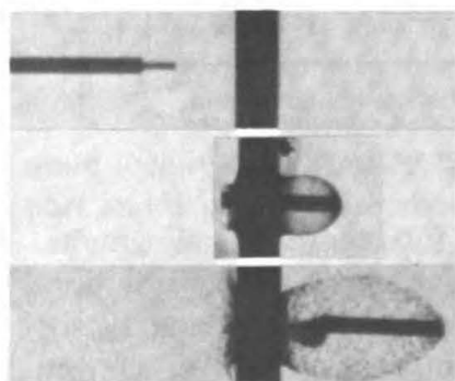
Figure 8 — Sequential flash x-ray photographs of a steel rod moving at 15,000 ft sec and penetrating a 1/4 in. steel plate (edgeview)
