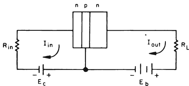
Figure 11 – Transistor circuit
