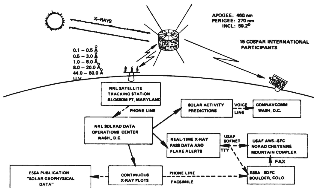
Figure 26 – The SolRad 9 solar x-ray monitoring and disturbance warning system
