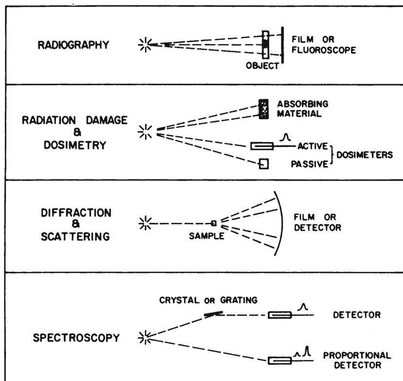
Figure 6 — Schematics of the x-ray source and equipment used for measurements in each of the major x-ray areas
