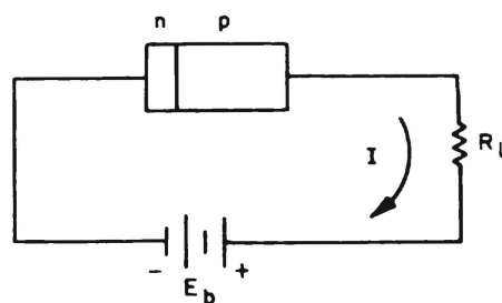
Figure 7 — Equivalent, forward biased diode
