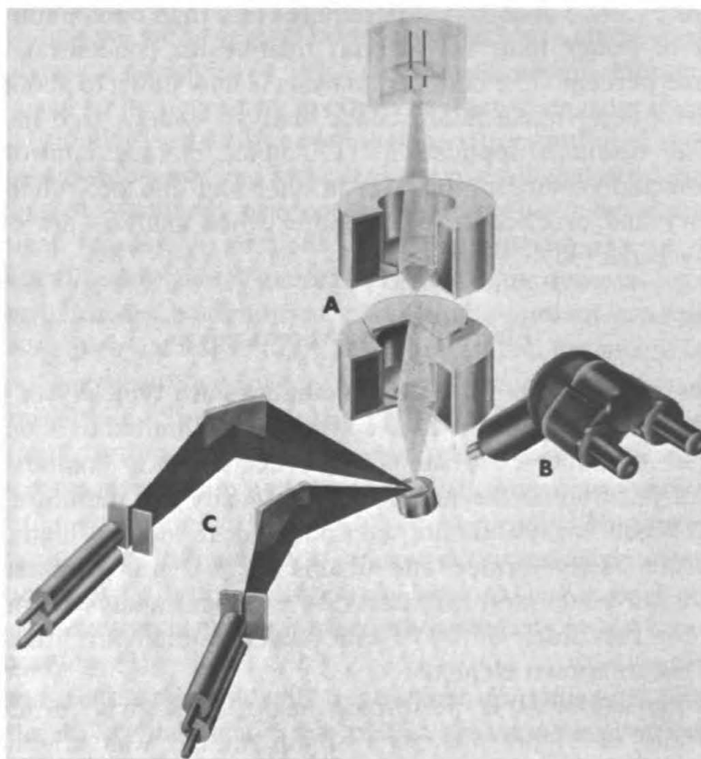
Figure 14 — Schematic of the electron probe micro-analyzer (35). The electron optics (a) produce a beam to excite x-rays from a one micron diameter spot on the specimen chosen by use of the light optics (b). Measurements with the x-ray optics (c) yield the quantitative chemical analysis.
