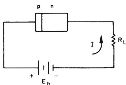
Figure 6 — Forward biased diode
