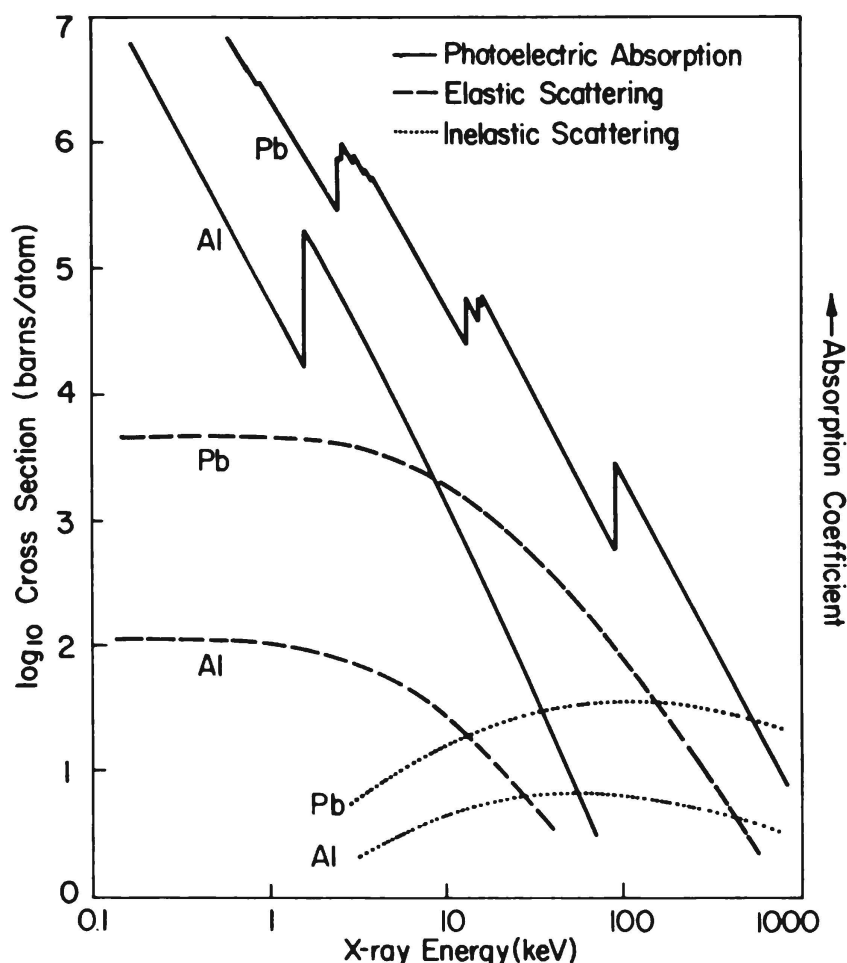
Figure 4 – Cross sections for the interaction of x-ray photons with Al and Pb
