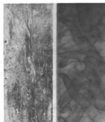
Figure 7 — Photograph (left) and x-radiograph (right) of a piece of apparently sound wood which has been hollowed out by Teredo marine borers
