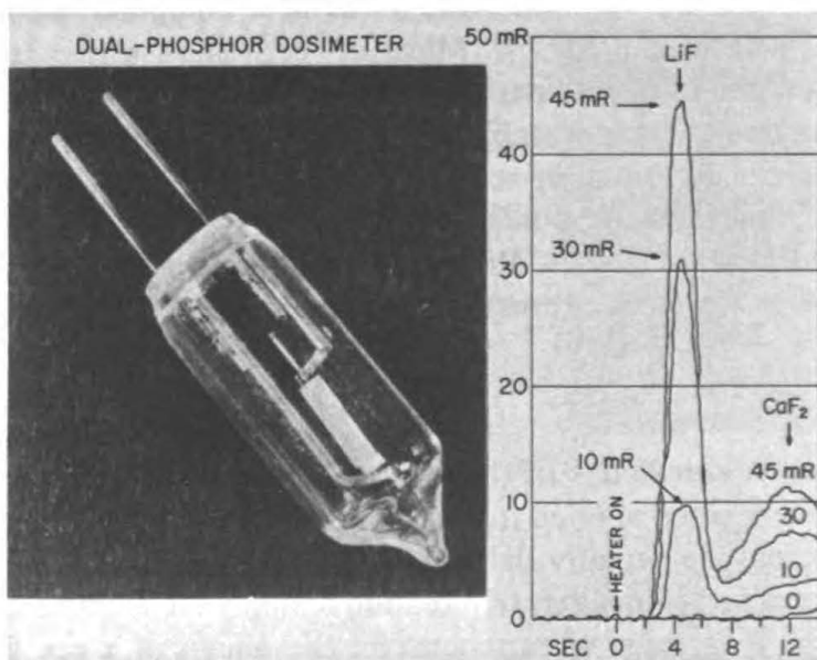
Figure 9 — Glow curves (right) obtained from a bulb-type dosimeter containing LiF and CaF 2 (left) (5). Exposure levels are given in milliroentgens.
