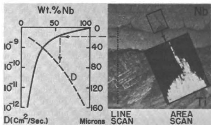
Figure 15 — Titanium-niobium interdiffusion couple measured with the electron probe x-ray microanalyzer. Left: Measured concentration profile and calculated interdiffusion coefficient. Right: Photomicrograph of the diffusion zone plus a composition map of Ti in a grain boundary diffusion feature.
