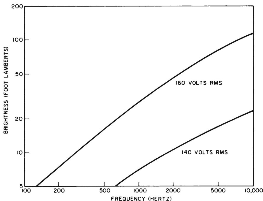
Figure 10 — Typical brightness and frequency characteristic for LEF driven at constant voltage. High contrast numeric element, 0.40 inch high
