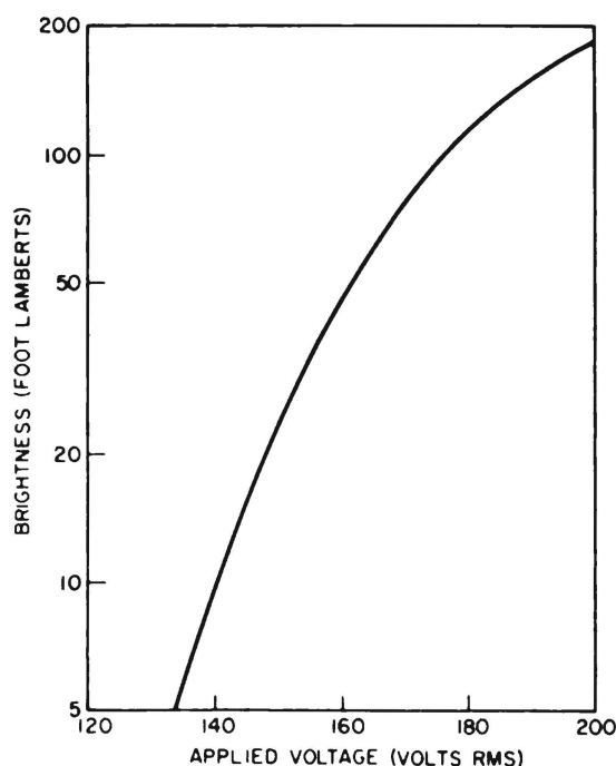
Figure 9 — Typical brightness and voltage characteristic for LEF driven at constant frequency (2.5 KHz). High contrast numeric element, 0.40 inch high.
