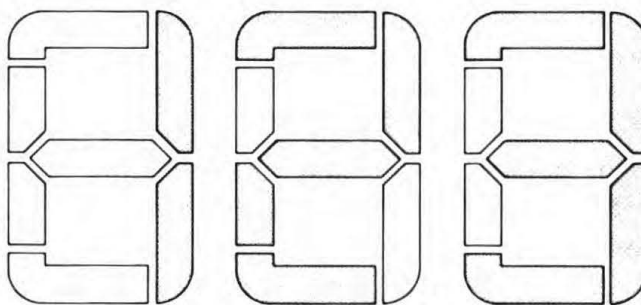
Figure 4 — Typical configuration for a seven-segment numeric, showing the numbers 1, 2, and 3
