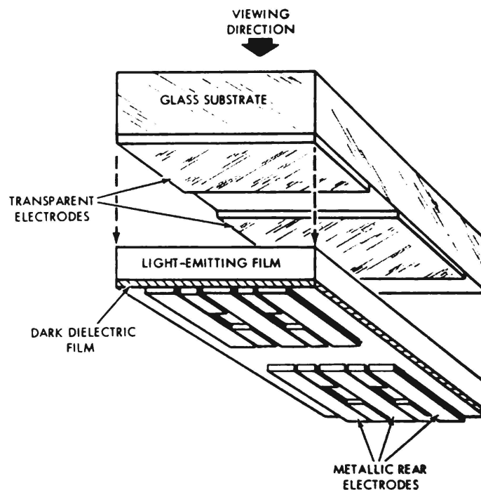
Figure 3 — Typical LEF structure
