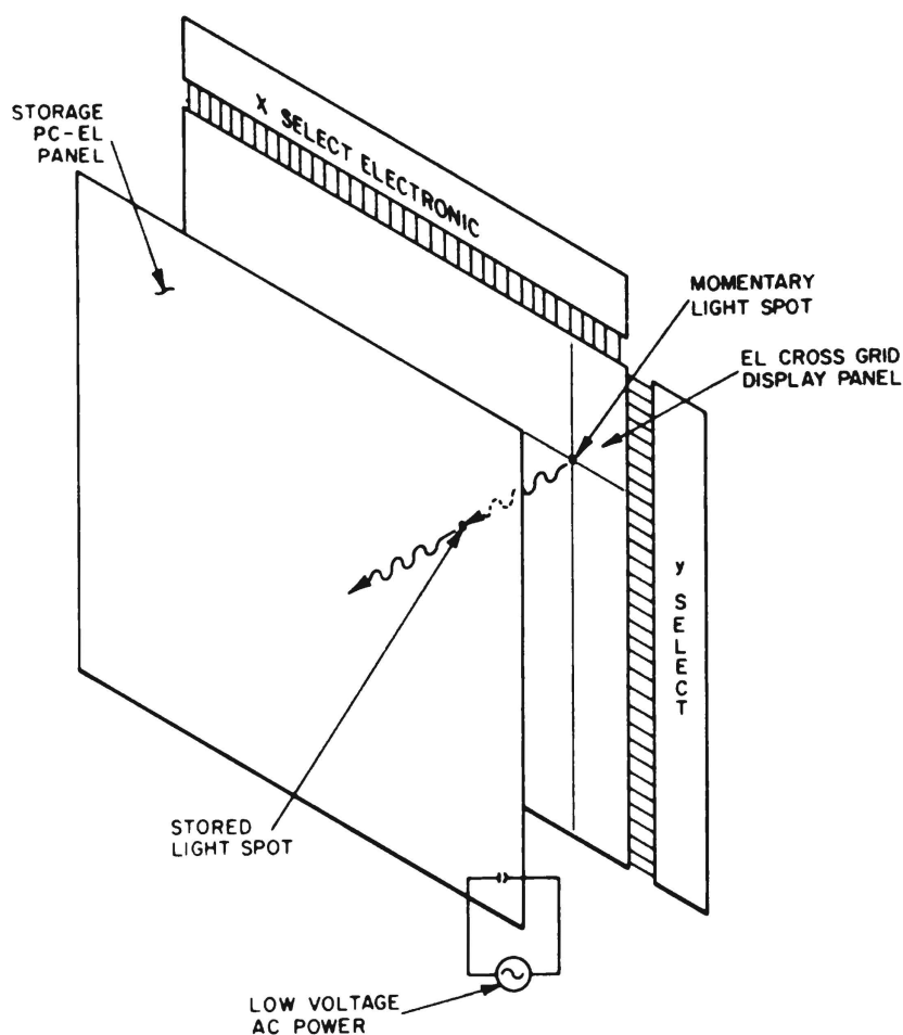
Figure 6 — Functional EL storage display
