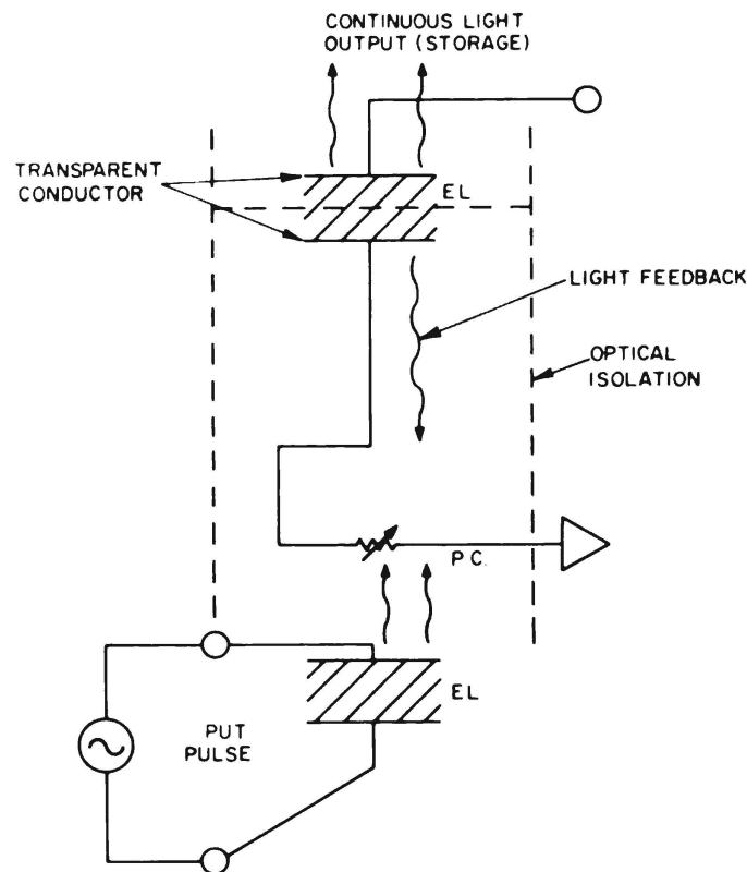
Figure 2 – Electro-optic circuit for EL storage panel
