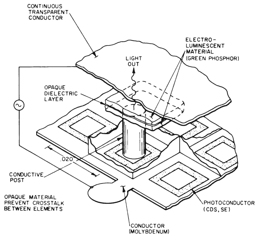
Figure 5 — Simple 3D geometry of PC-EL storage display section
