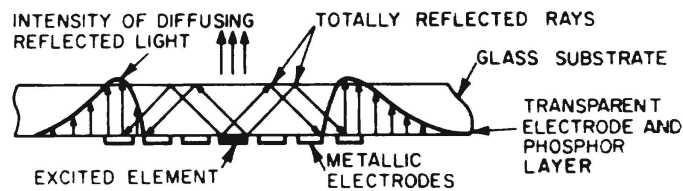
Figure 2 — Halo effect in LEF panel, caused by total internal reflection at the glass/air interface at and beyond the critical angle. This effect can be sharply reduced by use of transparent phosphors and a backing layer with low diffuse reflectivity.
