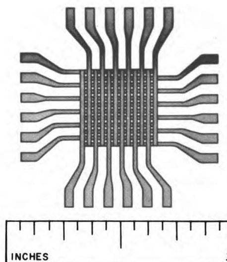
Figure 7 — Crossed electrode configuration of small LEF test panel
