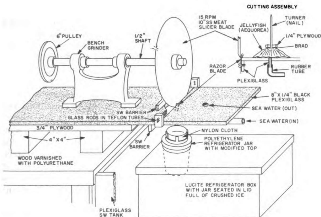
Figure 4 — Machine used in “de-ringing” specimens of Aequorea, by first positioning them over inflowing sea water, which also inflates the body somewhat by filling the internal canals, then, with the aid of a “turner,” rotating the specimen against a razor blade juxtaposed against a slowly moving meat-slicer blade. The black plexiglass platform aided visibility of the internal organs, though careful observation during the cutting process was usually not necessary because the teflon-covered horizontal glass rods (held at the positions indicated but not fully shown in the figure) prevented more than a narrow edge of the specimen from reaching the blades. The platform was slightly tilted so that sea water drained towards the opening just beyond the cutting edges. The excised rings were thus washed gently into a receptacle which was kept immersed in crushed ice. The overflow from the receptacle drained through a nylon cloth collar which prevented the escape of the rings.
