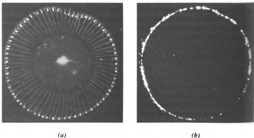
Figure 1 — (a) A single specimen of Aequorea photographed by daylight in its natural sea water habitat, as viewed from the aboral surface. The mouth is indicated by the central, whitish mass, visible through the nearly transparent body, on the under side. The passage from the mouth leads to the radial canals and thence to the marginal canal at the periphery. The tentacles are shown in a contracted state as conspicuous white dots along the marginal canal, with the much smaller photogenic organs difficult to discern between the bases of the tentacles. (b) A similar specimen, photographed by its own light in otherwise complete darkness.
