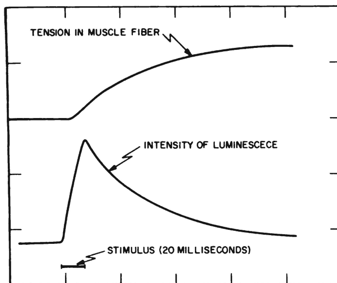
Figure 3 — Slightly smoothed curves from the data of Ridgway and Ashley (1967), the first published example of the use of aequorin as a test from calcium in a living system. A single muscle fiber of the barnacle Balanus nubilus was micro-injected with partially purified aequorin which was allowed to diffuse through the fiber, causing no harm. Light emission of aequorin followed very closely after the onset of electrical stimulation, i.e., after a delay of about a thousandth of a second, and the development of tension after about 5 thousandths of a second. Following the initial excitation, tension in the fiber continued to increase after the cessation of the electrical pulse, at which time the light began to decrease. These data are averaged (by inspection) from five repeated experiments giving quantitatively close to the same results.
