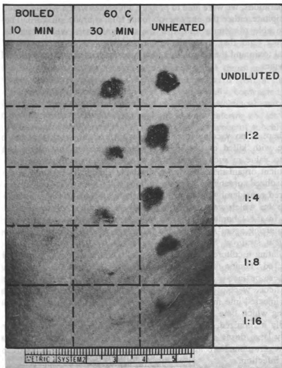
Figure 6 — Lesions in a guinea pig produced by intradermal inoculations of sterile filtrate from a 10-day-old broth culture of Pseudomonas pseudomallei , strain 111-9. The photograph was taken 4 hours after inoculation. From reference number 3.
