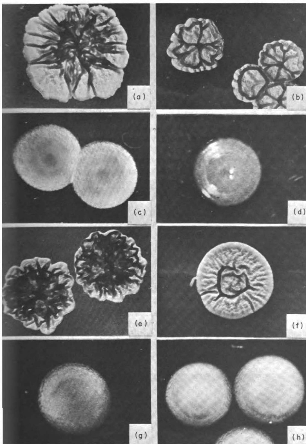
Figure 2 — Representative rough and smooth variants isolated from stock cultures of Pseudomonas pseudomallei . All strains were virulent since less than 100 cells were lethal for hamsters. All photographs at approximately 5.5X. (a) From strain 101. Rough yellow lacy type. (b) From strain 101. Rough white type. (c) From strain 101. Smooth white type. (d) From strain 104-2. Smooth yellow type. (e) From strain 102. Rough orange type. (f) From strain 102. Rough cream type. (g) From strain 103. Smooth cream type. (h) From strain 114. Smooth white type. (From reference number 2.)
