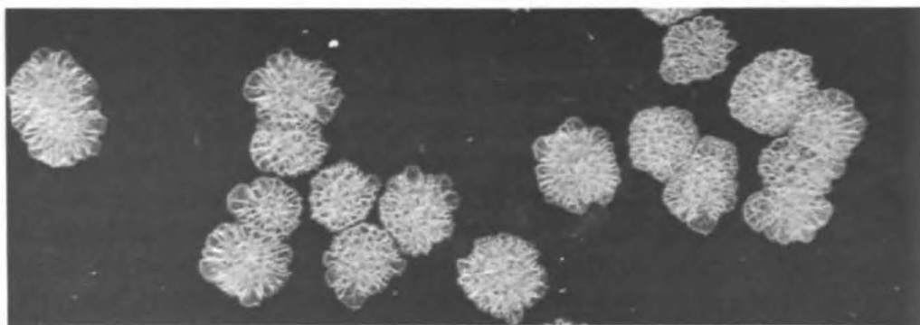
Figure 3 — Strain 103R before adaptation to mice. Large lacy rough yellow colonies.
