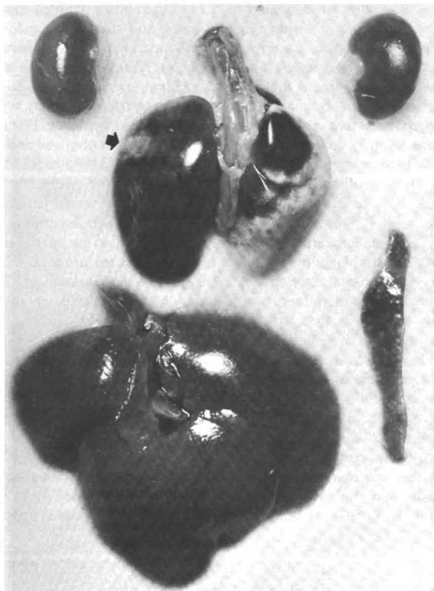
Figure 1 — Organs of hamster moribund 3 days after inhalation of approximately 46 organisms. Three lesions were present in the lungs, one of which is shown at the periphery of the left lung (arrow). There is hemorrhagic pulmonary consolidation of the entire left lung and of portions of the right lung. The spleen shows many small lesions. The liver and kidneys appear normal. From reference number 1.
