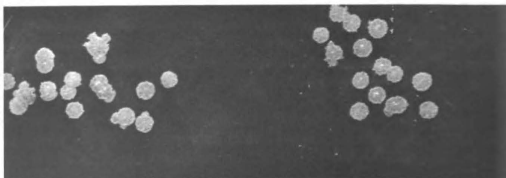
Figure 4 — Strain 103R after adaptation to mice, showing pure culture of small intermediate rough yellow colonies
