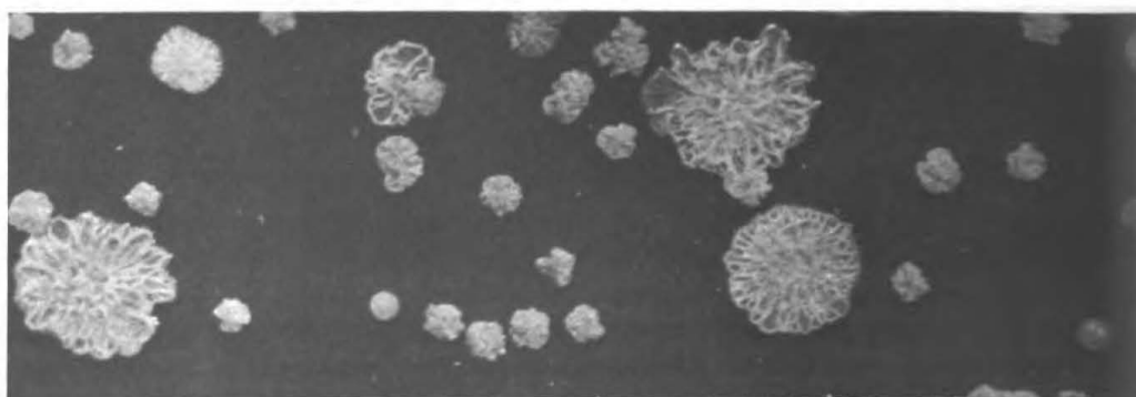
Figure 5 — Strain 103R, showing reversion to the parent type (in Figure 3) of the small intermediate rough yellow colony (in Figure 4) after several passages on agar. From reference number 2.
