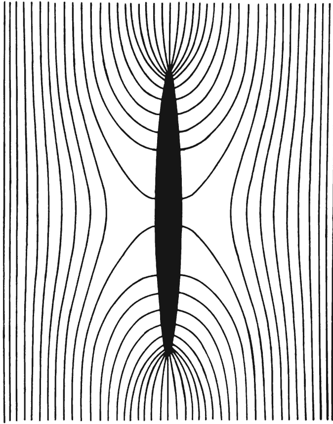
Figure 2 — Uniform electric field distorted by a conducting ellipsoid
