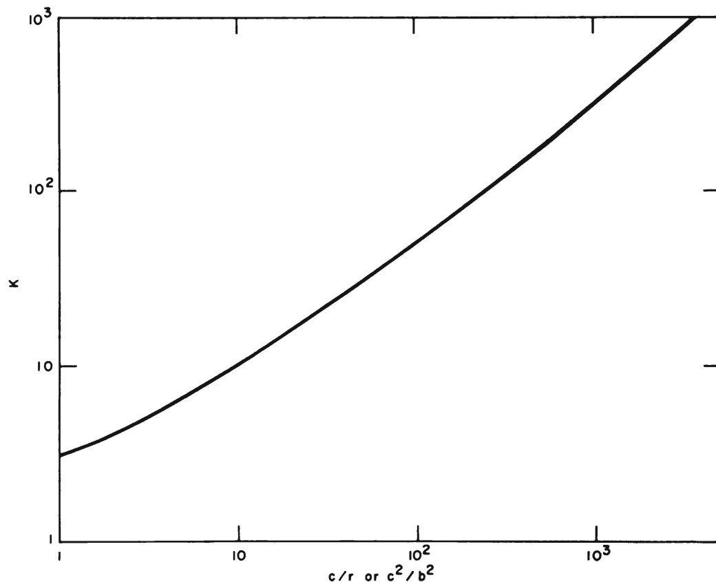
Figure 3 — The electric field enhancement factor "K" at the top of a vertical, prolate ellipsoid versus the ratio of the height of the half ellipsoid c to the radius of curvature of the tip, r
