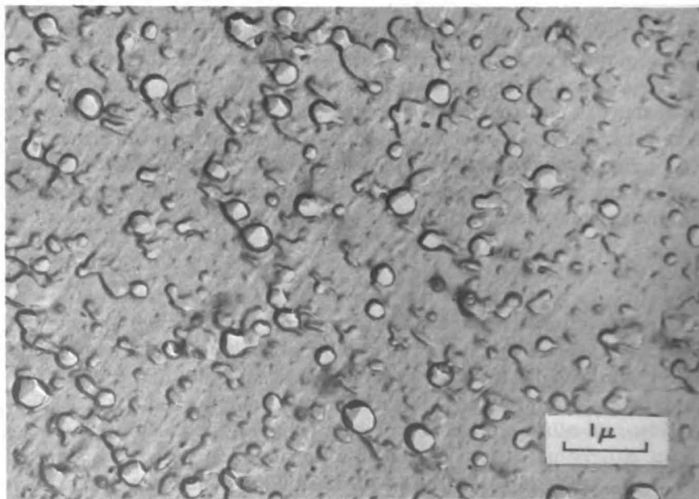
Figure 2b — Iron containing fine iron carbide particles can be considered as an example of a “particulate” composite. Magnification 15,000X.
