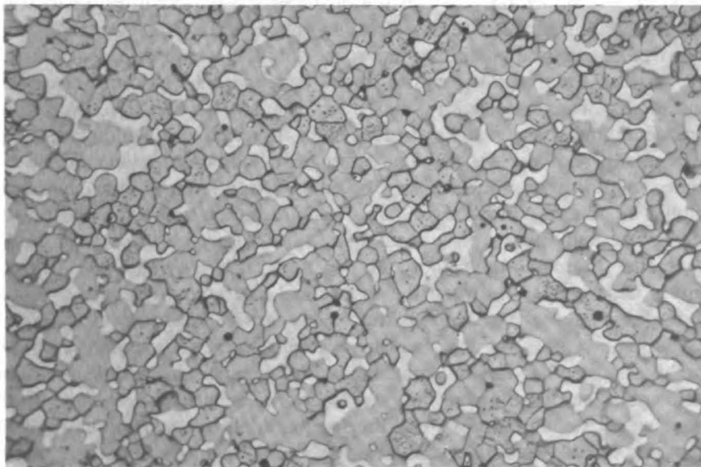
Figure 1 — Photomicrograph of silver infiltrated tungsten showing occasional uninfiltrated pores (small dark areas) in tungsten matrix. The light regions are silver and the gray regions are tungsten. Magnification is 500X. Murakami's etching reagent used.
