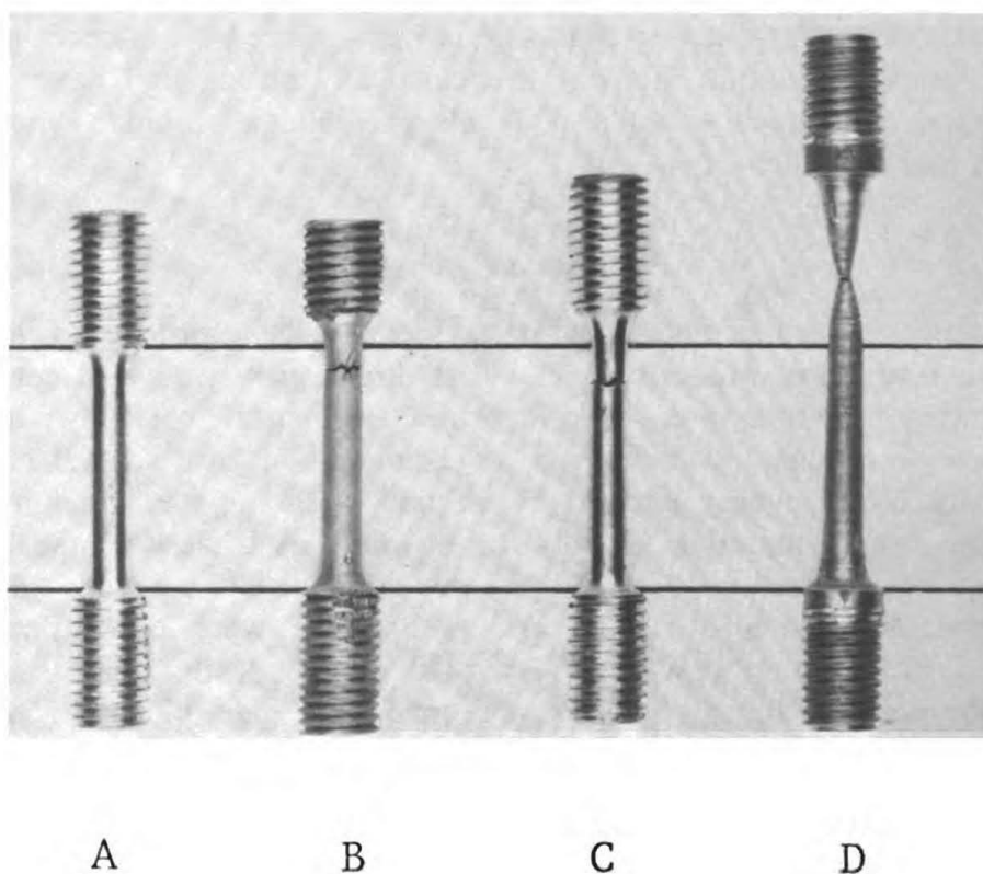
Figure 4 — Tensile bars of zinc containing various amounts of tungsten particles deformed at room temperature to failure. A and B depict undeformed and deformed pure zinc. C depicts zinc containing 5 volume percent tungsten particles. D depicts zinc containing 15 volume percent tungsten particles. When a small amount of tungsten particles are added to zinc, no increase in elongation is observed over that for pure zinc (compare C with B). When a large amount of tungsten particles are added, fifteen volume percent, the particulate composite becomes very ductile (specimen D).
