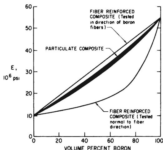
Figure 3 — Predicted elastic behavior of aluminum-boron alloys when in the form of "fiber" composites and "particulate" composites
