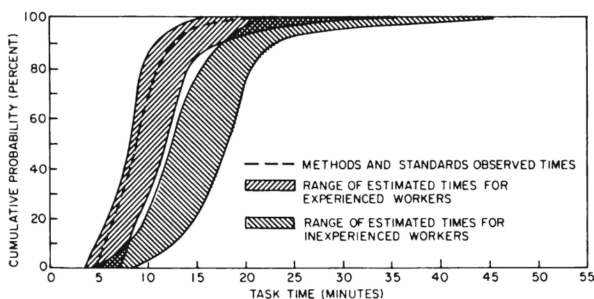
Figure 3 – Observed and estimated times for replacing and securing manhole covers, Long Beach Naval Shipyard
