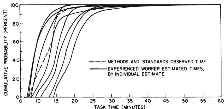
Figure 2 — Observed and estimated times for silver braising four-inch copper-nickel pipe, experienced workers Long Beach Naval Shipyard
