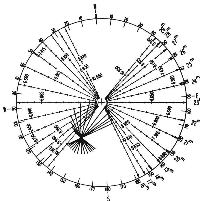
Figure 3 — Fix determined on intercept chart
