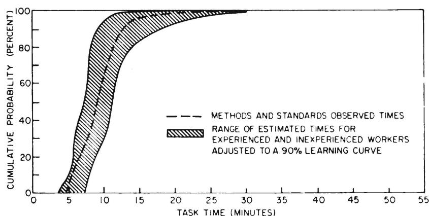
Figure 4 – Observed and adjusted estimated times for replacing and securing manhole covers, Long Beach Naval Shipyard
