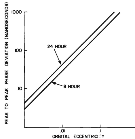
Figure 12 — Error in satellite clocks due to relativistic effects on eccentric orbits
