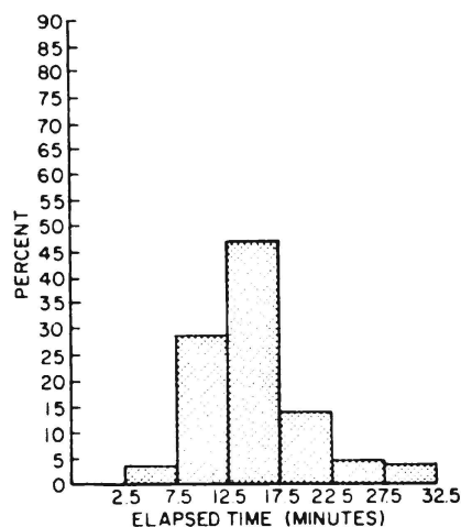
Figure 1 — Estimated times for silver braising four-inch copper-nickel pipe, subject No. 16 Long Beach Naval Shipyard
