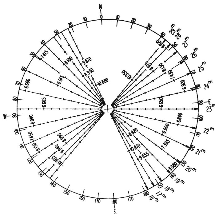
Figure 2 — Precomputed intercept chart
