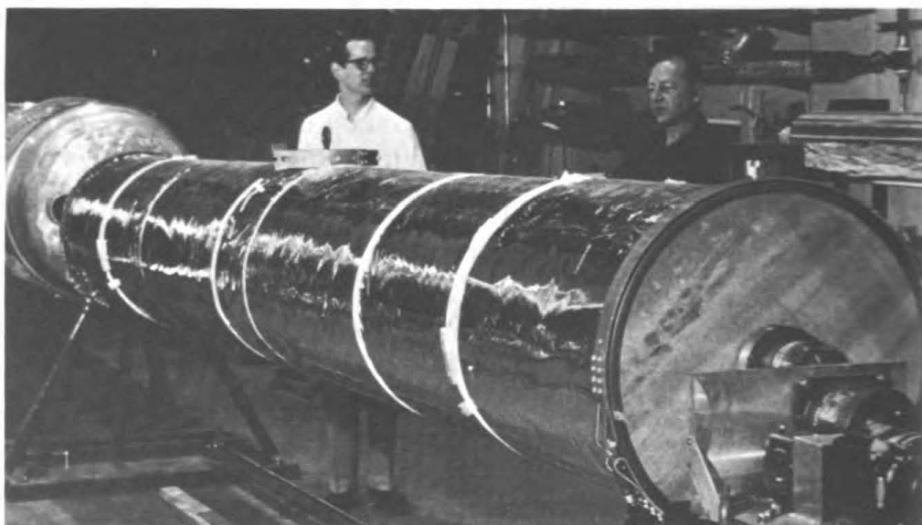
Figure 4 — Prototype 20-foot dewar module during assembly
