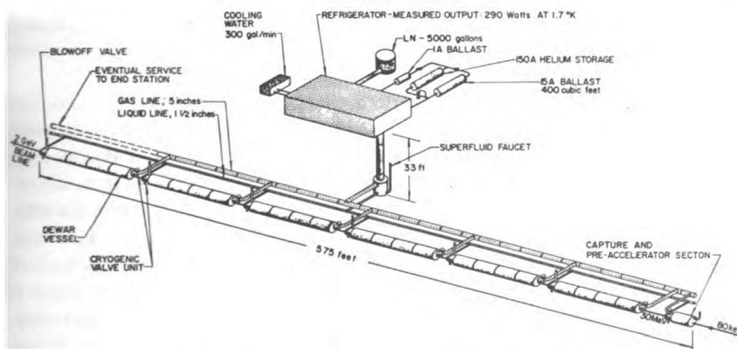
Figure 2 — Block diagram of cryogenic system
