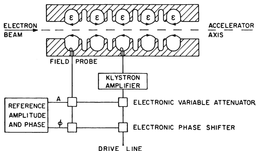
Figure 1 — Bi-periodic \pi/2 -mode accelerator structure with electronic feedback stabilization
