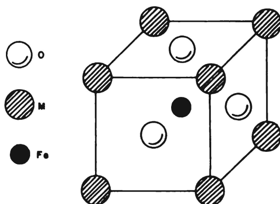
Figure 1 — Crystal structure of perovskite-type magnetic oxides
