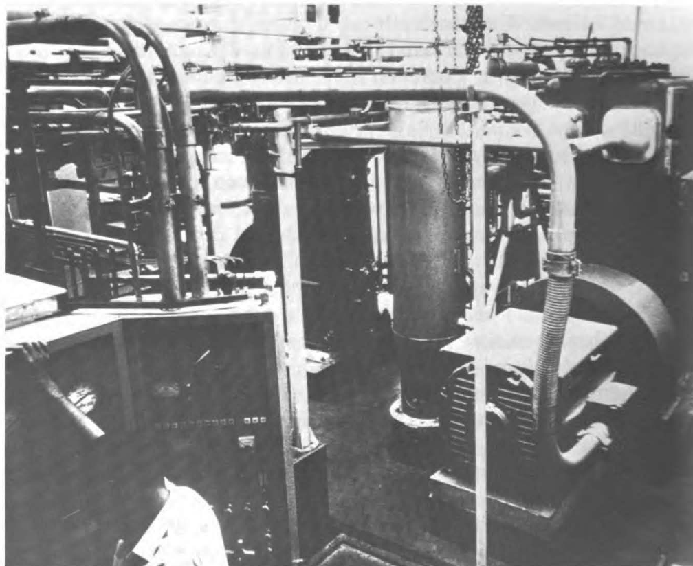
Figure 3 — Refrigeration plant
