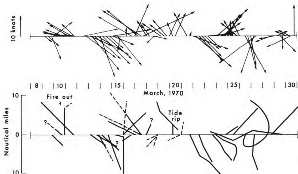
Figure 3 — Wind vectors versus slick vectors
