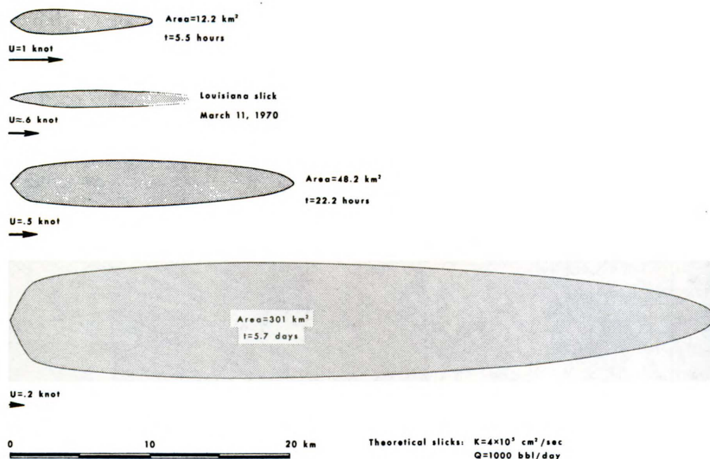
Figure 4 – Comparison of observed slick against theoretical slicks, illustrating effect of decreasing current velocity on slick size
