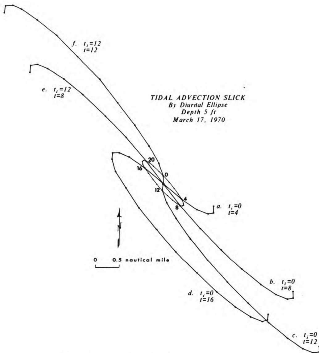
Figure 5 — Traces of oil slick from a continuous source created by diurnal rotary current
