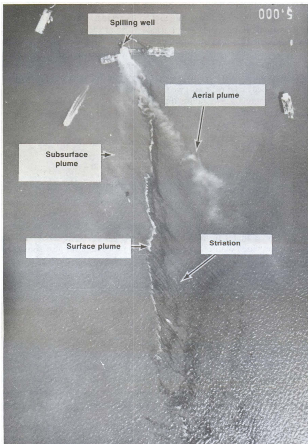
Figure 2 — Aerial, surface, and subsurface plumes moving in different directions from the spilling well. Note striations parallel to the aerial plume, indicating downward elongation. (Photo courtesy of U.S. Geological Survey.)
