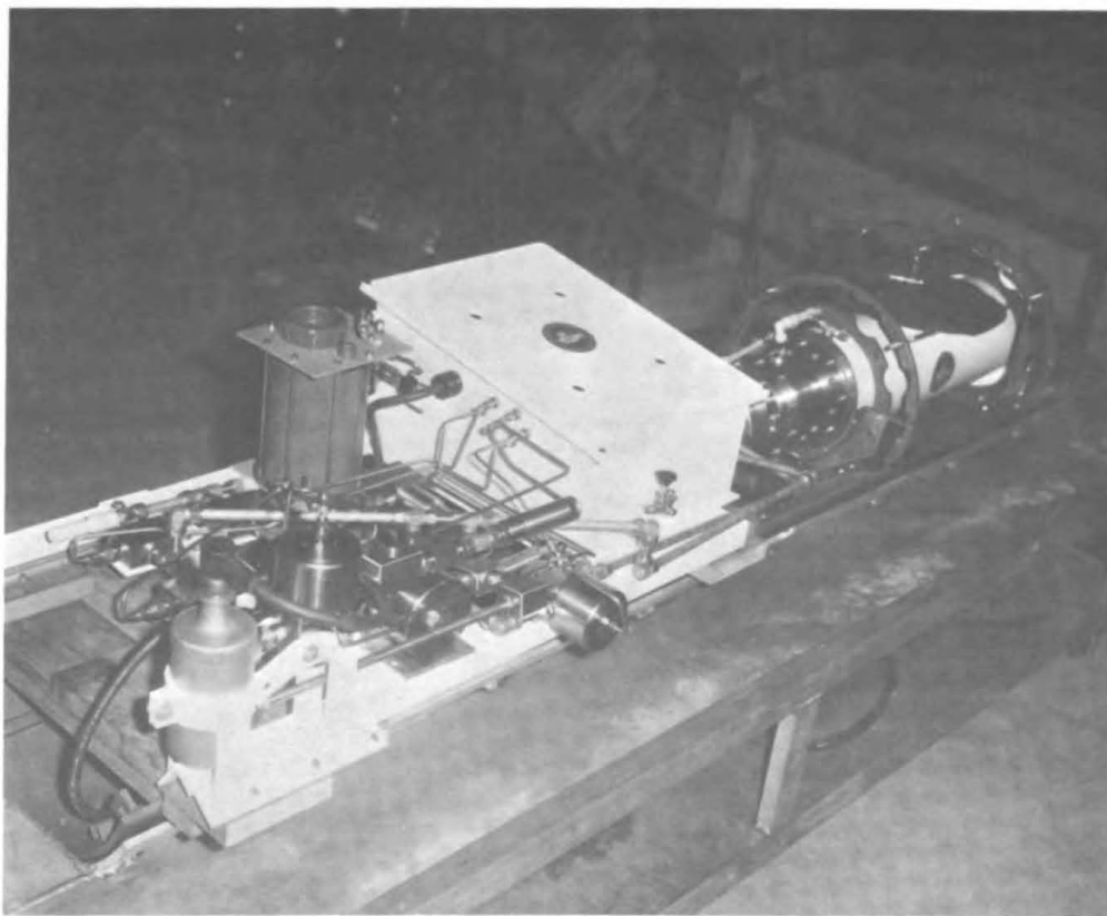
Figure 6 – The Center-developed seawater variable ballast system before installation in the ALVIN. At the left are the seawater control valves. In the center is the pressure-compensated, auxiliary hydraulic control box. To the right is the pressure-compensated seawater pump with its d.c. drive motor and controls.
