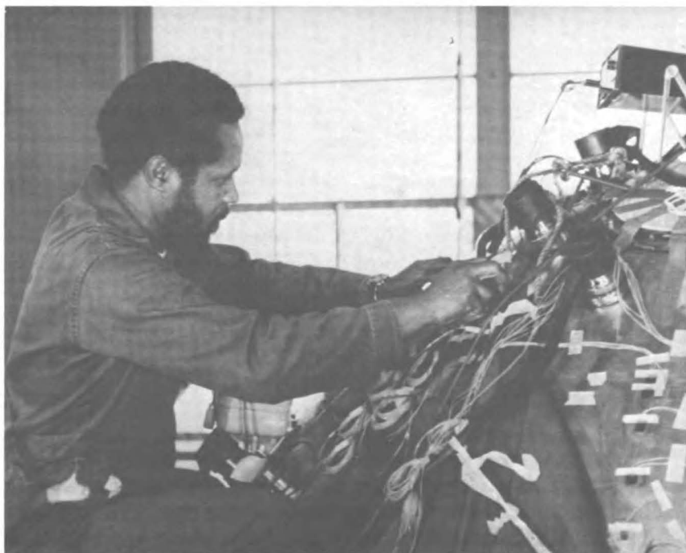
Figure 4 – At Carderock, Structures Department engineers directed the placement of strain gauges on the prototype sphere.
