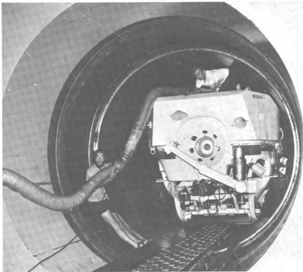
Figure 9 – The ALVIN, positioned in the large pressure tank for the manned test, receives a final air conditioning before the closure plug is inserted.
