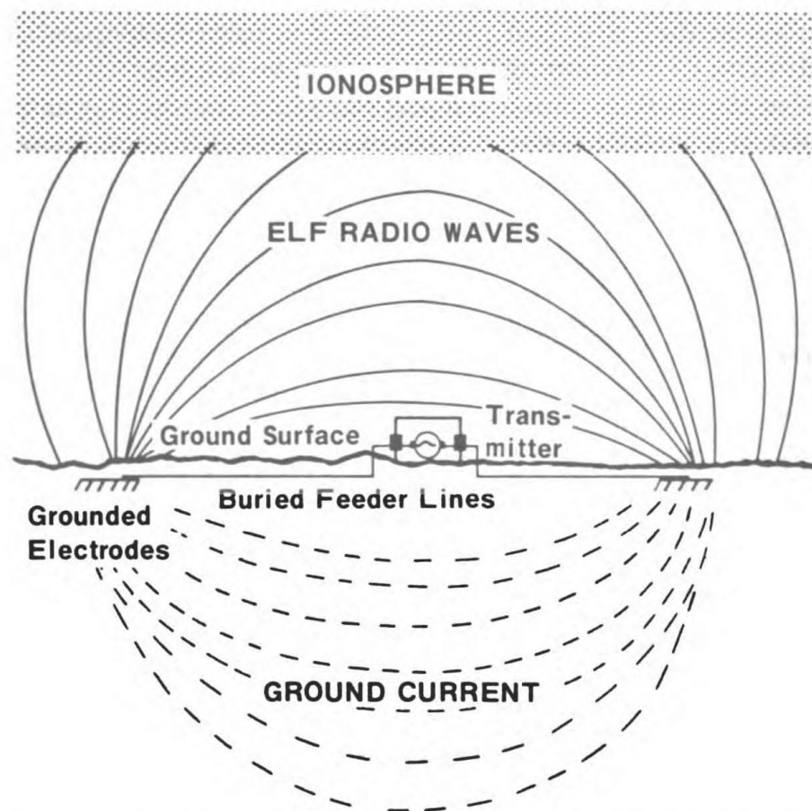
Figure 2 – The Sanguine transmitter will have feeder lines connected to two separated and grounded electrodes in the earth and the energy will flow between them via multiple paths within the earth.
