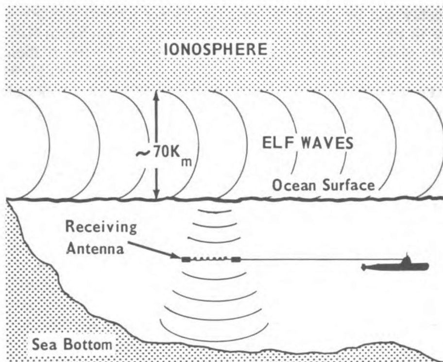
Figure 1 – The receiving antenna will probably consist of a type of trailing wire antenna in which both the electric and the magnetic field components are detected.
