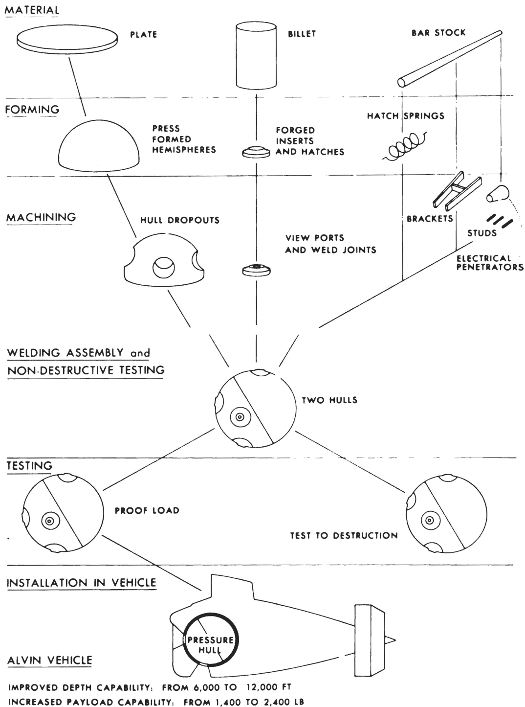
Figure 1 – Steps in fabricating titanium pressure hull for DSRV ALVIN.
