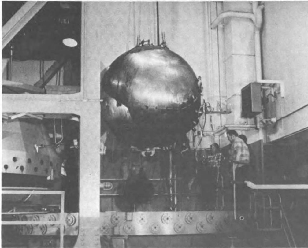
Figure 5 – The hull is lowered into a ten-foot, 10,000 psi spherical pressure chamber and subjected to three pressure runs to verify its structural predictions.
