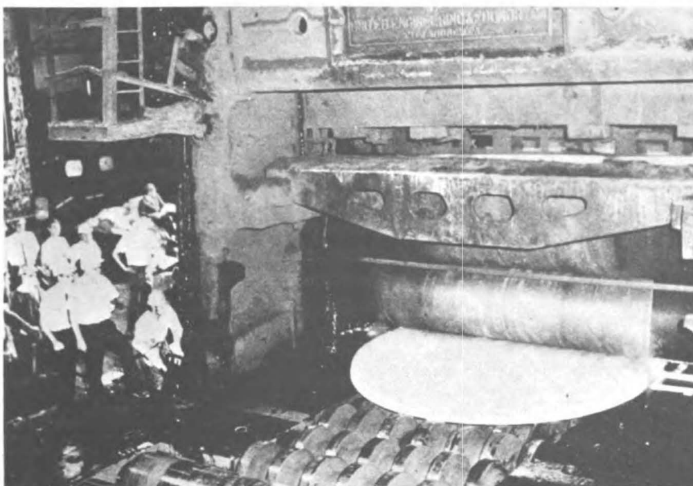
Figure 3 – Circular rolling of Ti 621/0.8 Mo alloy titanium plate.
