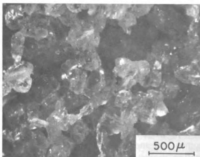
Figure 2 – Photomicrographs of the cutting faces of two types of grinding wheels. The diamond wheel has a “closed” structure in the sense that the abrasive grains protrude from a continuous matrix of binder. The alumina wheel, on the other hand, has an “open” structure with a cutting face that contains a large number of voids.
