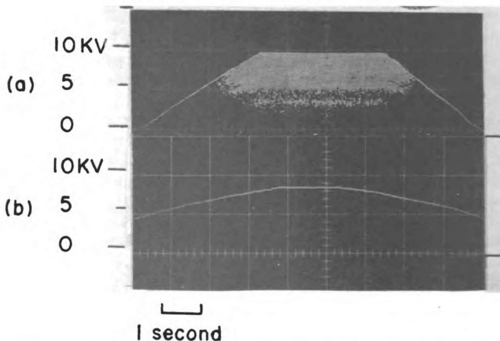
Figure 9 – Effect of surface flaws on the incidence of corona discharge in a PZT sonar transducer ring. CRT display records many positive half cycle voltage traces (60 Hz; a.c.). Image intensity enhancement at voltage maxima gives trace of applied voltage. Image intensity enhancement when charge flow exceeds 5 picocoulombs indicates when corona discharge takes place. (See R. G. Johnson and S. J. Tibbetts, Rev. Sci. Inst. 44 , 519 (1973)).
