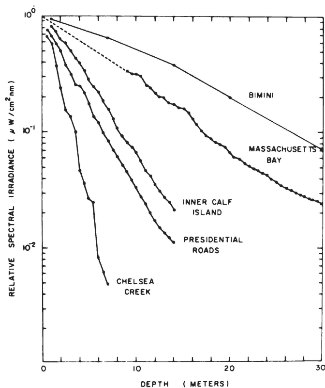
Figure 8 - Irradiance vs depth at 560 nm for 3 locations in Boston Harbor (Aug. 12-24).
