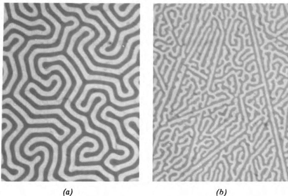
Figure 7 – Effect of substrate surface preparation on magnetic domain configuration in an epitaxial garnet layer. In (a) the domain boundaries are clearly held up along residual scratches. In (b) the substrate is carefully lapped, polished and stress relieved to produce equilibrium domain configuration. Magnification 160X. (Courtesy T. S. Liu and R. B. Fryer, Honeywell Corporate Research Center.)
