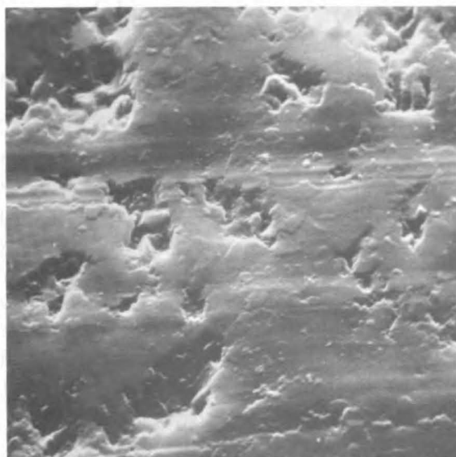
Figure 6 – Scanning electron micrograph of hot pressed polycrystalline alumina ground with a 100 grit diamond wheel. In a ceramic with high impact resistance, material removal occurs mainly by plastic flow. Grinding direction horizontal. Magnification 2000X.
