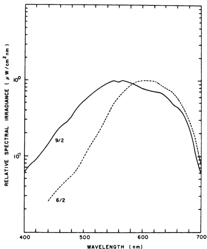
Figure 7 – Comparisons of spectral distribution on two days three months apart. Both sets of data were taken at the same location in Boston Inner Harbor at a depth of 3 m.
