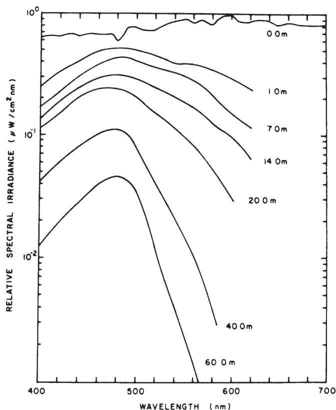
Figure 3 – Relative spectral irradiance for a series of depths in the Gulf Stream 5 miles west of Bimini, Bahamas.
