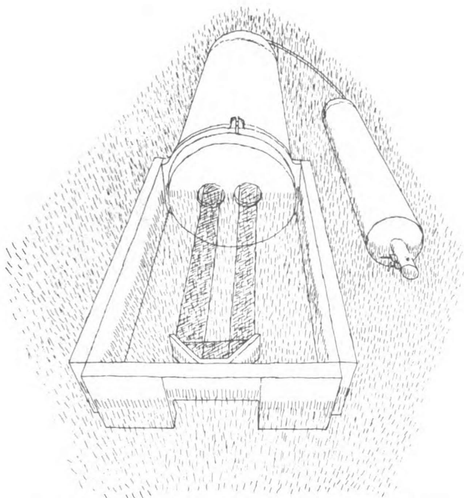
Figure 2 – The optical instrument and the CTD simultaneously measure an undisturbed microstructure feature, here a salt finger interface. The 5 cm diameter laser beam traverses 160 cm of seawater. Refraction by optical inhomogeneities along the path produces a shadowgraph which is photographed within the housing. The CTD measures salinity to .001 ‰, temperature to .0005°C, and depth to 5 cm.
