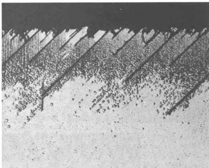
Figure 3 - \{100\} cross section through a magnesium oxide crystal ground with a 100 grit diamond wheel. The machined surface (top) was \{110\} . Grinding has introduced a large number of subsurface \{100\} cleavage cracks. The cracks extend to the bottom of a highly deformed layer as revealed by dislocation etch pits. Magnification 250X.
