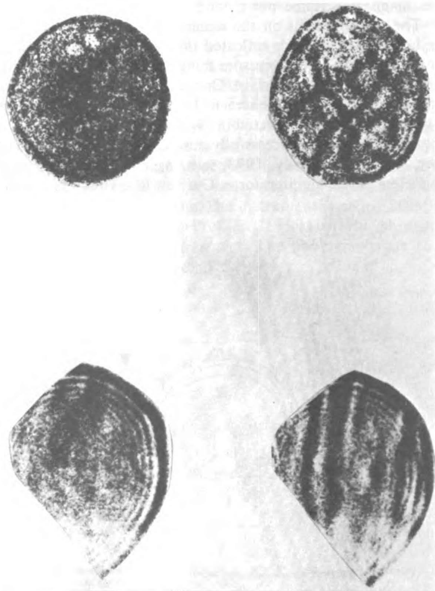
Figure 3 – Shadowgraphs taken by SCIMP show turbulent structure at the upper right contrasted to nearby homogeneous water at the upper left. Salt fingers are indicated by the vertical bands in the image at the lower right contrasted to the image 25 cm shallower without bands at the lower left. The images are 5 cm in diameter.
