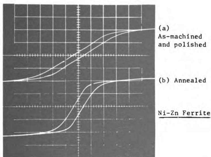
Figure 8 – Effect of surface condition on the B-H loop of a Ni-Zn ferrite toroid showing degradation of magnetic properties resulting from ceramic machining (Courtesy J. R. Kench, Honeywell Corporate Research Center.)
