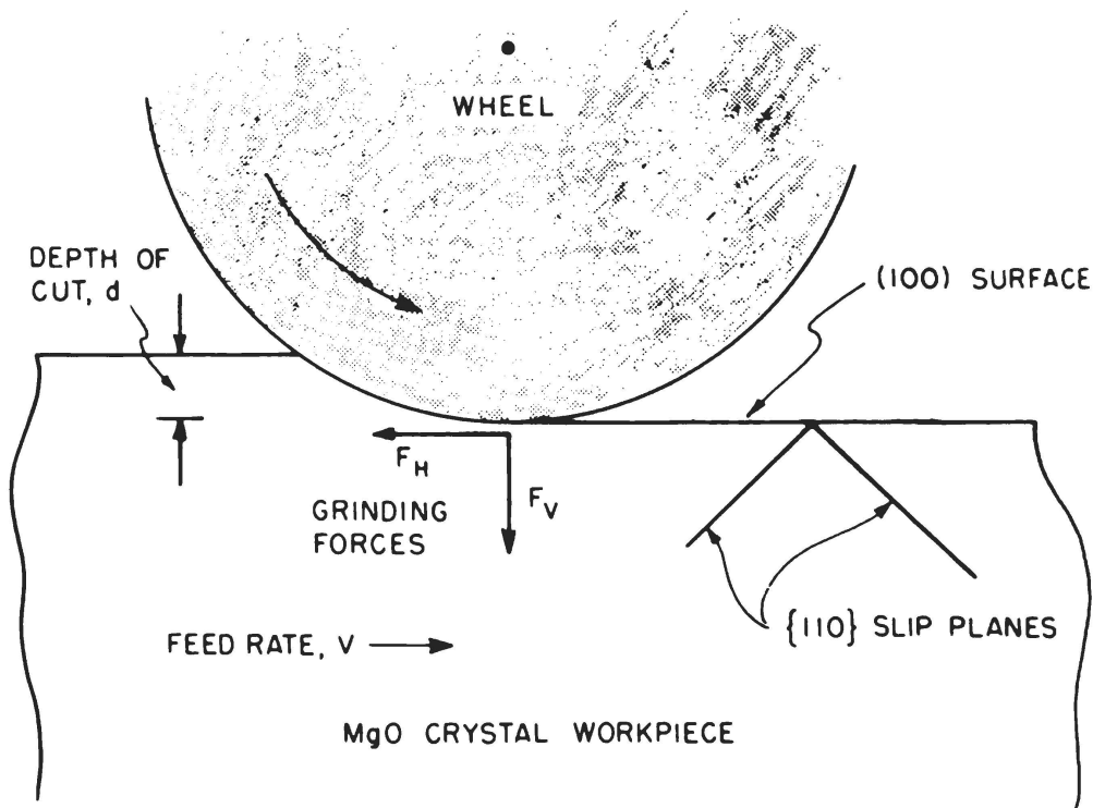
Figure 1 – Schematic showing the wheel-workpiece geometry during a climb-grinding pass on a magnesium oxide crystal workpiece. The cutting face of the wheel moves in the same direction as the workpiece. In the orientation shown, the workpiece is least liable to fracture since slip on {110} planes at 45^\circ to F_V relieves the grinding stresses.
