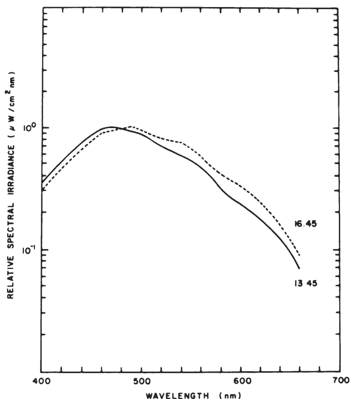
Figure 4 – Variation in spectral distribution of irradiance from 13:45 EST to 16:45 EST. These data were taken 1.0 m below the surface of the water off Bimini.
