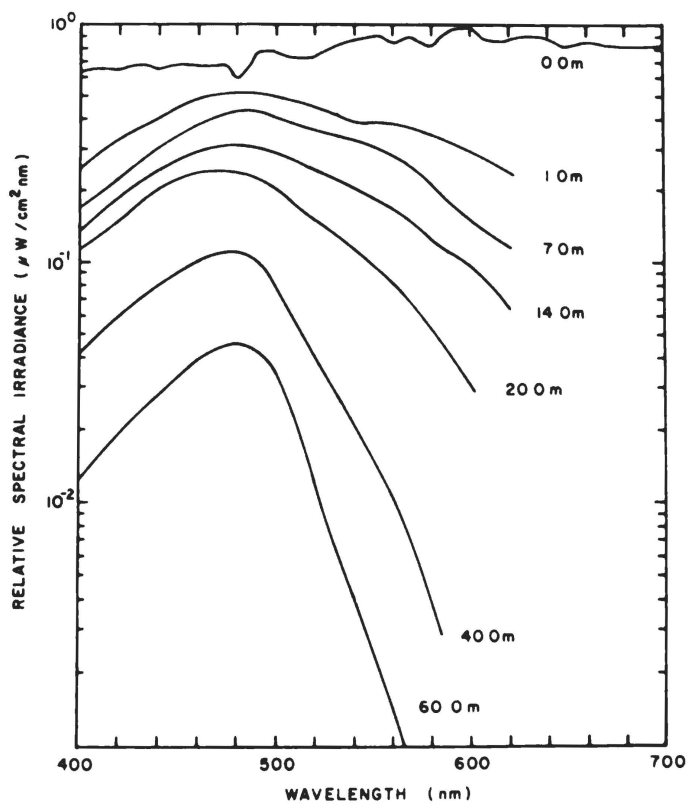
Figure 6 – The variation with depth of the spectral irradiance in Boston Harbor (May 24).
