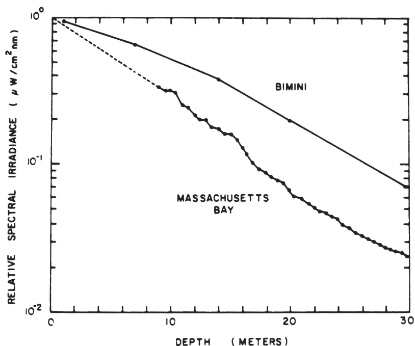
Figure 5 – Irradiance vs. depth at 530 nm at a point in Massachusetts Bay 20 miles off-shore from Boston (Aug. 22). There is a noticeable step-like attenuation due to stratified phytoplankton in the upper layers.
