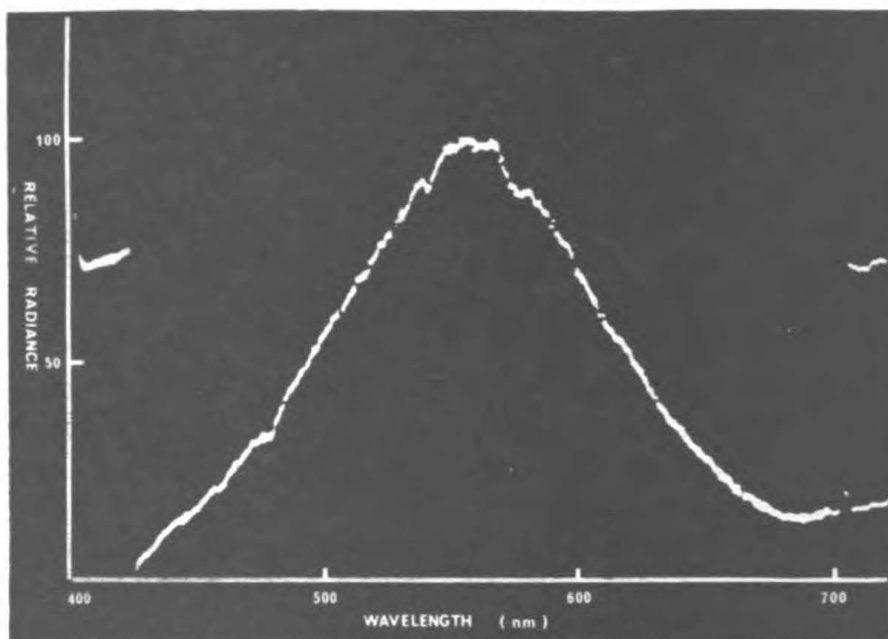
Figure 2 – Oscilloscope display of the output signal during a single spectral scan of the SLDS. Triggering and reference pulses are located at 400 nm and 700 nm.
