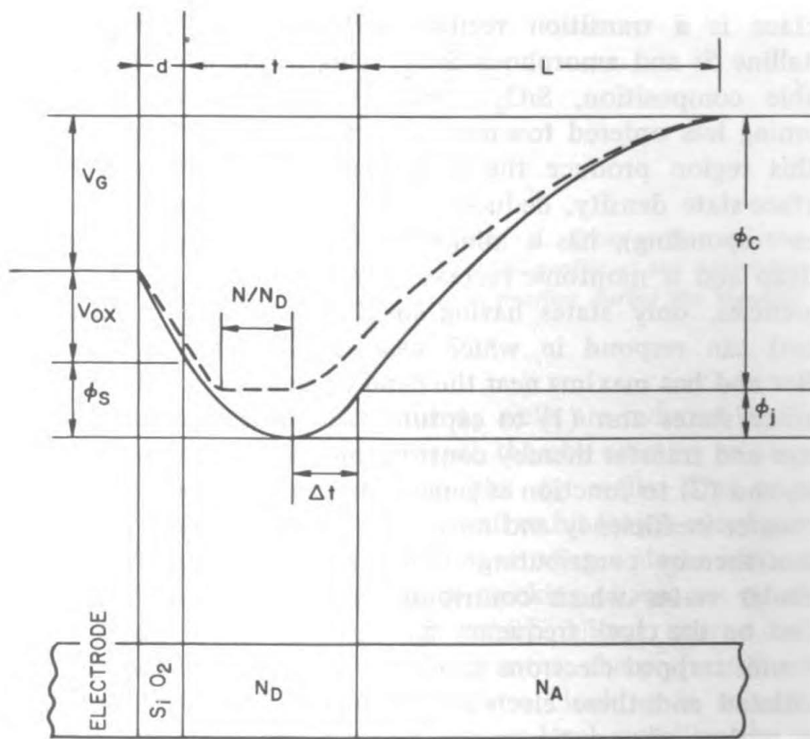
Figure 3—Potential vs. distance into the silicon for a buried-channel MOS capacitor. The solid curve shows the potential with no signal charge present ( N = 0 ). The dashed curve shows the potential with N carriers per unit area in the potential well.
