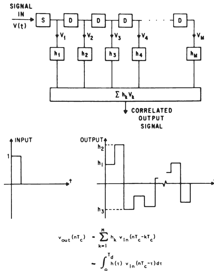
Figure 15—Block diagram of a CCD transversal filter.
