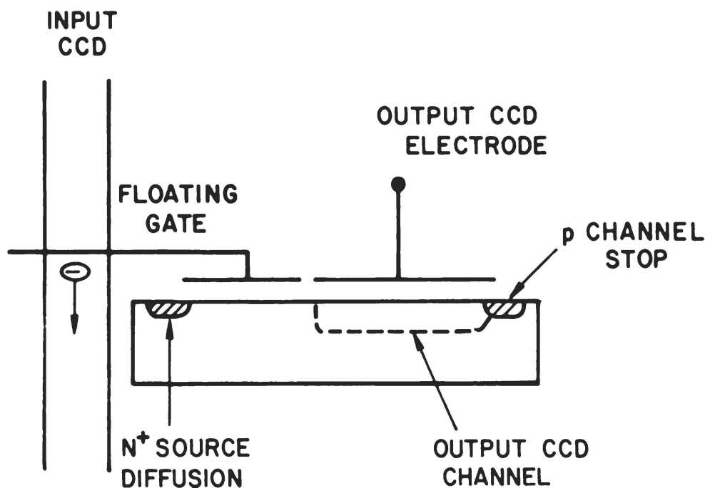
Figure 11—Schematic diagram of a floating-gate amplifier stage.
