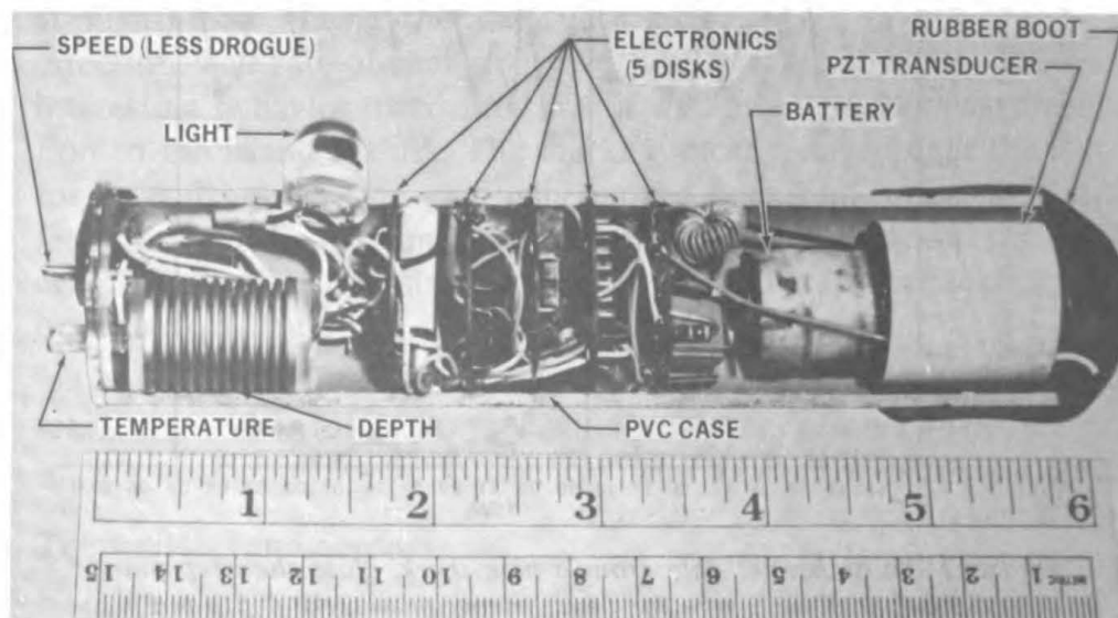
Figure 4—Mark III multichannel transmitter: cut-away view showing internal components of an 8-channel unit with sensors for depth, swim speed, light, and temperature. PZT = Lead-Zirconate-Titanate. PVC = Polyvinyl Chloride.
