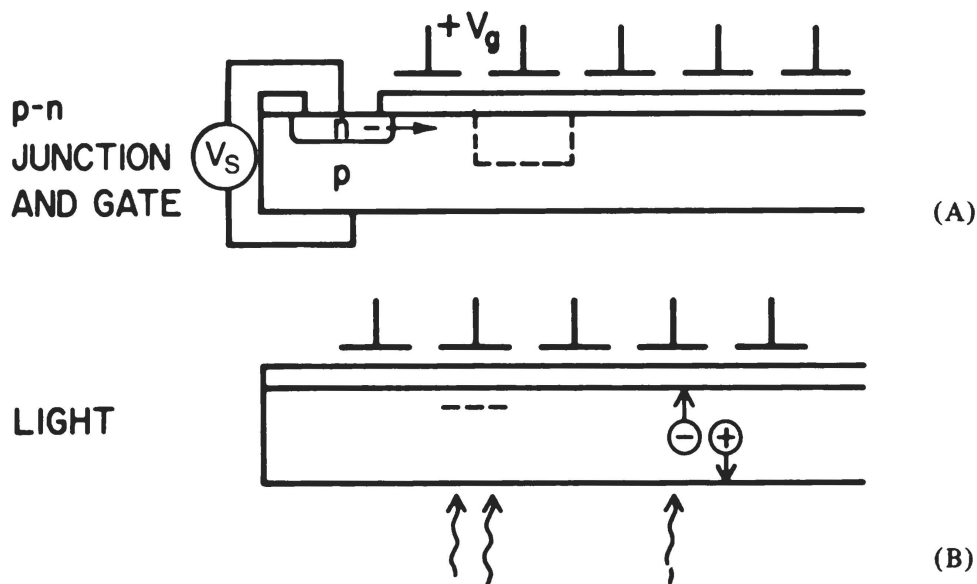
Figure 5—Input schemes for charge-coupled devices. A. Electrical signal input. B. Photon excitation
