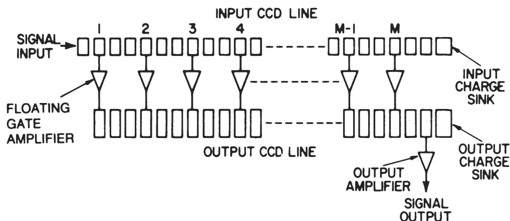
Figure 10—Schematic diagram of the distributed floating gate amplifier.
