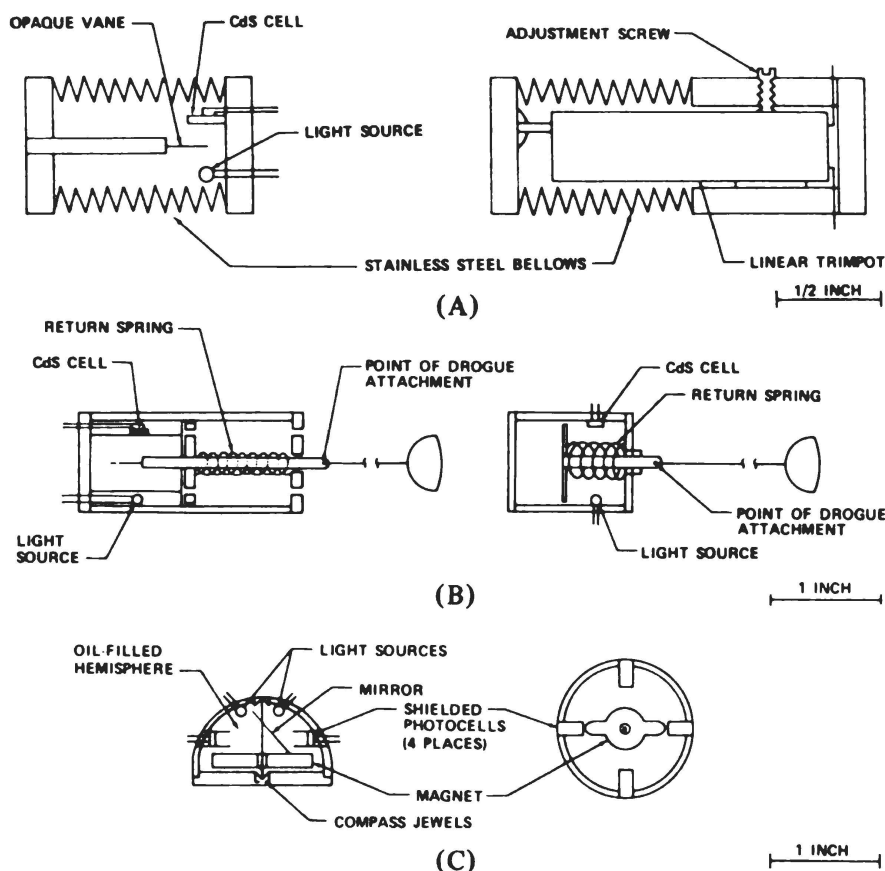
Figure 5—Some representative sensor types utilized in past transmitter packages: A, depth (pressure); B, swim-speed (water flow); C, compass heading (azimuth). All act as variable resistors. The light-photocell types utilize very low-power light-emitting diodes powered by zener-diode regulated voltage from the transmitter battery. Several newer versions are under development which are considerably smaller and without moving parts.
