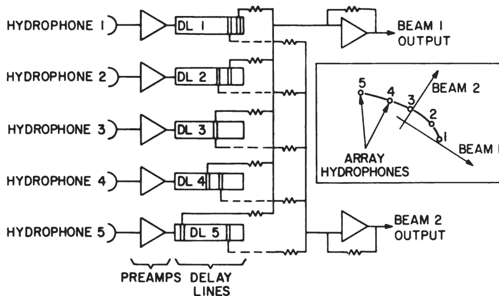
FIVE-HYDROPHONE, TWO-BEAM BEAMFORMER
