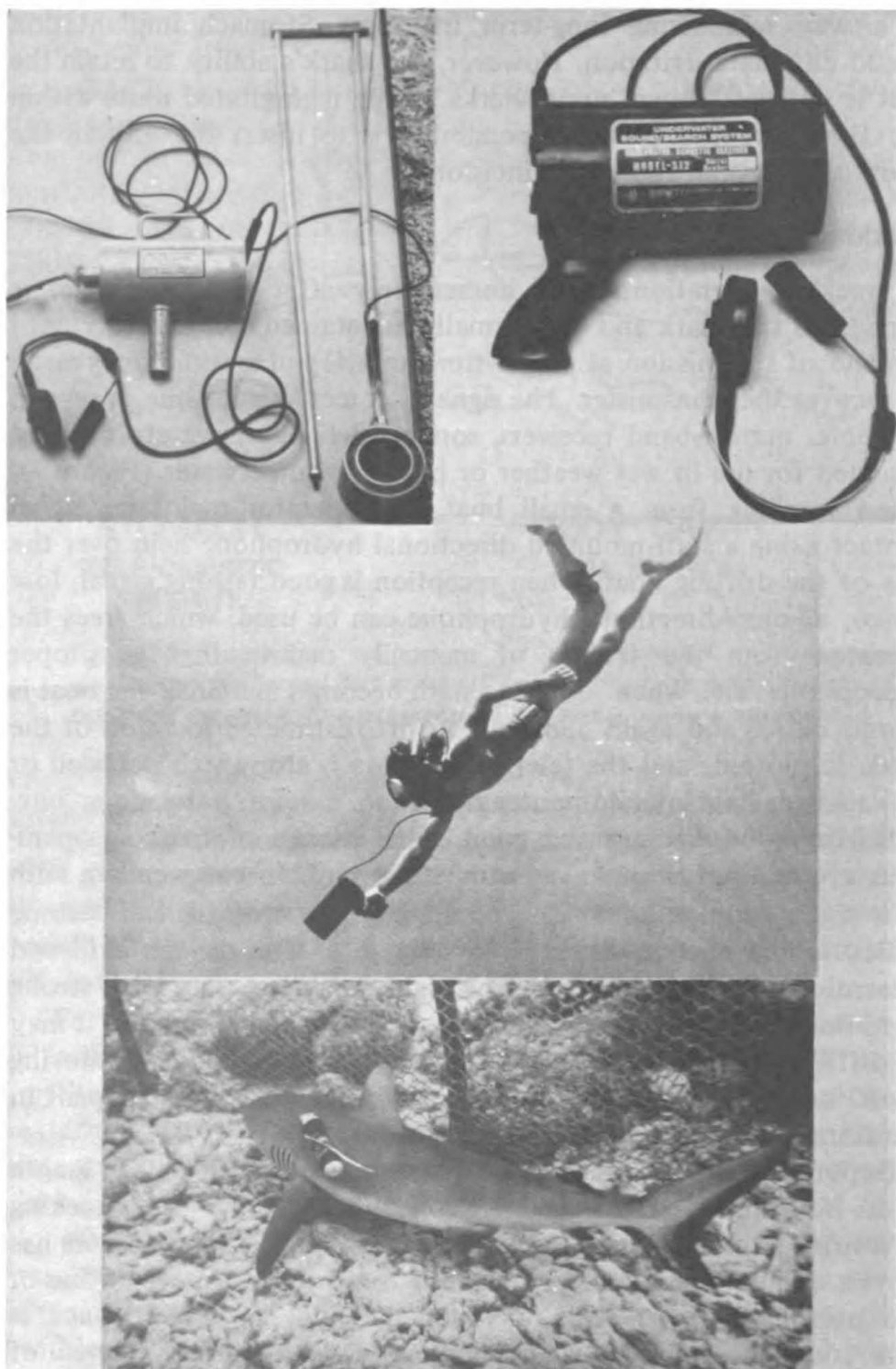
Figure 7—Ultrasonic telemetry receivers, DuKane (top left), and Burnett (top right). Center: free diver using Burnett unit underwater. Bottom: gray reef shark with externally attached Mark III transmitter (in fish trap prior to release for tracking). (Photos by R. McKenzie, top; D. Mosher, center; and R. Johnson.)
