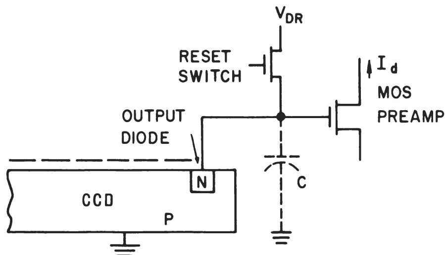
Figure 6—Output circuit for CCD.
