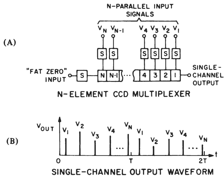
Figure 14—Diagram illustrating the operation of CCD's in time-division multiplexing. A. Multiplexer schematic. B. Multiplexer output.
