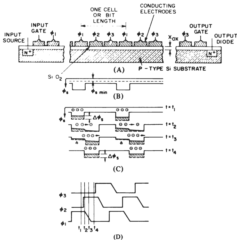
Figure 2—Charge coupled transfer process. A. Cross-section of the charge coupled structure. B. Surface potential profile at the beginning of the transfer cycle. C. Surface potential profiles during the transfer cycle. D. Three-phase clock waveforms
