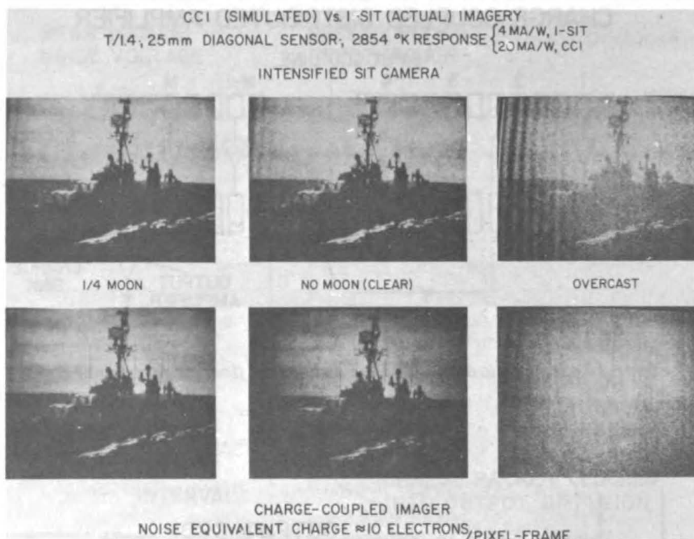
Figure 12—Simulation of cooled buried-channel frontside illuminated CCD area array performance vs. the performance of an I-SIT tube.
