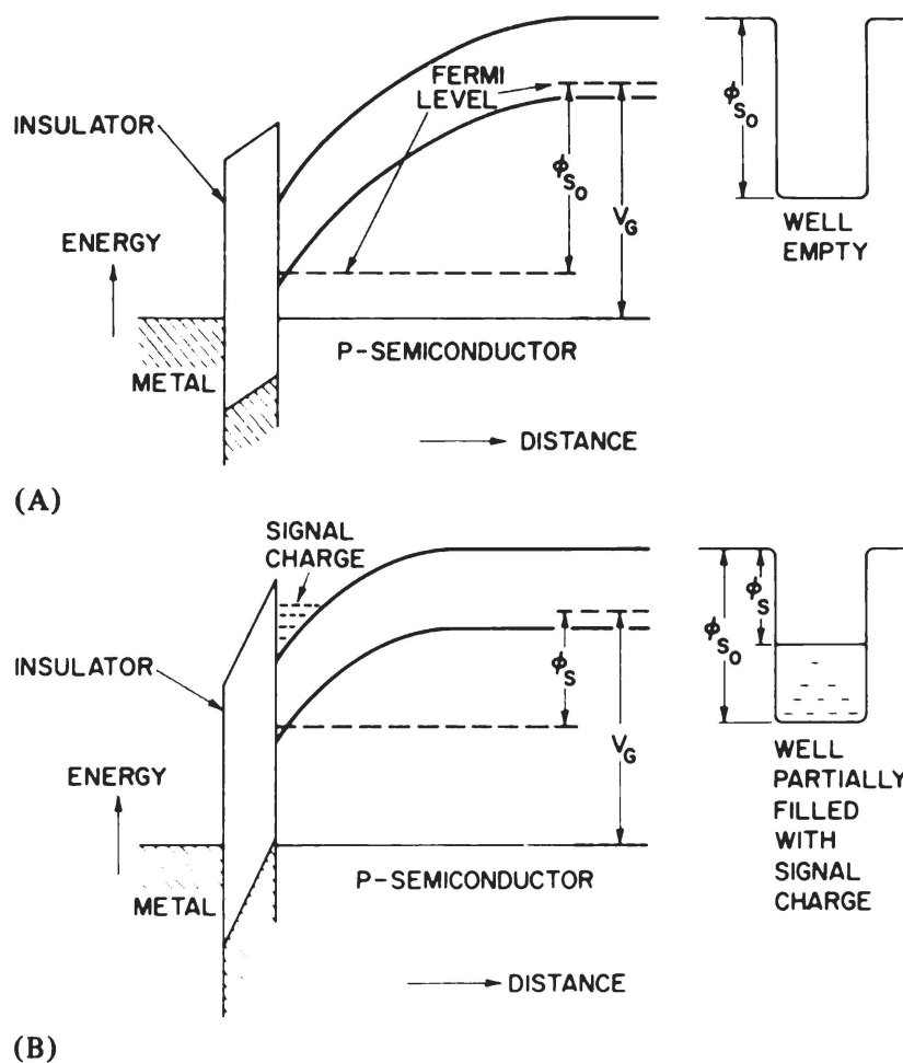
Figure 1—Energy level diagram of MIS capacitor. A. Empty potential well. B. Partially filled well
