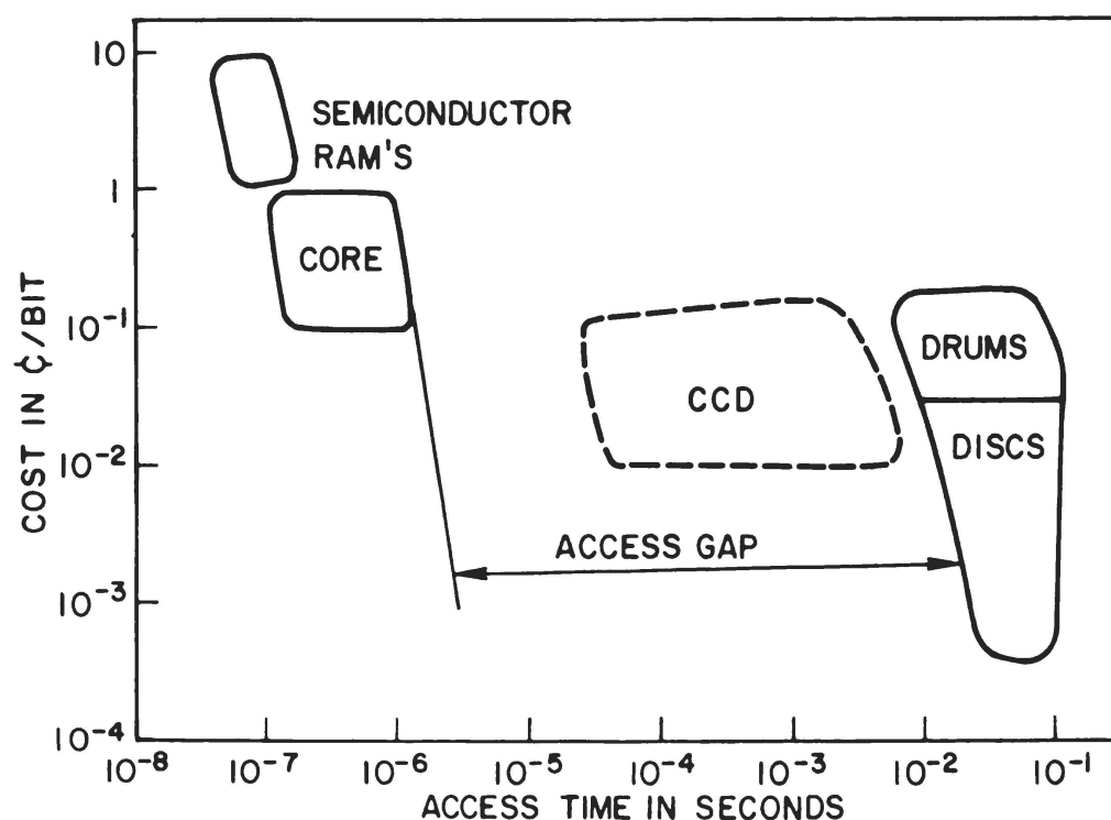
Figure 16—Memory cost (at the systems level) vs. access time.
