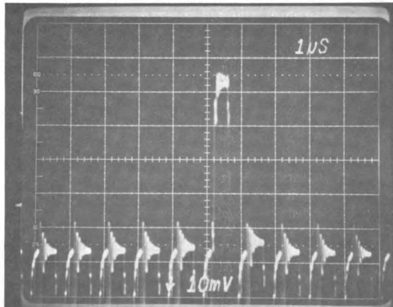
Figure 4—Oscilloscope traces of CCD output.
