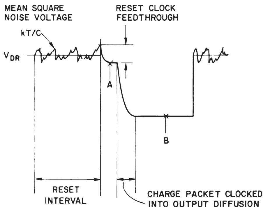
Figure 9—Output voltage waveform of a CCD operated in the reset mode.
