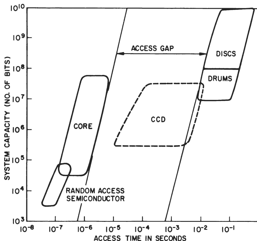
Figure 17—Memory-system capacity vs. access time.
