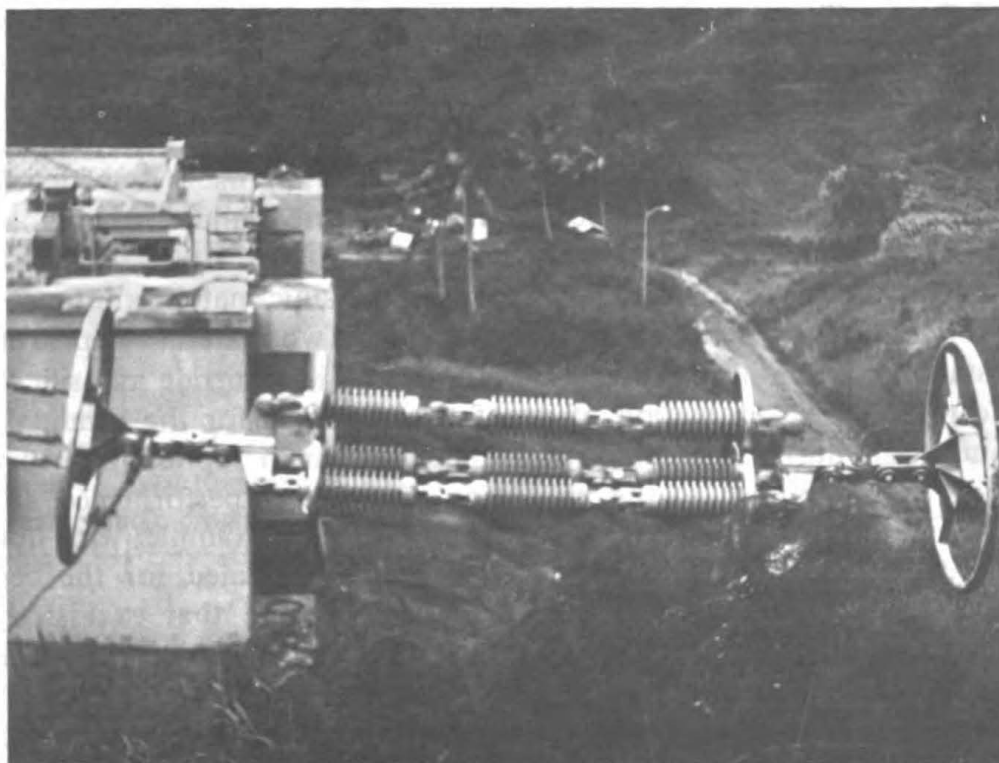
Figure 5 — Omega Station Valley Span, Haiku, Hawaii. The insulators in this figure serve a dual function: Support of load due to the cable; and electrical insulation of the cable from ground. Maximum load on these insulators is 40,000 pounds. Each of the nine insulators in this figure is approximately three feet long.
