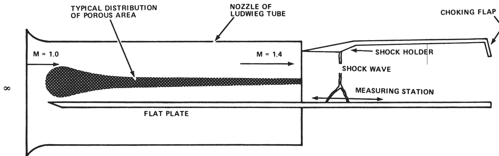
Figure 3 — Schematic of the shock wave—boundary layer interaction experiment in the Calspan Ludwieg tube
