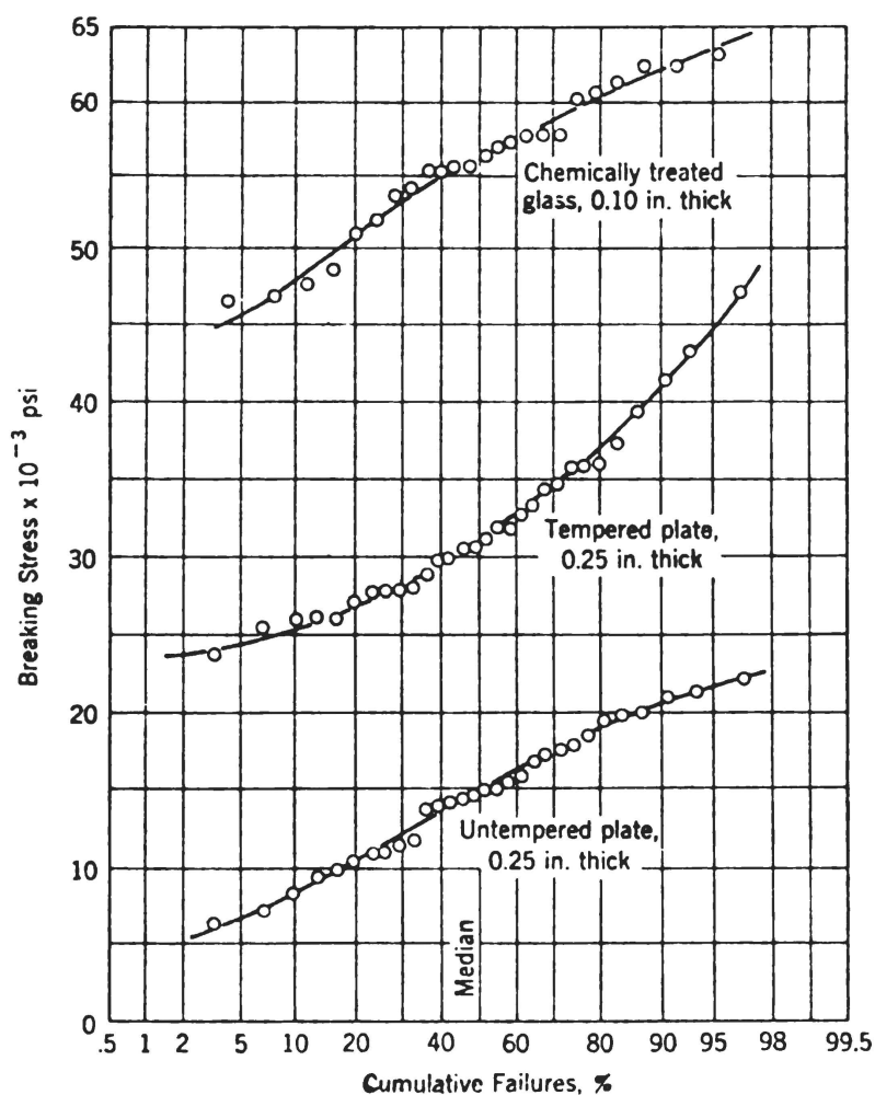
Figure 1 – Typical distribution of breaking stresses of glass. From the Encyclopedia of Chemical Technology , 2nd ed., vol. 10, pp. 533-604, John Wiley and Sons, Inc., (1966)
