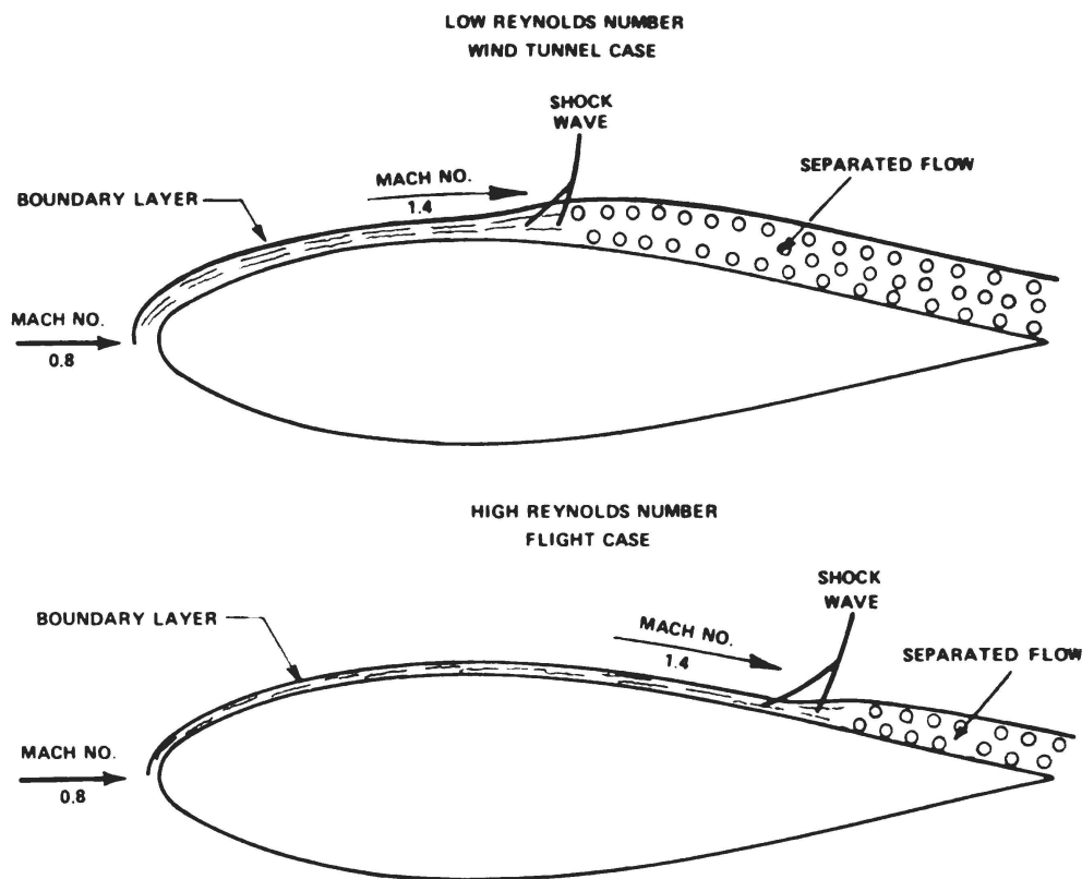
Figure 1 — Scale-effect on shock-induced separation
