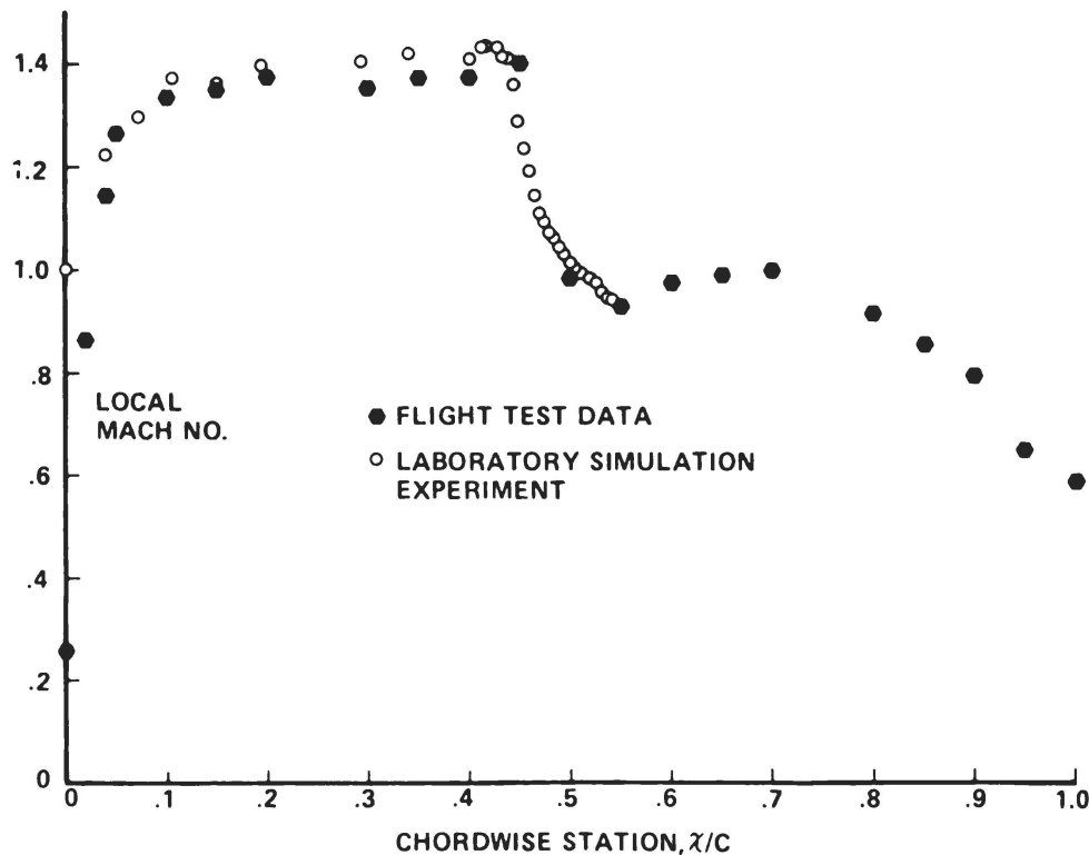
Figure 8 — Local mach number distribuion on a transonic airfoil
