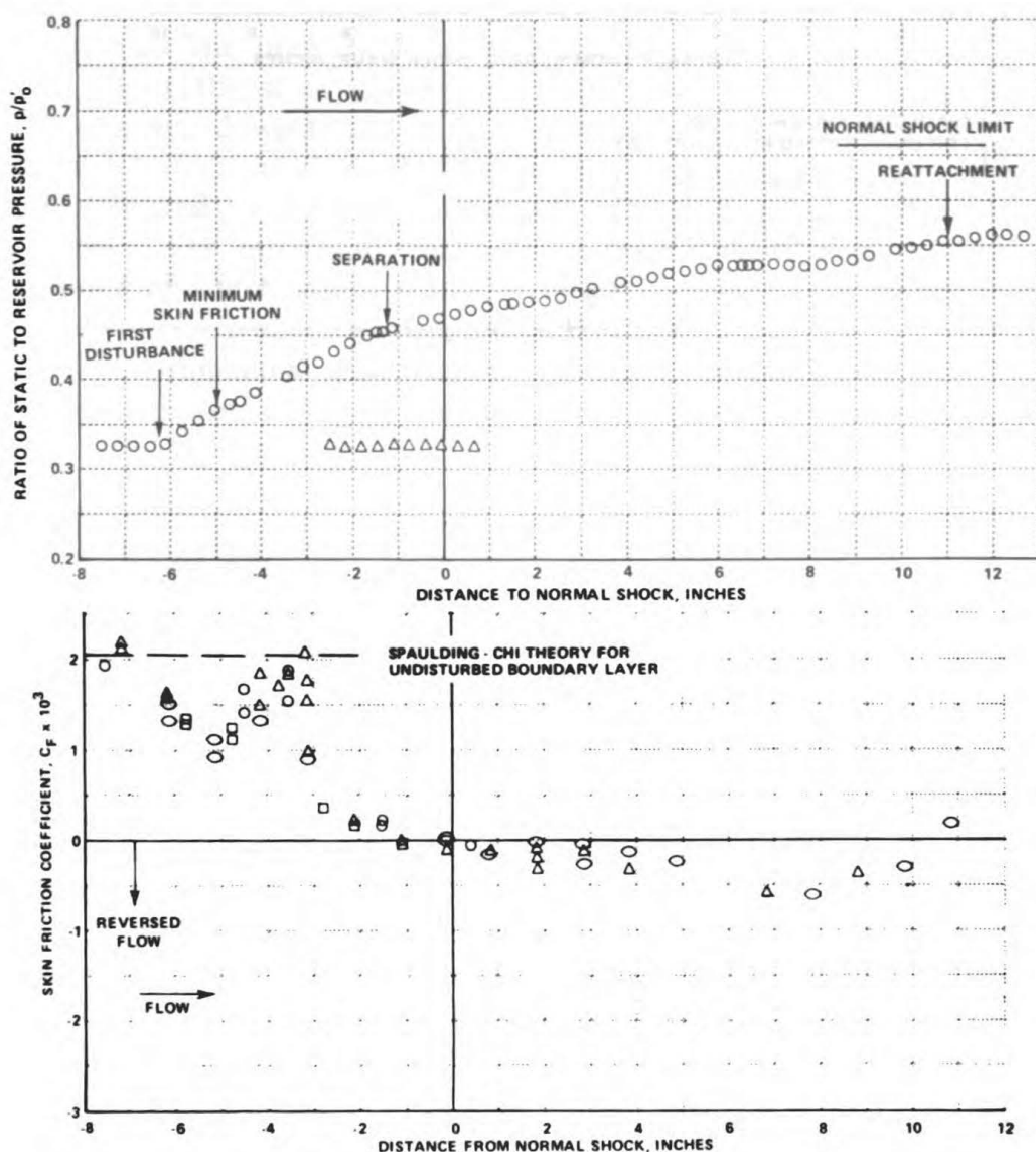
Figure 9 — Surface pressure and skin friction distributions in the interaction zone, Re = 9 \times 10^6
