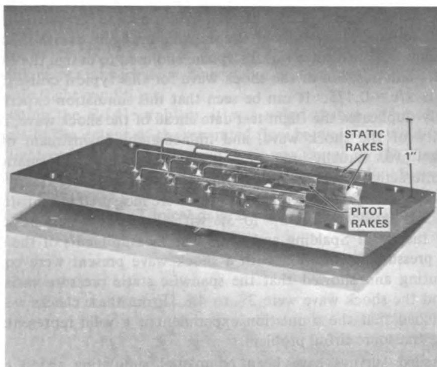
Figure 7 – Typical survey rake
