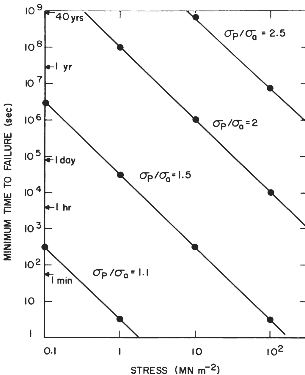
Figure 4 – Proof test diagram for porcelain used as electrical insulators. The minimum expected lifetime is given as a function of stress for a series of different proof test ratios. For an expected service stress of 2,000 p.s.i. ( \sim 14 \text{ MN/m}^2 ) the proof load must be 2.5 times the applied service load of 40,000 pounds to guarantee a lifetime of 40 years.
