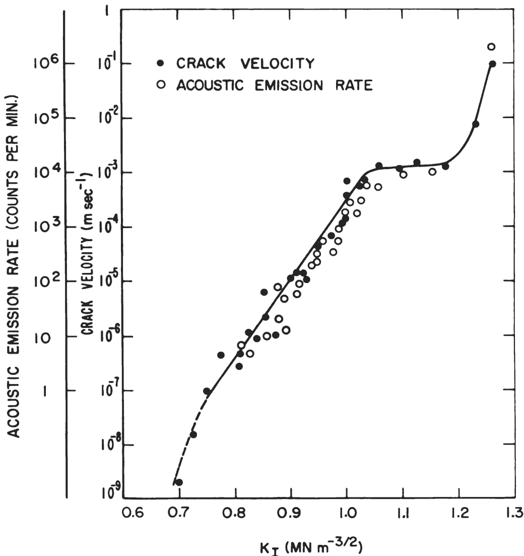
Figure 3 – Crack velocity and acoustic emission rate in porcelain as a function of applied stress intensity factor.
