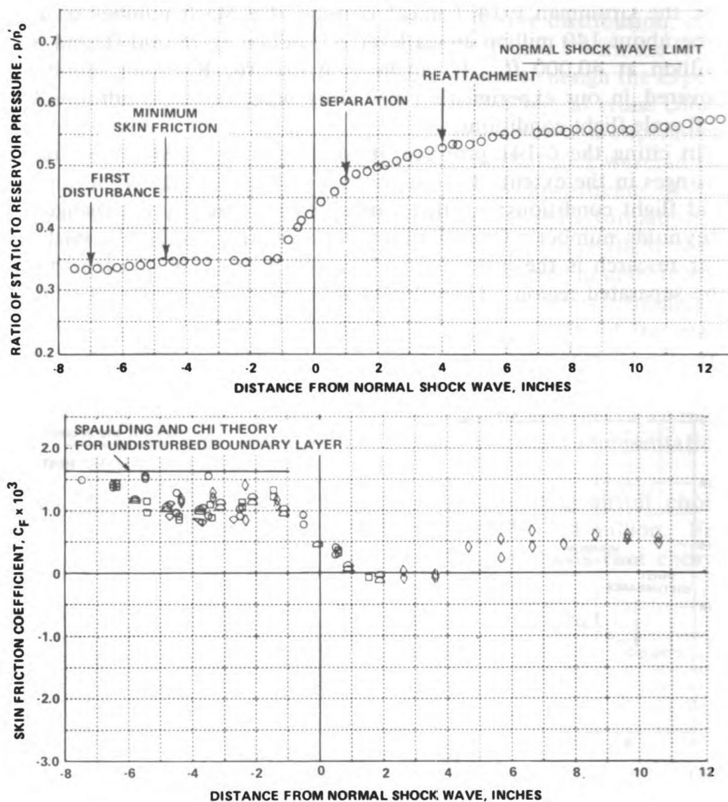
Figure 10 — Surface pressure and skin friction distributions in the interaction zone, Re = 36 \times 10^6
