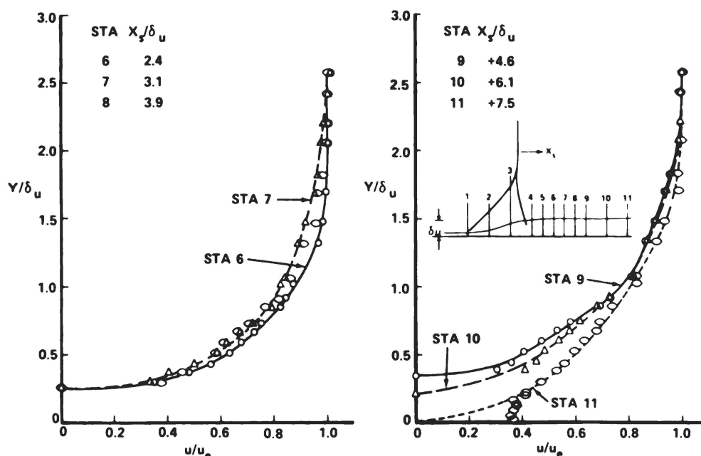
Figure 11 — Viscous layer profiles in the interaction zone Re_x = 9 \times 10^6
