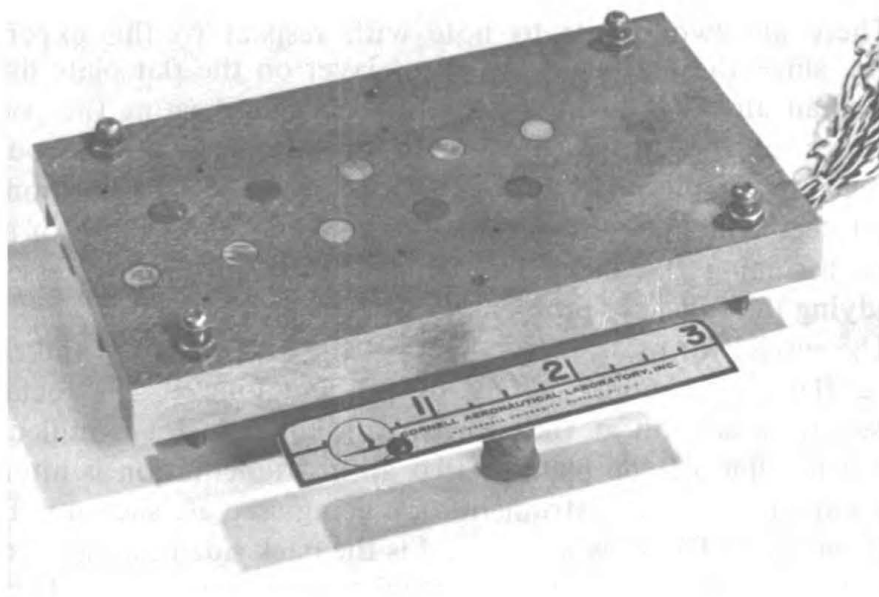
Figure 5 — Exposed surface of the skin friction and pressure survey plate
