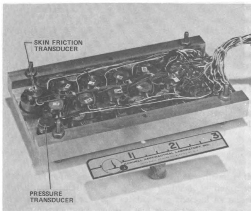
Figure 4 — Underside of the skin friction and pressure survey plate
