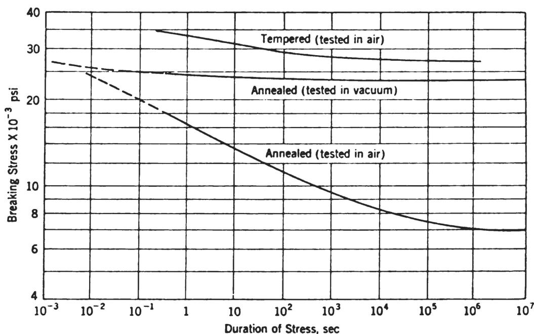
Figure 2 – Stress-time characteristics of glass at room temperature. From the Encyclopedia of Chemical Technology , 2nd ed., vol. 10, pp. 533-604, John Wiley and Sons, Inc., (1966)
