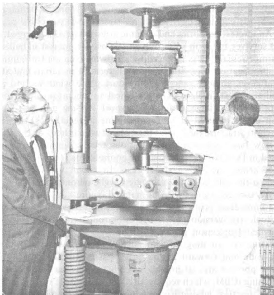
Figure 2—Preparation of a specimen under axial load for fracture test. Dr. Irwin is watching Mr. Clark in process of initiating crack in sheet specimen.
