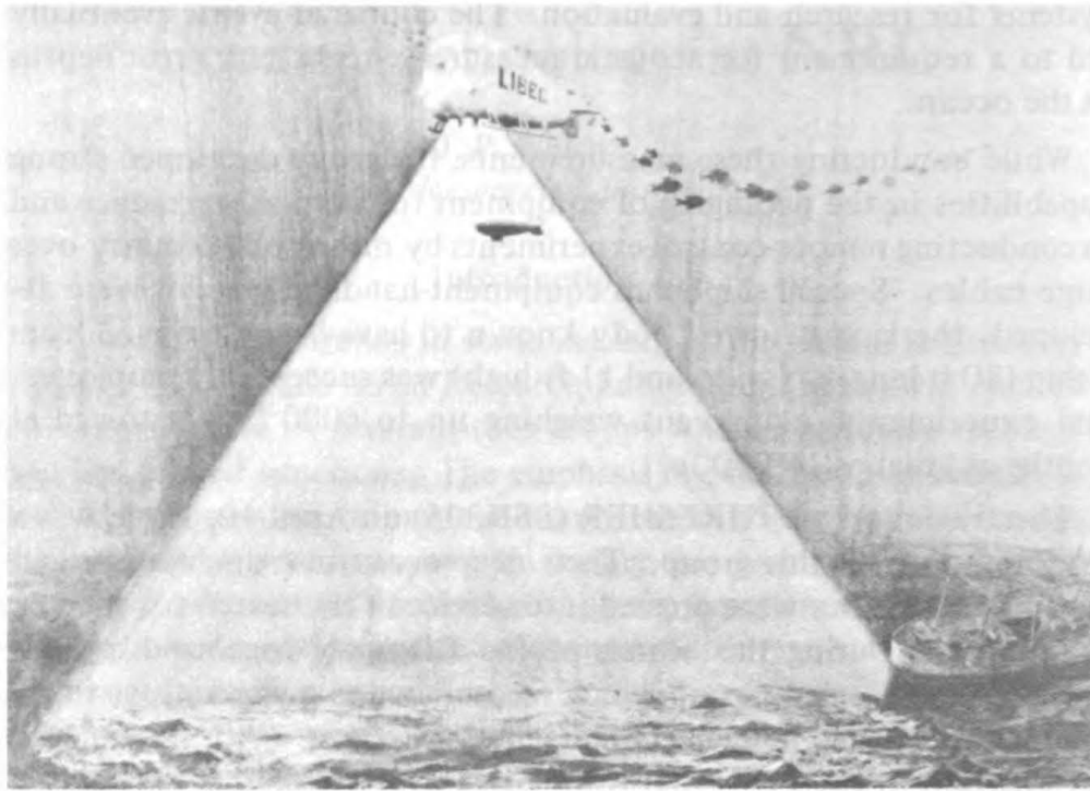
Figure 1—Extension of deep-sea photographic coverage by Light-Behind-Camera (LIBEC) system. Artist's conception illustrates lighting principle.
