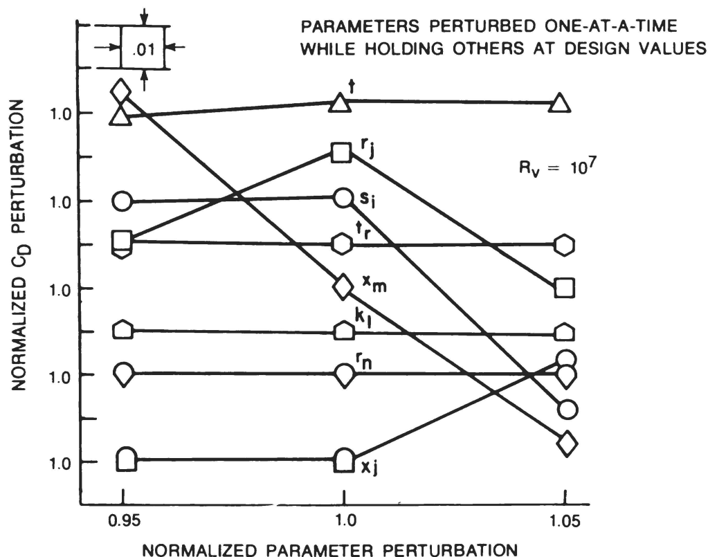
Figure 4. Perturbation studies on body X-35 at Reynolds number of 10^7 . A plus and minus five percent perturbation is made on each dimensionless parameter while the other seven parameters are held at their design values.
