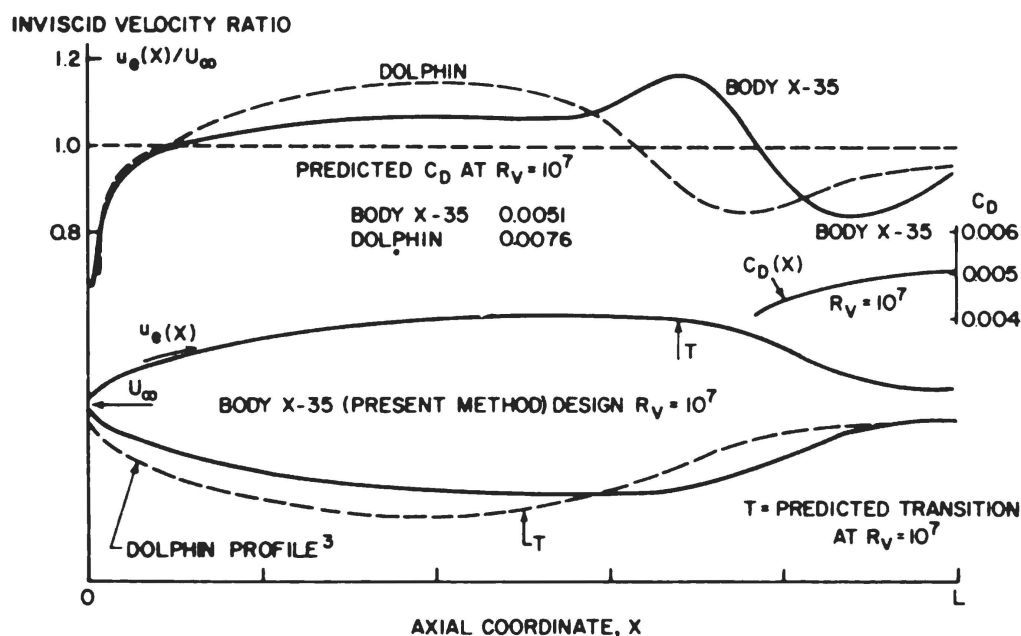
Figure 1. The design R_V (Reynolds number) of 10^7 for body X-35 corresponds to the Dolphin volume of 5.6 cubic feet at 40 knots in water. Body X-35 with its inviscid velocity distribution and C_D (drag coefficient) are shown here along with the Dolphin for comparison. The C_D for body X-35 is about one-third lower than that of the Dolphin at R_V of 10^7 .
