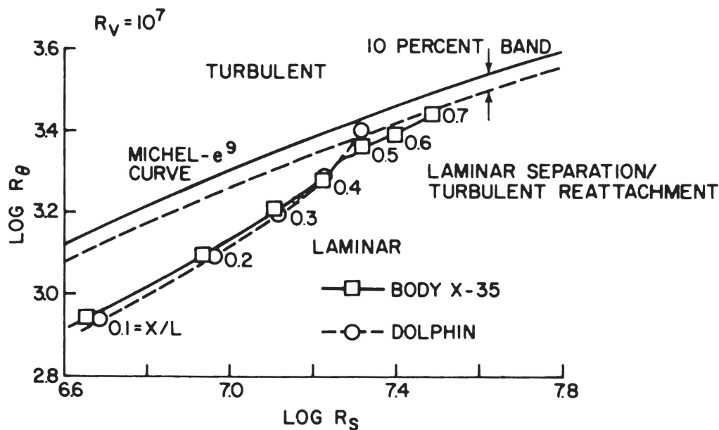
Figure 2. Transition predictions at R_V (Reynolds number of 10^7 for body X-35 and the Dolphin with the transition (Michel - e^9 ) curve.
