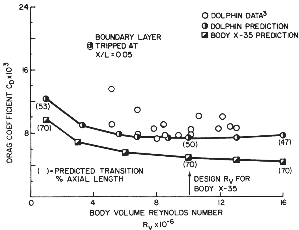
Figure 3. Predicted drag coefficients ( C_D ) for body X-35 and the Dolphin, as well as experimental data for the Dolphin over a range of Reynolds number.
