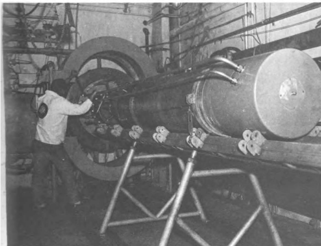
Figure 4—NUSC has the unique capability for system testing of an entire submarine-launched torpedo. In this photograph a technician is preparing a torpedo for total depth testing in the Center's propulsion test facility.
