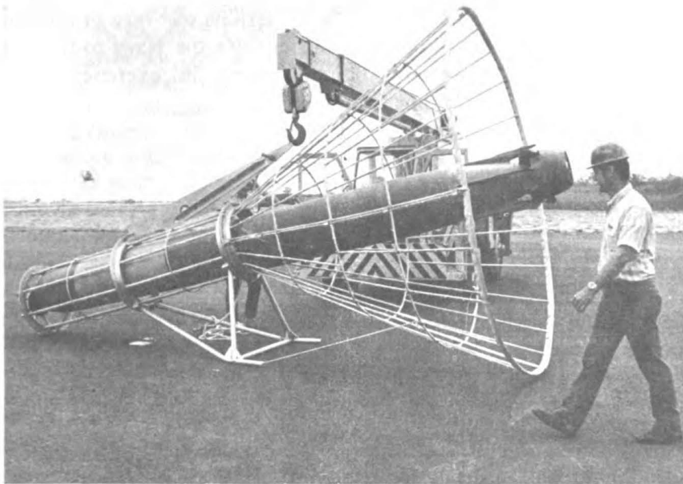
Figure 2 -Within minutes the torpedo is landed and ready for shore facility handling. The ferrying helicopter can be seen (left background) departing the station area for another exercise recovery. The cage is so constructed that surface abrasion or other damage to the torpedo casing (sometimes an aggravating problem with retriever-boat recovery) is negligible.
