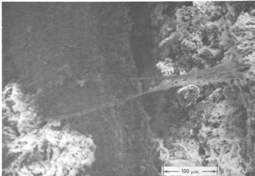
Figure 1 –This photomicrograph, taken with a scanning electron microscope, shows how the elastomer holds the zinc particles to the grid structure in a zinc plate from a cell that has been cycled 20 times. The electrodes are made using a technique for which NUSC has filed a patent application.
