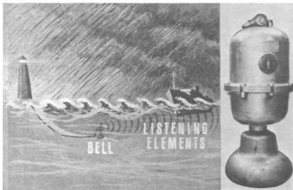
Figure 3 – Underwater navigation bell developed by the Submarine Signal Company was in fairly widespread use before World War I.
