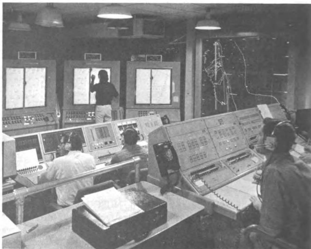
Figure 7—For range exercises, in-air and in-water tracking data and impact prediction plots can be displayed in this weapons range control room at the Atlantic Undersea Test and Evaluation Center (AUTC).
