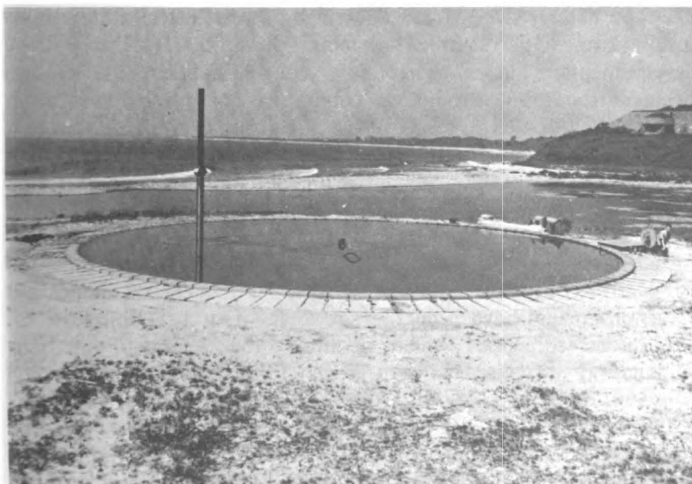
Figure 2—Submarine radio antennas and integrated communications systems are developed and tested at NUSC's unique test facility on Fishers Island. This tidal pond is the principal facility for testing buoyant cable antennas. There is no other such facility known.
