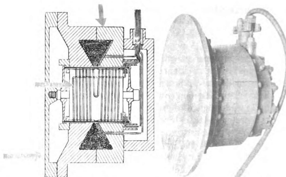
Figure 4 – Modified versions of this Fessenden oscillator, patented in 1913, were still in use in the 1950s.
