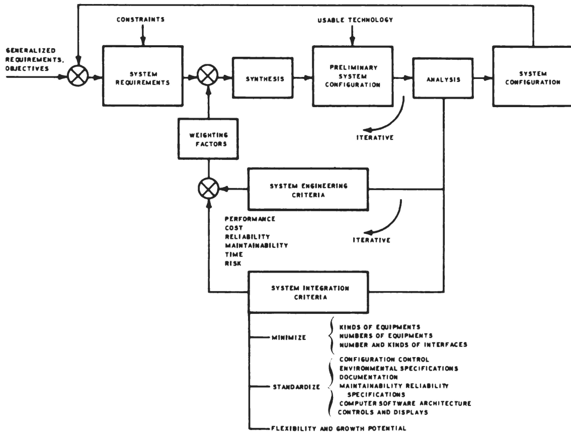
Figure 1 – General Combat System Engineering/Integration Process
