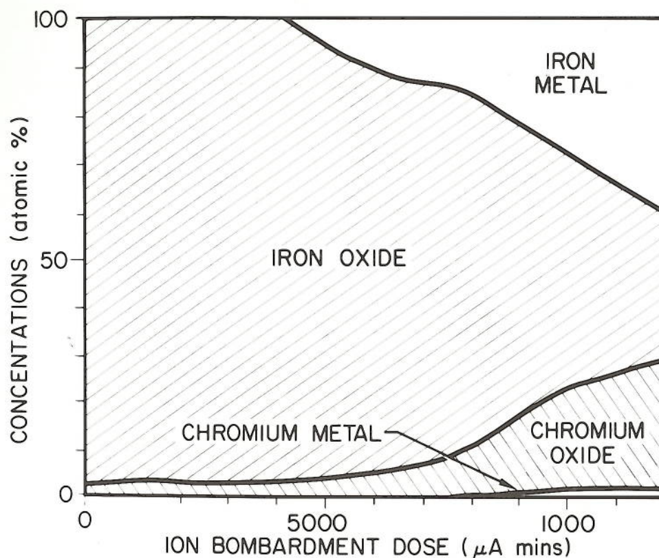
Figure 4: Composition profile of an iron-chromium steel surface obtained by XPS in conjunction with ion beam sputtering.
