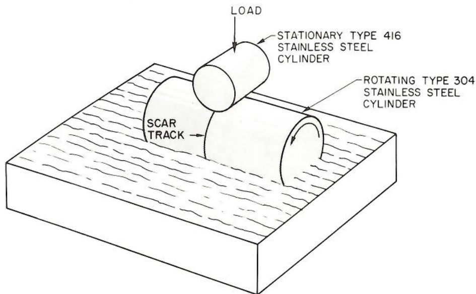
Figure 5: Experimental arrangement used to test the sliding-wear resistance of stainless steel.
