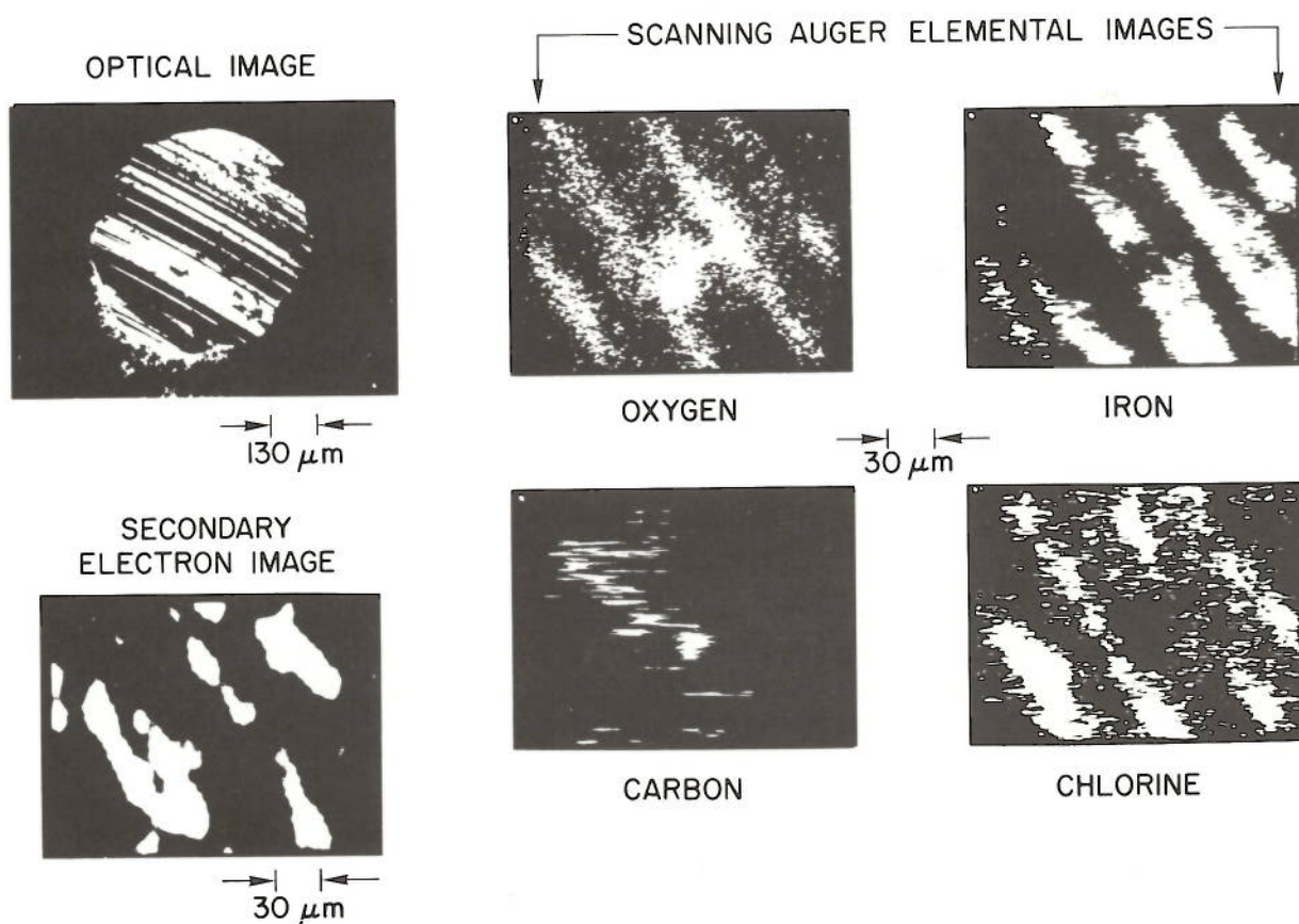
Figure 3: Optical, secondary electron and Auger electron images of a sputter-etched surface in a severe wear area. Striations in the optical image depict the physical contours of the wear scar. Patches of white on dark in the secondary electron image indicate that the wear scar is covered by a film non-uniform in composition or thickness. (The optical image is rotated slightly with respect to electron images.)
