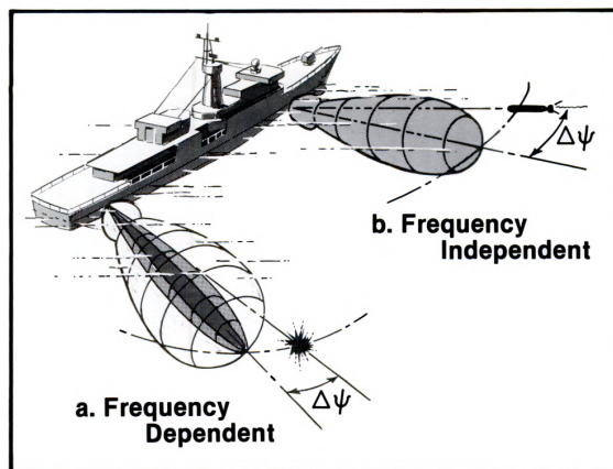
Figure 5. Passive surveillance of a wideband noisy point source ASW target in the clear; (a) with a frequency-dependent sonar antenna and (b) with a frequency-independent constant beamwidth sonar antenna.
