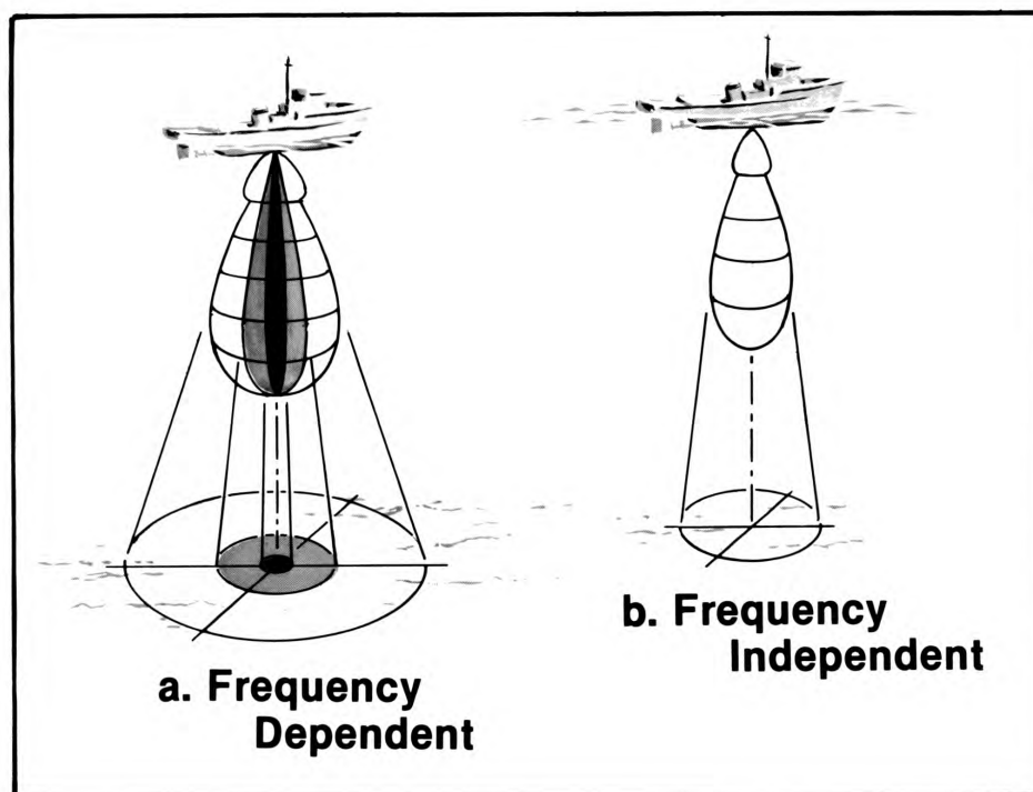
Figure 6. Active surveillance of an extended sea floor target area as in ocean resources prospecting or buried mine hunting; (a) with a frequency-dependent sonar antenna and (b) with a frequency-independent constant beamwidth sonar antenna.
