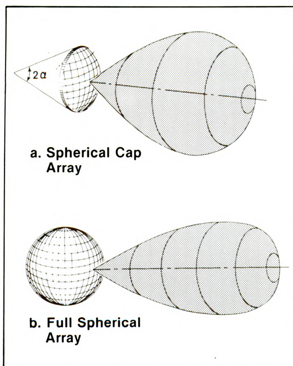
Figure 10. Spherical cap and full spherical array concepts for frequency-independent constant beamwidth beam formation; (a) spherical cap array of Rogers and Van Buren and (b) full spherical array of Jarzynski and Trott.
