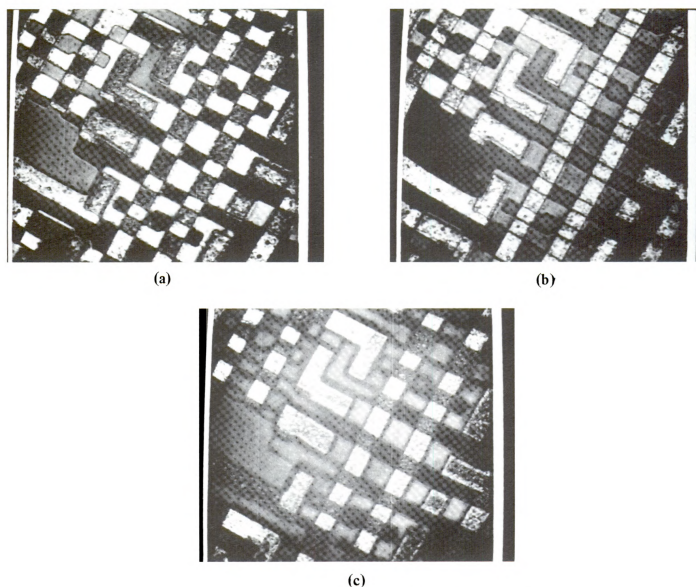
Figure 6: The acoustic appearance of integrated circuits in the acoustic microscope. For a given element the acoustic contrast changes and even reverses as the sample is moved to different focal positions. The changing contrast is a function of the layering structure of these devices and a careful comparison will reveal information on the elastic properties of the layers.
