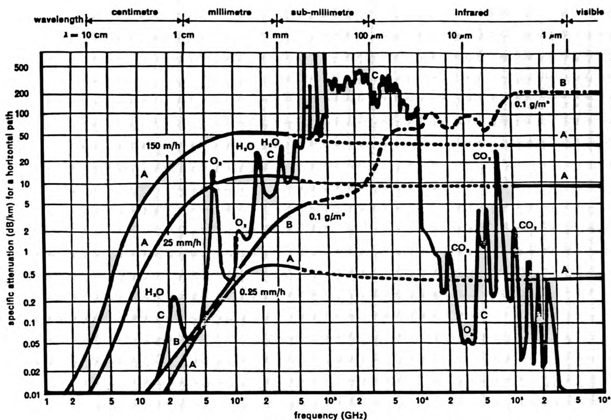
Figure 3. Specific attenuation of radiowaves, 1R, and visible light due to atmospheric constituents. The conditions assumed: T = 20^\circ\text{C} , vapor pressure = 7.5 \text{ cm/m}^3 . A = \text{rain} , B = \text{fog} , C = \text{gas} .
