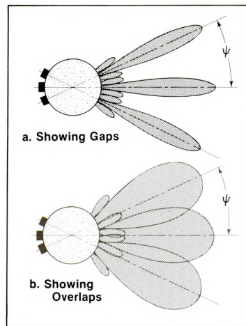
Figure 4. Multiple beam formation with an ordinary Luneberg lens equipped with a retina of wideband transmitting or receiving elements; (a) showing gaps between the beams at high frequencies and (b) showing overlaps of the beams at low frequencies.
