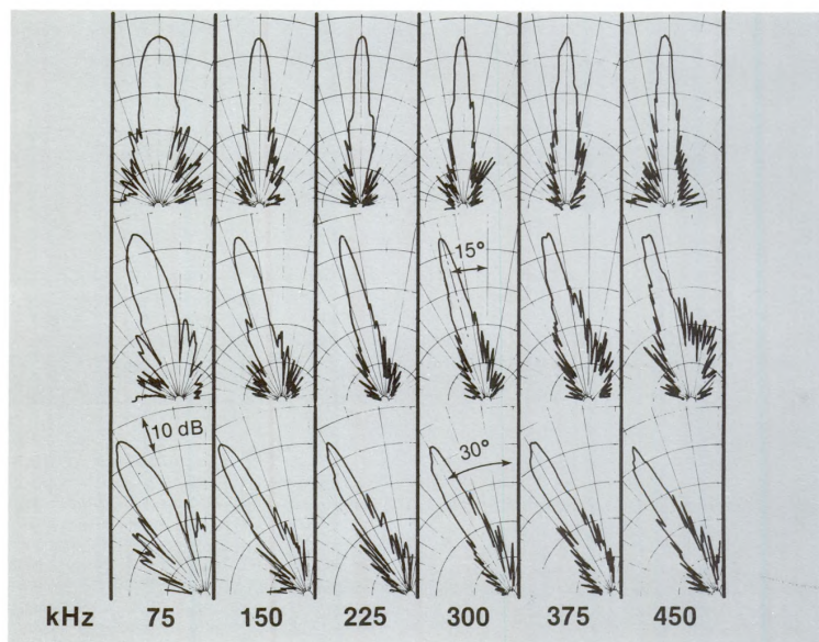
Figure 8. Experimentally measured frequency-independent acoustic lens-acoustics filter plate receiving beam patterns taken at various frequencies and scan angles showing approximately constant beamwidths of about 4 at frequencies above 75 kilohertz.
