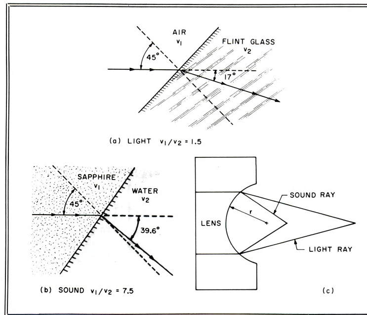
Figure 1: The application of Snell's Law for light waves (1a) and sound waves (1b). A spherical surface (1c) will have a different focal length for these two wave types.
