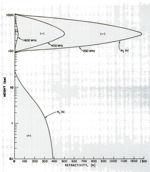
Figure 2. Radio refractivity versus altitude. Representative ionosphere profiles are shown for 250, 400, and 1600 MHz.
