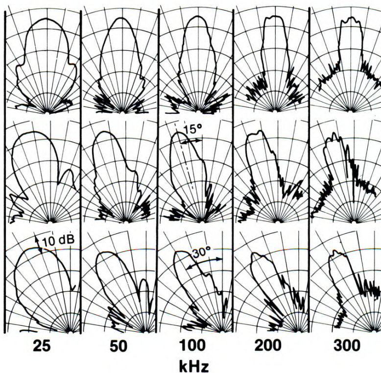
Figure 3. Experimentally measured frequency-independent acoustic lens-acoustic filter plate receiving beam patterns taken at various frequencies and scan angles showing approximately constant beamwidths of about 12^\circ at frequencies above 25 kilohertz.
