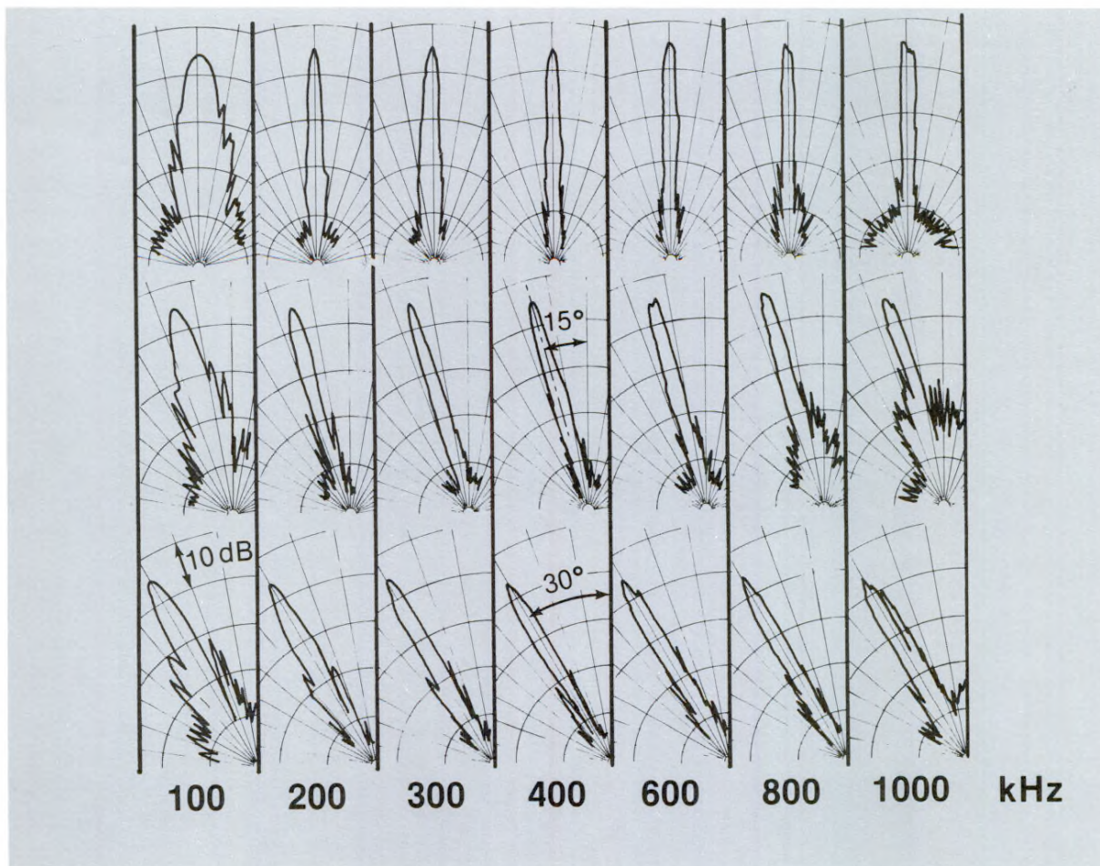
Figure 9. Experimentally measured frequency-independent acoustic lens-acoustic filter plate receiving beam patterns taken at various frequencies and scan angles showing approximately constant beamwidths of about 2^\circ at frequencies above 100 kilohertz.
