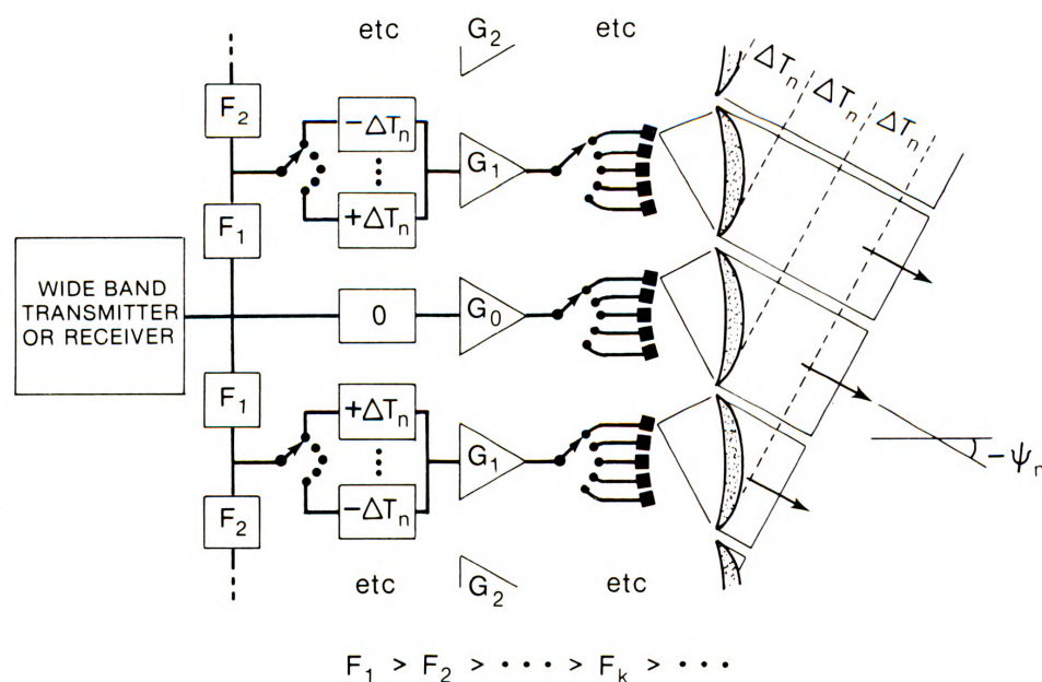
Figure 11. Mosaic-lens array antenna concept of Sternberg and Anderson for multiple or scannable approximately frequency-independent, approximately constant beamwidth beam formation suitable for large scale applications.
