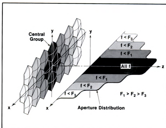
Figure 12. Mosaic-lens array antenna concept for approximately frequency-independent fan beam formation using hexagonally-cut lenses with a central group of four lenses showing the approximate aperture spectral distribution and shading function when the fan beam is pointed in the z -axis direction and fanned in the y , z -plane.
