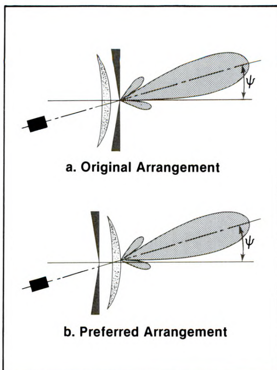
Figure 2. Alternative acoustic lens-acoustic filter plate mounting arrangements; (a) original arrangement and (b) preferred arrangement.
