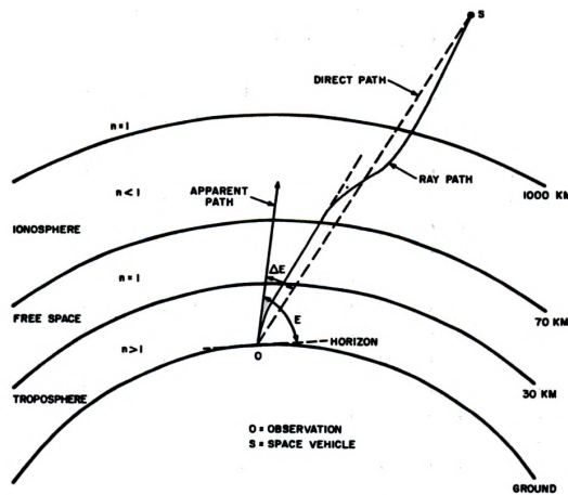
Figure 1. Radiowave Trajectory through the Troposphere and Ionosphere.
