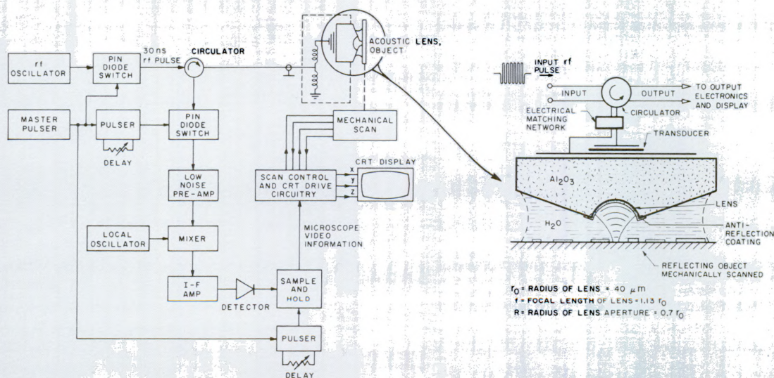
Figure 3: The schematic of the overall electronic system (3a) used in the scanning microscope and the detail of the principle elements of the acoustic lens configuration (3b).
