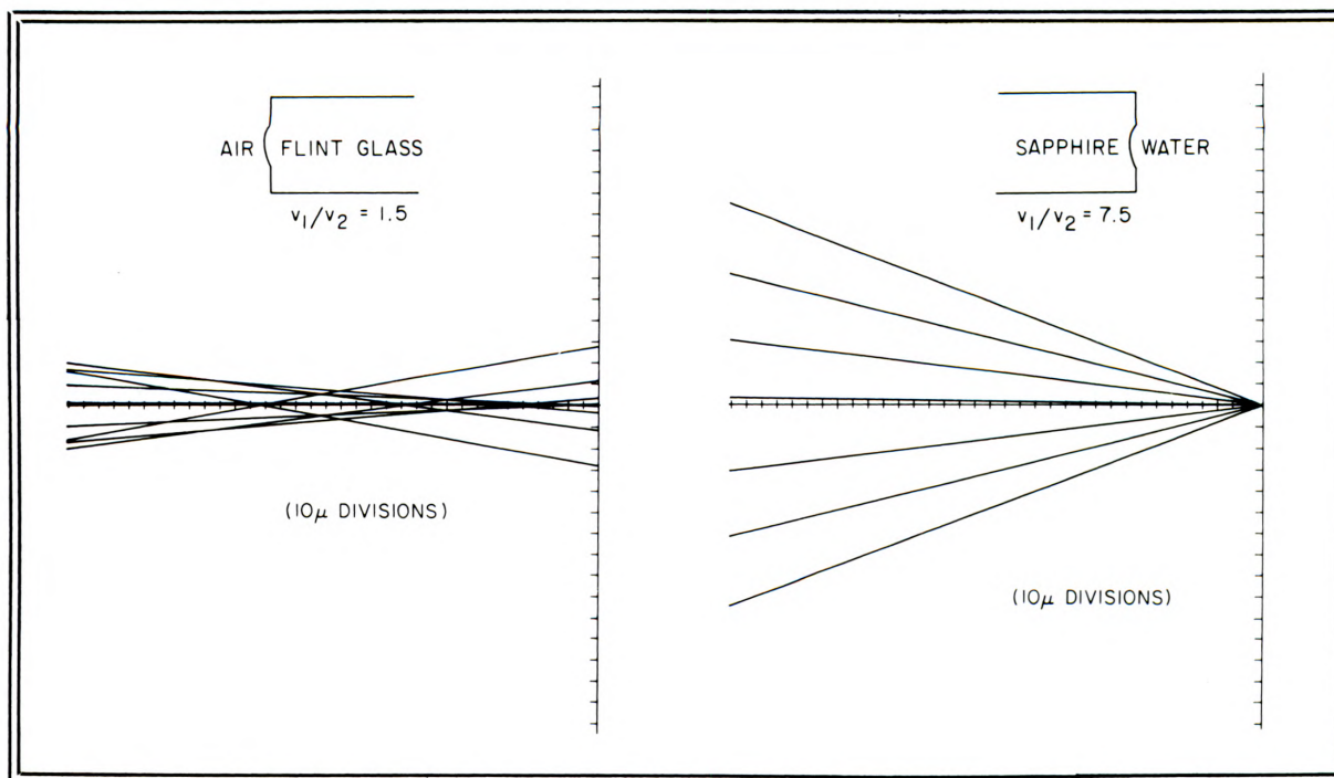
Figure 2: A comparison of the focusing strength of the optical system (left) and the acoustic system (right) as illustrated with ray tracing. The weak refraction of optical waves produces spherical aberrations which limit the minimum size at the beam waist. The aberrations in the acoustic case are not important.
