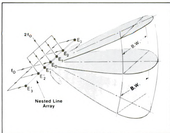
Figure 7. Nested line array concept of Hixson and Au for formation of a frequency-independent fan beam with the same azimuth beamwidths at frequencies f_0 and 2f_0 and approximately constant azimuth beamwidths at intermediate frequencies.
