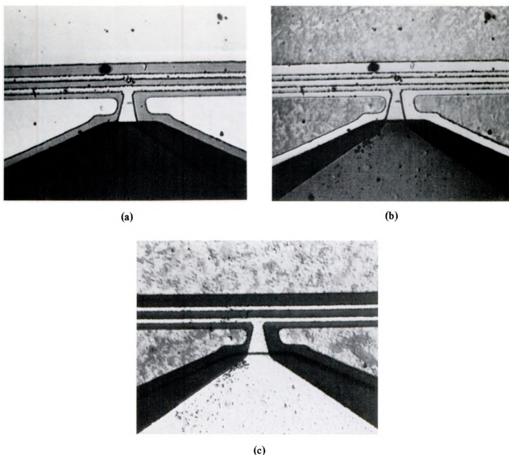
Figure 7: The acoustic micrograph from the cryogenic microscope. The liquid used here is argon near 80^{\circ}\text{K} . The sample is a field effect transistor built on a wafer of gallium arsenide. The width of the two parallel lines is one micron. The two acoustic images (a) and (b) are taken at different focal positions. The optical comparison is given in (c).
