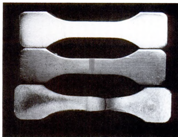
Figure 18. Tensile test samples of 4140 steel solid state bonded with a 1.6%C UHC steel. The two samples on the top are illustrated in the as-machined condition, unetched and etched respectively. The sample on the bottom is shown after testing at room temperature. The sample failed in a region away from the welded zone attesting to the soundness of the UHC steel—4140 steel interface.
