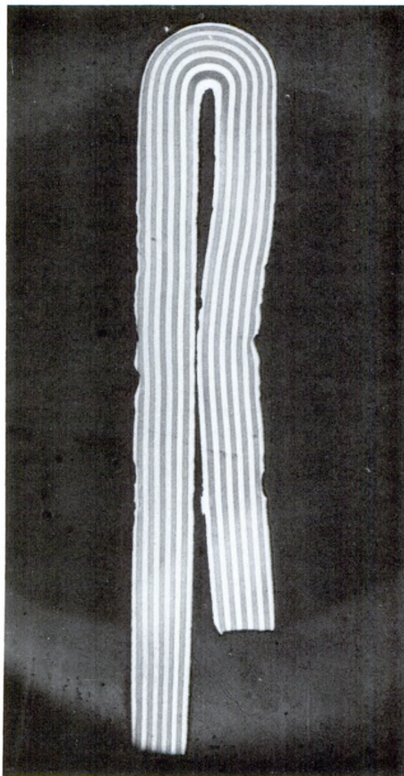
Figure 13. A zero T bend is readily achieved in an eleven-layer laminated composite of a 1.6% C UHC steel—1005 steel at warm temperature (600°C). The uniform deformation of each layer, with no evidence of fracture, attests to the possible superplastic nature of the laminated composite. The thickness of the composite is 2.5 mm.
