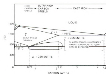
Figure 4. The above Fe-C phase diagram illustrates the range of composition and temperature where UHC steels can be superplastic if they are made sufficiently fine grained. A high carbon content is needed in order to introduce a large volume fraction of cementite particles for stabilization of the fine ferrite grains.
