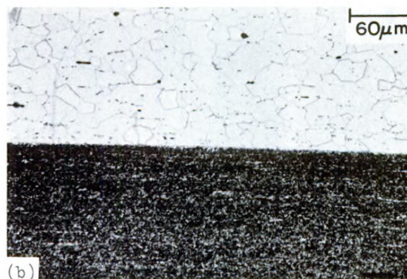
Figure 16. Photomicrograph of the interface of a laminated Adze Blade (dated 400 BC; attests to the metallurgical skill of the blacksmiths of ancient time (a). The bond is compared with the UHC steel/mild steel composite press bonded at Stanford (b). The authors thank Dr. Robert Maddin for permission to publish the photograph.
