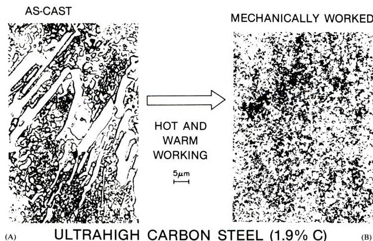
Figure 5. Optical photomicrographs of a 1.9% C steel. (A) Reveals coarse proeutectoid cementite particles in a matrix of ferrite and cementite in the as-cast state and (B) reveals fine equiaxed structure of ferrite grains containing submicron cementite particles after hot-and-warm working.
