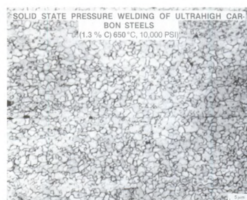
Figure 11. The above photomicrograph illustrates that superplastic UHC steel plates (1.3%C) can be readily solid-state diffusion bonded in air at relatively low temperature (0.51T m ) and low pressure (69 MPa). A line of demarcation can be seen at the bond interface because the cementite particles and ferrite grains are flattened at the interface, leading to flat ferrite grain and interphase boundaries.
