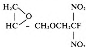
Isomeric fluorodinitroethyl glycidyl ether (FNGE) ( \text{C}_5\text{H}_7\text{N}_2\text{O}_6\text{F} )
