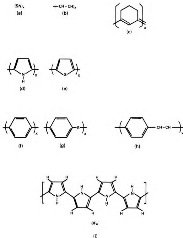
Figure 3. Conducting Polymers: (a) polysulfurnitride, (b) polyacetylene, (c) poly-1,6-heptadiyne, (d) polypyrrole, (e) polythiophene, (f) polyparaphenylene, (g) polyparaphenylenevinylene.
