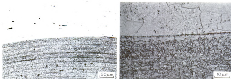
1005—ULTRAHIGH CARBON STEEL (1.3 % C) LAMINATE COMPOSITE NOT HEAT TREATED
