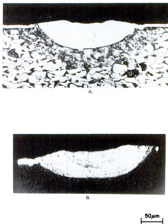
Figure 2. (a) Polished and etched cross section of an AISI 1018 steel coupon which was coated with an 8 \mu\text{m} thick layer of chromium and laser surface alloyed using a focused 5 kW laser swept at 50 cm/sec. (b) A chromium x-ray display of the cross section in (a).
