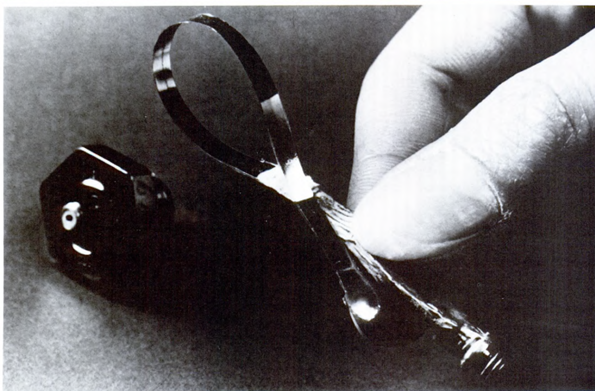
Figure 1. The advantages of weight, flexibility and size of a piezoelectric transducer over conventional ceramic devices are illustrated in this photo. The polymer device weighs 0.3 milligram (without the metal lead) while the ceramic device weighs 21 grams.
