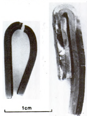
Figure 14. A warm-pressed two-layer laminated composite of a 1.3%C UHC steel/mild steel is bent at room temperature. Photomicrographs of the interface at the bent region reveal no sign of delamination attesting to the sound metallurgical bond in the laminate.
