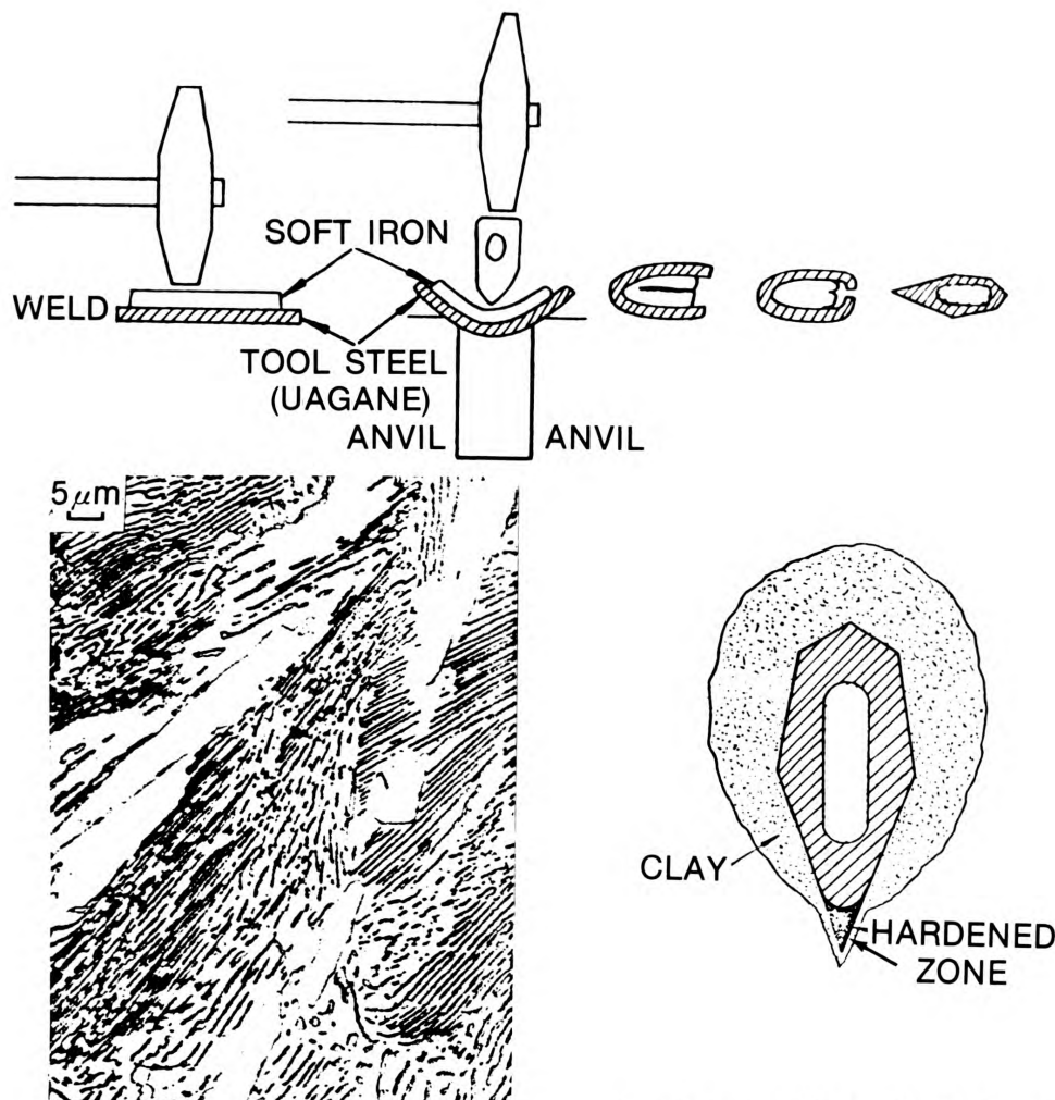
Figure 3. Japanese blacksmiths of ancient times made laminated tools by solid state bonding ultrahigh carbon (UHC) steels, known as uagane, to soft iron. After hot forging, the laminated tool was heat-treated to yield a hard cutting edge (adapted from E. C. Bain [14] ).
