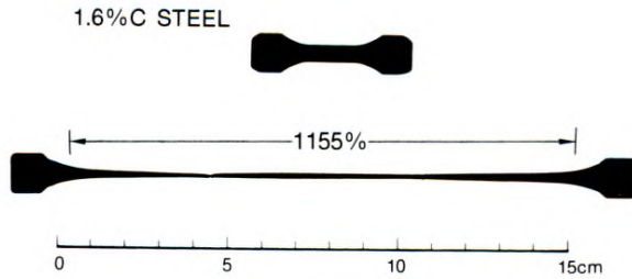
Figure 6. The above photograph illustrates a sample of a fine-grained UHC steel (1.6%C) deformed superplastically at 650°C. The initial engineering strain rate was 1% per minute.
