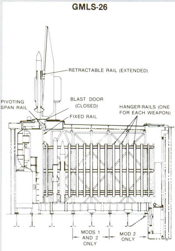
Figure 17. Mark-26 guided missile launch structure produced at NIROP Navy surface combatants.
