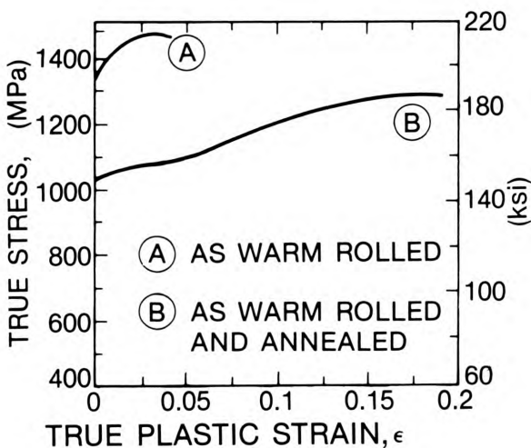
Figure 8. True stress-true strain curves for a 1.3%C steel at room temperature. Sample A was warm worked extensively at 565°C with no annealing after warm-working. Sample B was annealed for 20 min. at 650°C after warm-working at 565°C.
