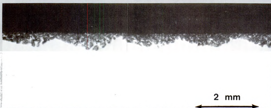
Figure 10. Sectional view of Ti-6Al-4V sample injected with TiC. Surface was ground flat after injection processing.
