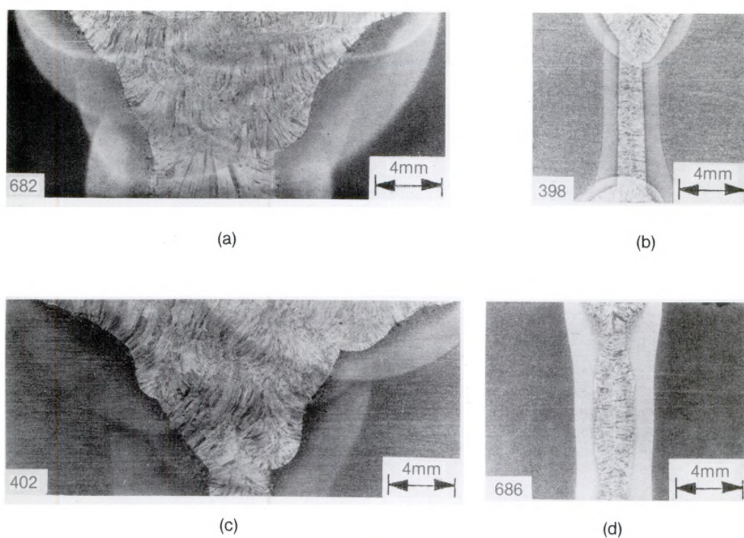
Figure 12. Cross sectional views of 0.5 in thick weldments (a) SMA weld; (b) EB weld, (c) GMA weld, and (d) LB weld.
