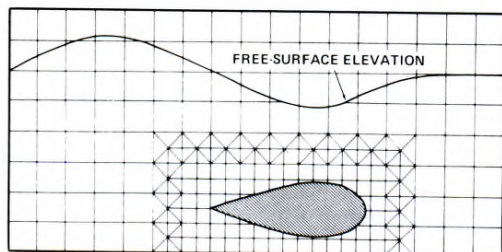
Figure 16. Finite Difference Grid System for Submerged Foil (Salvesen and von Kerczek, 1975)
