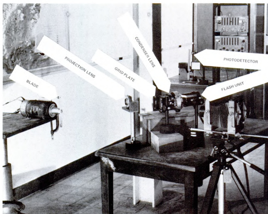
Figure 4—Experimental Setup for Propeller Rotating in Air
