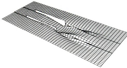
Figure 6. Free-Surface Elevations for Accelerating Surface Effect Ship (Unpublished)
