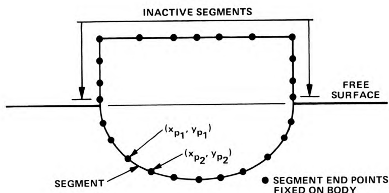
Figure 12. Body Segments for Large-Amplitude Body-Displacement Computations (Chapman, 1979)
