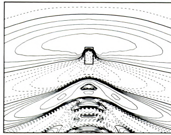
Figure 5a. Oscillating Pressure Disturbance Advancing at Froude Number, Fr = 0.40
