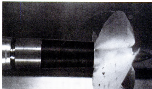
Figure 8—Propeller Inside Water Tunnel
