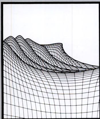
Computed breaking wave development.
