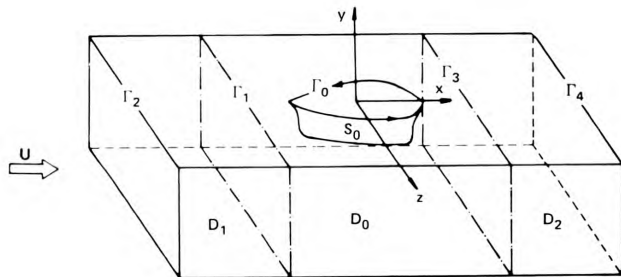
Figure 2a. The Three Subdivided Fluid Domains for the Localized Finite-Element Method
