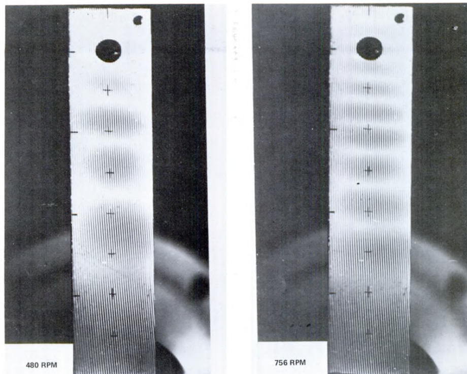
Figure 5—Deflection Fringes on Propeller Rotating in Air
