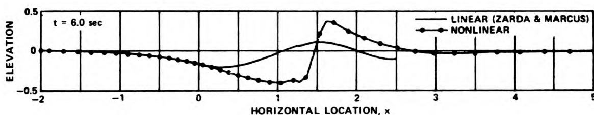
Figure 20. Nonlinear Unsteady Free-Surface Elevation for Translating Cylinder Compared with Linear Steady-State Results (Haussling and Coleman, 1977)
