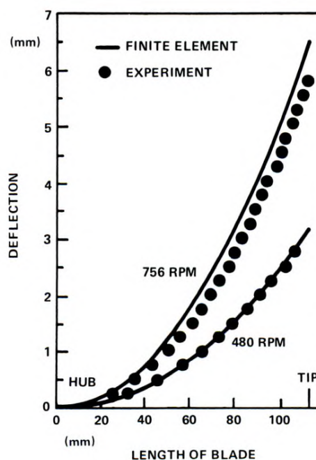
Figure 6—Blade Deflections of Propeller in Air
