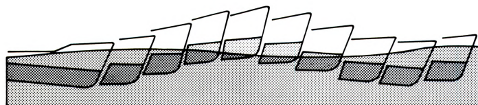
Figure 11. Bow Motion of Destroyer Hull in Sinusoidal Wave with Wavelength, \lambda = 1.20L , Wave Height, H/\lambda = 0.013 , and Froude Number, F_n = 0.35 (Salvesen, 1978)
