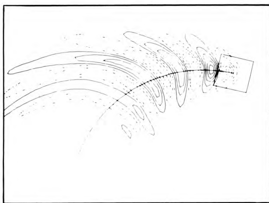
Figure 7. Wave Elevations Generated by an Air Cushion Vehicle Moving over Calm Water (Haussling and Van Eseltine, 1976a)
