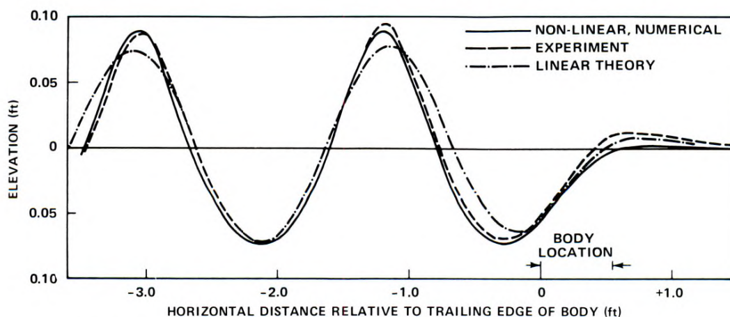
Figure 18. Comparison of Experimental, Theoretical, and Numerical Free-Surface Elevations for Submerged Foil Advancing at U = 3.18 ft/sec (Salvesen and von Kerczek, 1975)
