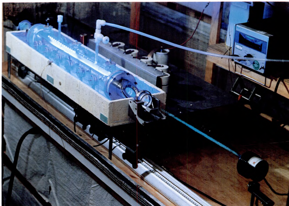
Figure 4. Naval Research Laboratory Raman-Downshifted Xenon Chloride Laser—In this arrangement an invisible beam of 308 nm UV radiation leaves the xenon chloride laser cavity through its gimbaled output mirror (small doughnut-shaped object in upper left of photograph). This UV beam enters a heated lead-vapor cell that is mounted in a firebrick-oven assembly (large white rectangular box). Stimulated Raman Effect in the lead vapor frequency-downshifts the UV radiation, producing a blue light-beam. This beam leaves the lead-vapor cell, through a water-cooled quartz window, and strikes a remote translucent glass plate (lower right of photo). A UV-to-blue down-conversion efficiency of over 50 percent has been achieved using this arrangement.
