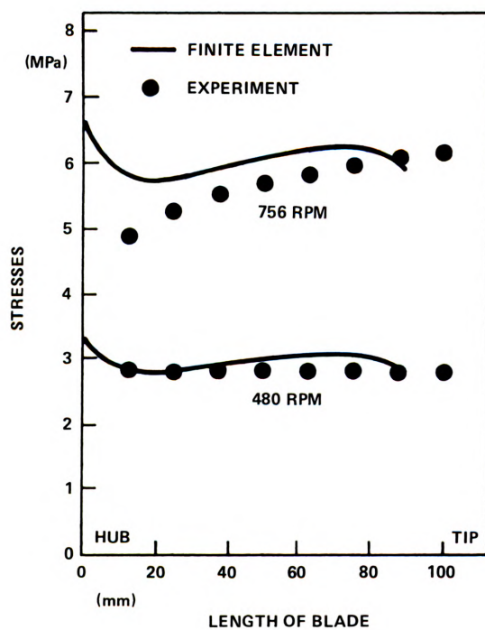
Figure 7—Blade Stress of Propeller in Air
