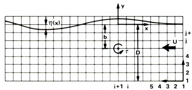
Figure 14. Finite Difference Grid for Submerged Vortex Case (Salvesen and von Kerczek, 1976)
