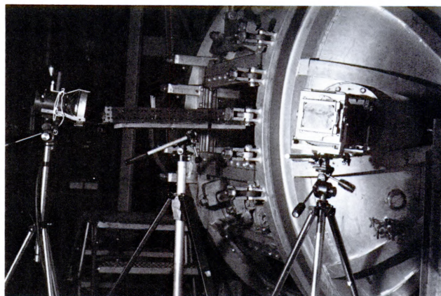
Figure 9—Experimental Setup at Water Tunnel
