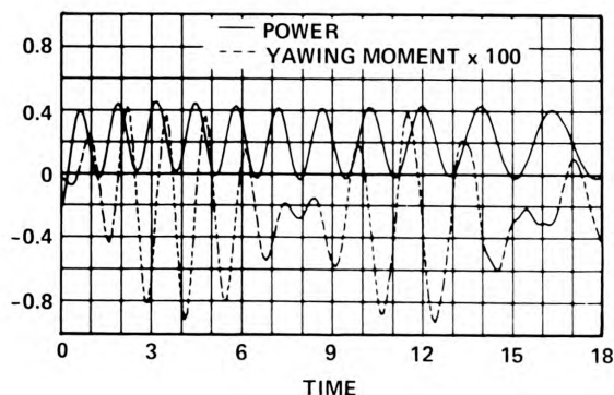
Figure 8. Yawing Moment and Power versus Time for an Air Cushion Vehicle Moving over a Disturbed Sea (Haussling and Van Eseltine, 1976a)
