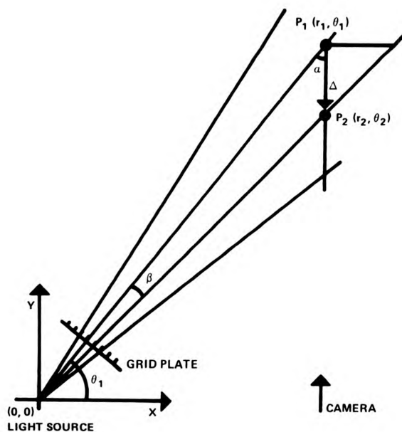
Figure 2—Schematic of Projected-grid Method
