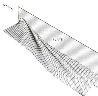
Figure 9. View of Free Surface for Plate Yawed to Starboard (Chapman, 1976)
