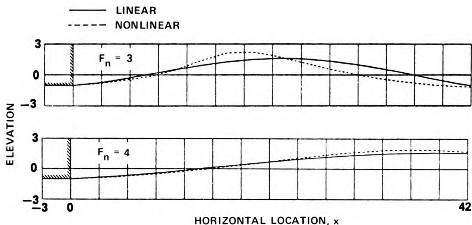
Figure 19. Linear and Nonlinear Waves behind a Transom Stern at F_n = 3 and F_n = 4 (Haussling, 1979)
