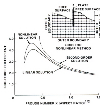
Figure 10. Linear, Second-Order, and Nonlinear Solutions for Side-Force Coefficients for Yawed Plate (Chapman, 1976)
