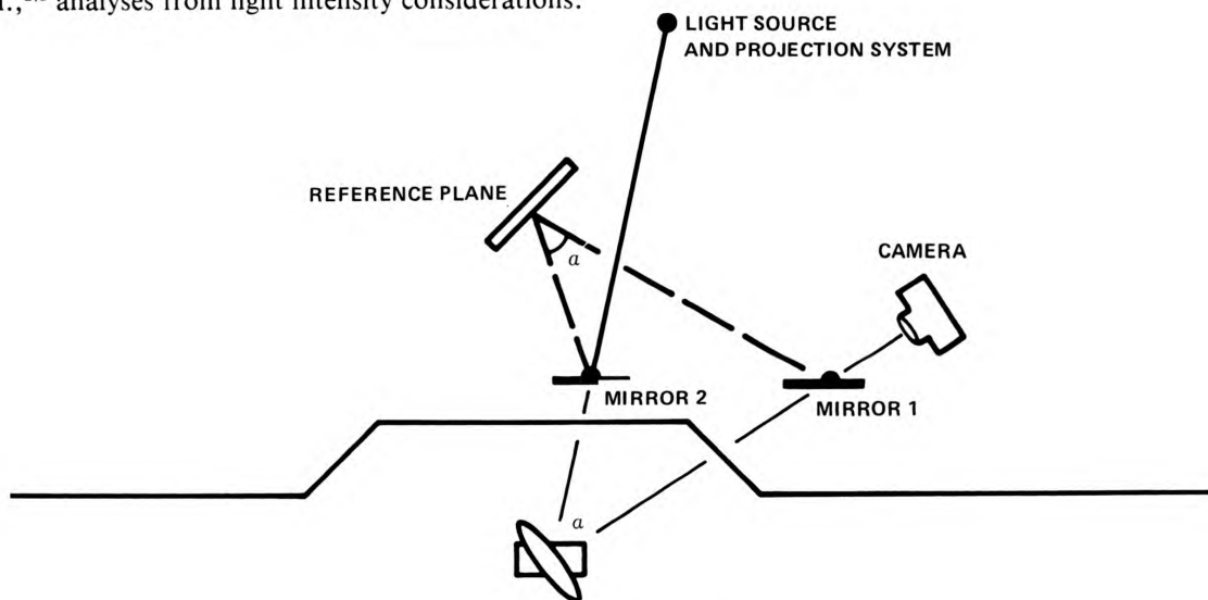
Figure 3—Contour-Difference Setup
