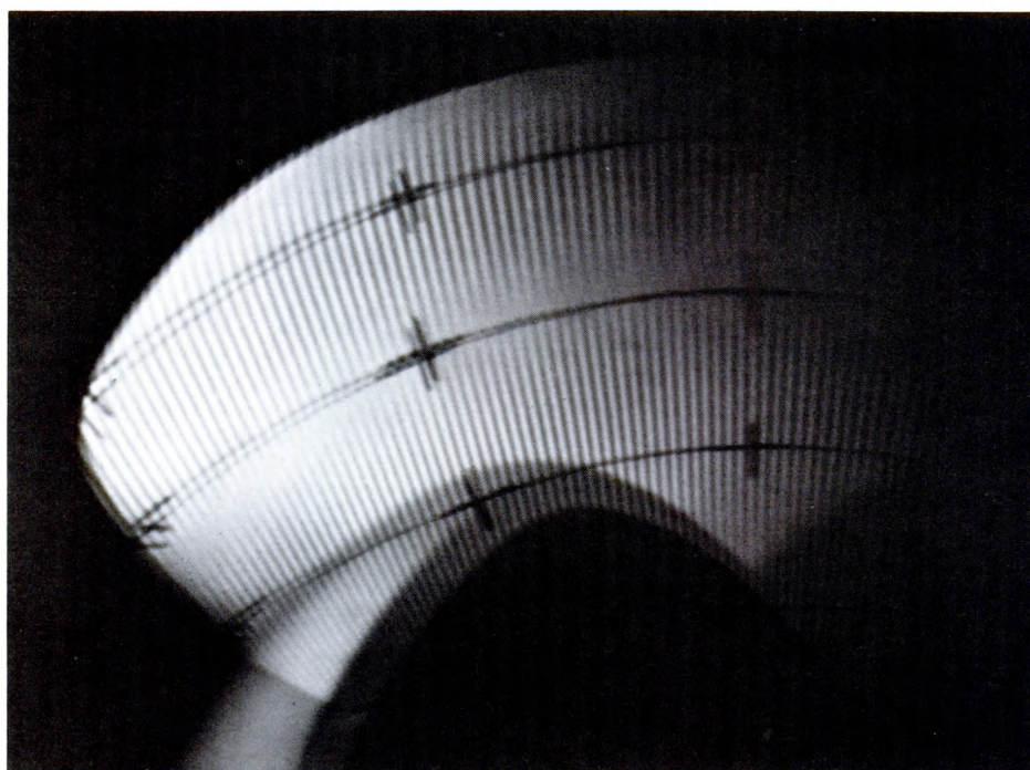
Figure 10—Deflection Fringes on Propeller Rotating Underwater
