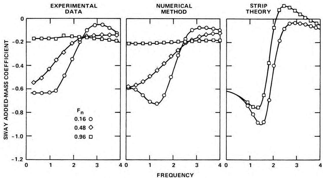
Figure 4. Flat Plate Sway Added-Mass Coefficients (Chapman, 1975)
