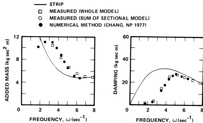
Figure 3. Pitch Added-Mass and Damping Coefficients for Series 60 Model, C_B = 0.70 at F_n = 0 (Chang, 1977)
