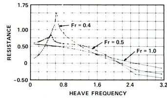
Figure 5b. Resistance for Three Froude Numbers
