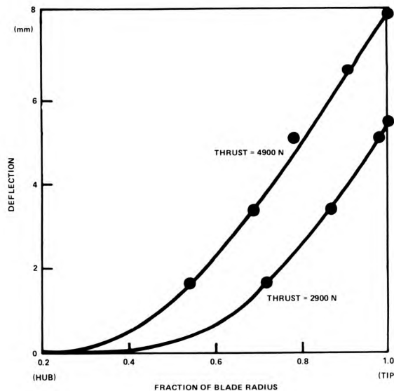
Figure 11—Blade Deflections of Propeller Rotating Underwater
