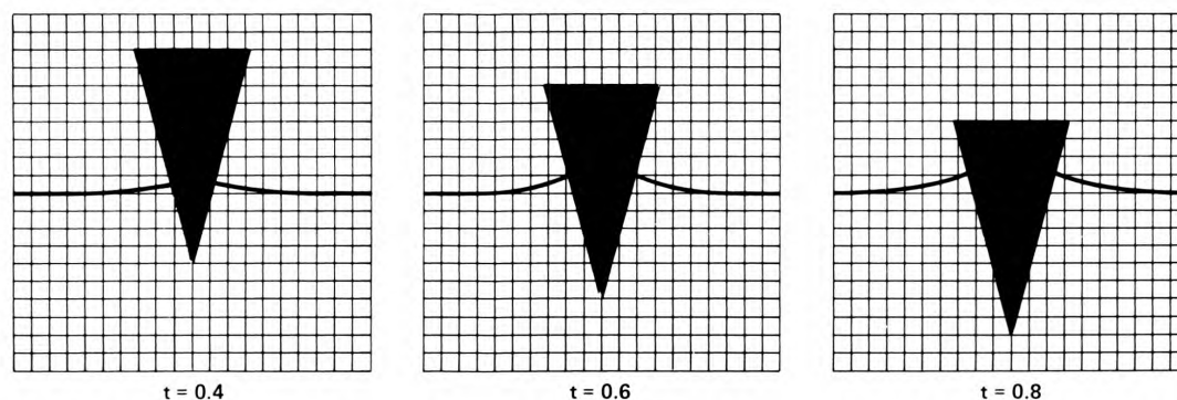
Figure 13. Free-Surface Elevations for Wedge Entry, Half-Angle, \psi = 15^\circ (Chapman, 1979)
