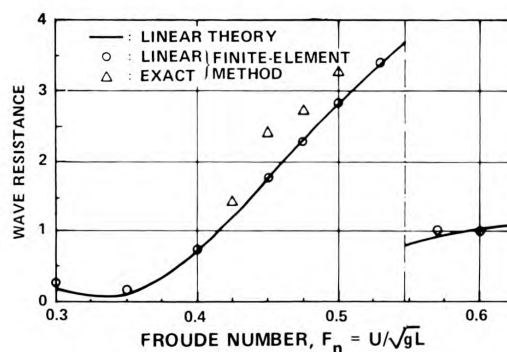
Figure 2b. Wave Resistance of a Wigley Parabolic Ship in a Canal
