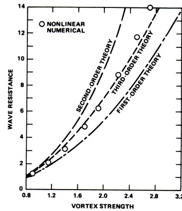
Figure 15. Wave Resistance as a Function of the Strength of Submerged Vortex Advancing at Constant Speed (Salvesen and von Kerczek, 1976)
