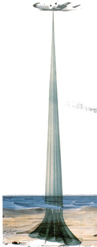
Figure 1. Aircraft-Borne Lidar Hydrographic System Operation—5 ns pulses from a 400 pps, 2 mJ/pulse green laser are projected from a small aircraft onto the ocean in a scan pattern. Pulse reflections from the surface and bottom are detected, using an aircraft-mounted PMT/Logamp, and water slant-depth is determined from the difference in platform-to-surface and platform-to-bottom optical pulse transit times. Aircraft horizontal coordinates are determined using standard electronic positioning equipment with RF-emitting shore stations.
