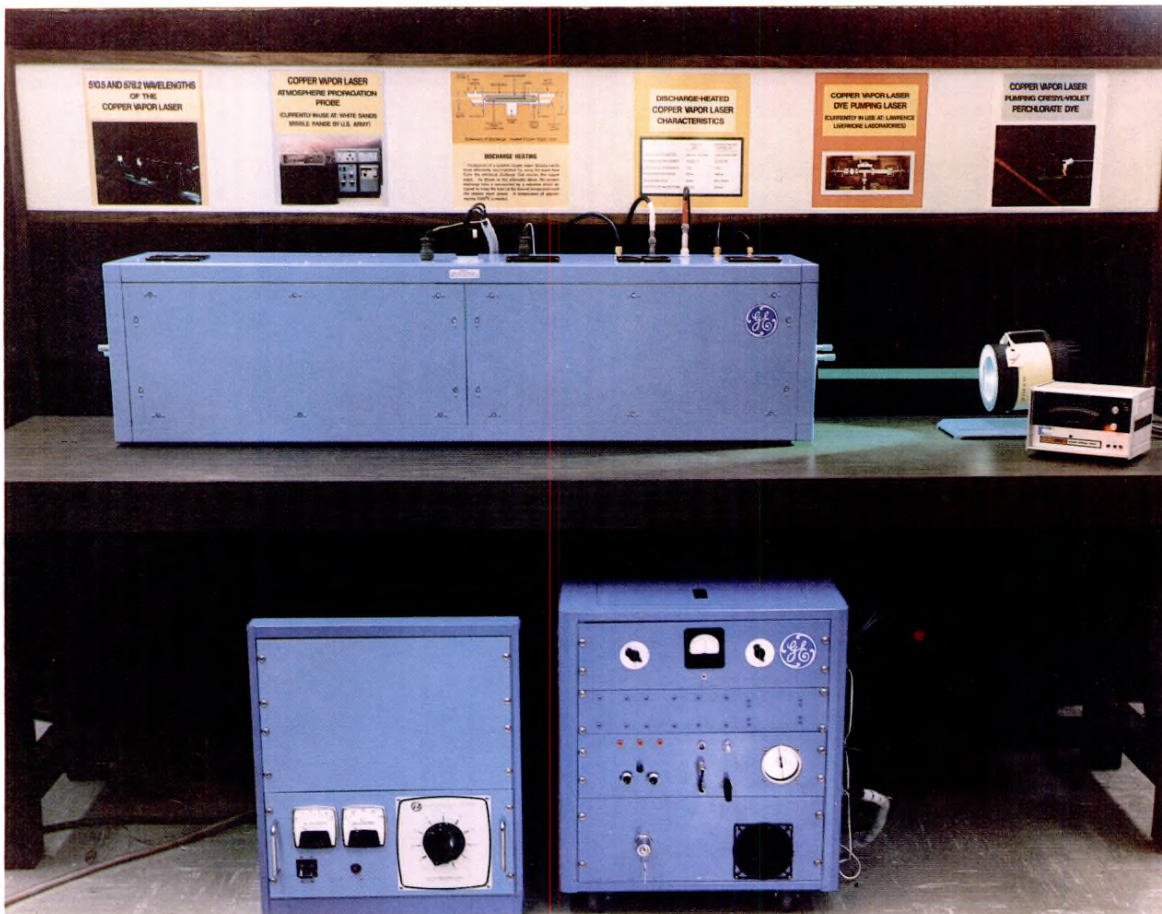
Figure 2. General Electric Company Model 6-15 Copper Vapor Laser—This commercial laser produces 15W of average optical output power at a 6kHz PRF with a maximum input electrical power consumption of 3KW. Output pulse width is 30 ns. In the photograph, the green 2.3 cm diameter output beam from the laser is shown impinging upon a power-meter. All the auxiliary electrical drive equipment necessary for operating the laser is stowed under the laboratory bench.
