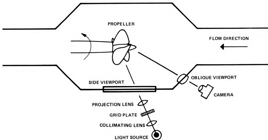
Figure 1—Optical Setup at Water Tunnel
