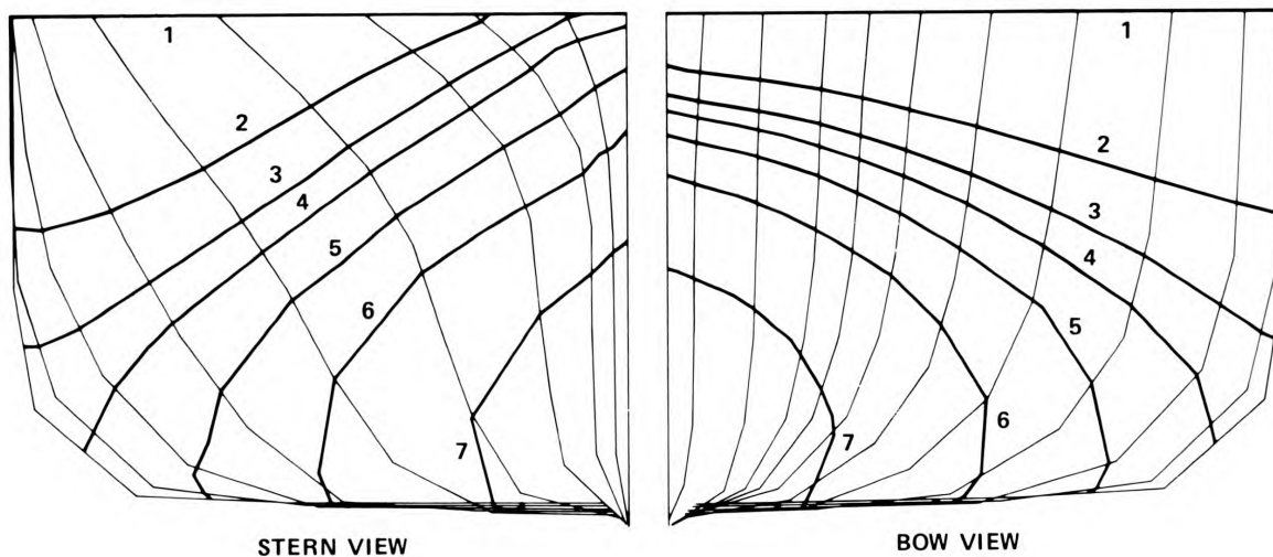
Figure 1. Streamlines on Hull Surface of a typical high-speed cargo ship at F_n = 0.35 (Dawson, unpublished)
