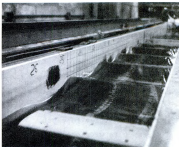
Figure 17. Experiment for Foil Advancing at U = 3.5 ft/sec (Salvesen and von Kerczek, 1975)
