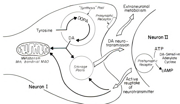
Figure 3. Schematic of the junction between two nerve cells in which dopamine is a transmitter.
