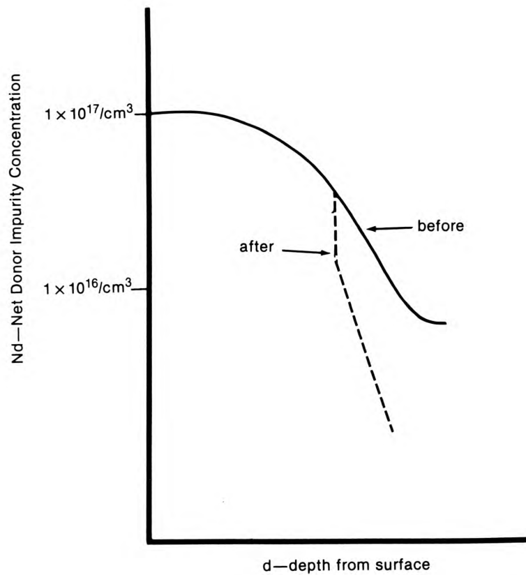
Improved Channel Pinch-off by Cr Complexing
