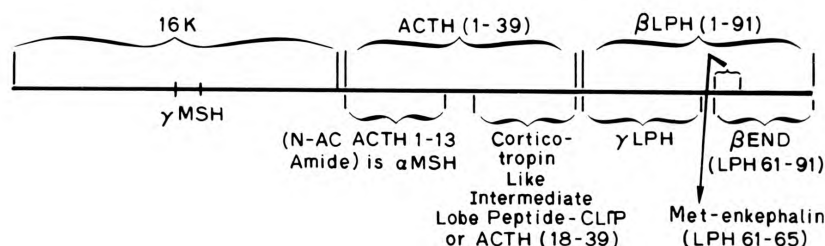
Figure 6. Neuropeptides under investigation in the Pritzker Laboratory. The relationships of some of these related peptides are shown by their common origin from a large precursor peptide. The
