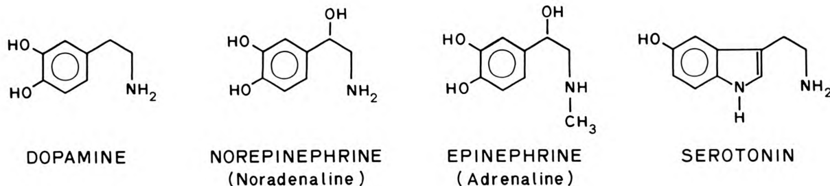
Figure 1. Chemical structures of some of the biogenic amine neurotransmitters and hormones under study.
