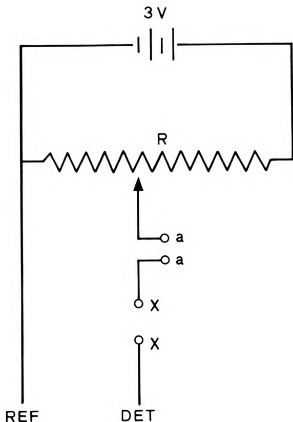
Figure 2. Circuit design for electrochemical detector used in analytical procedures. The detector is coupled to a high pressure liquid chromatography system and utilizes a reference and detector electrode. R - resistor; a, a - current measuring device; x, x - current offset connections.
