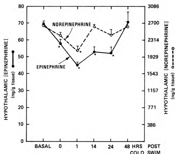
Figure 5. Changes in brain epinephrine and norepinephrine during a 48-hour period after a three minute cold water swim stress.
