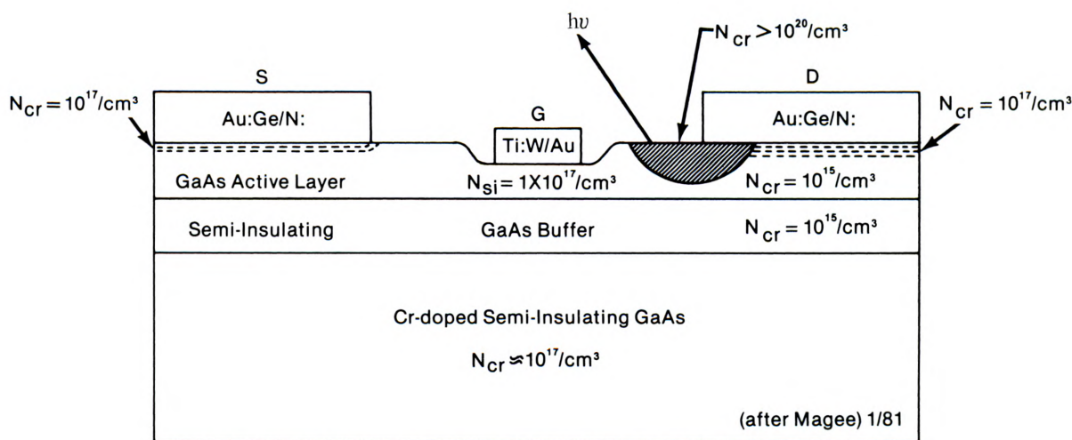
Spatial Distribution of Chromium Concentration after GaAs Power FET Failure
