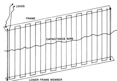
Figure 3. "Harp" wave gauge, with a wire strung in parallel runs. Resonant wave contour shown.
