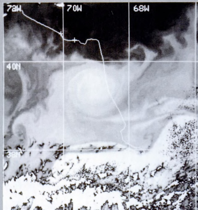
Figure 11. TIROS-N thermal infrared image for 15 June 1979 magnified about the warm core ring shown in the CZCS chlorophyll image, Figure 10. Warm temperatures are lighter, cooler darker. Line denotes ship track.
