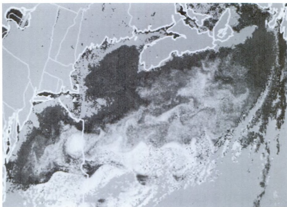
Figure 9. NIMBUS-7 CZCS derived chlorophyll image for 15 June 1979, orbit 3226. Lighter shades denote lower values, darker higher (from Gordon et al., 1982).
