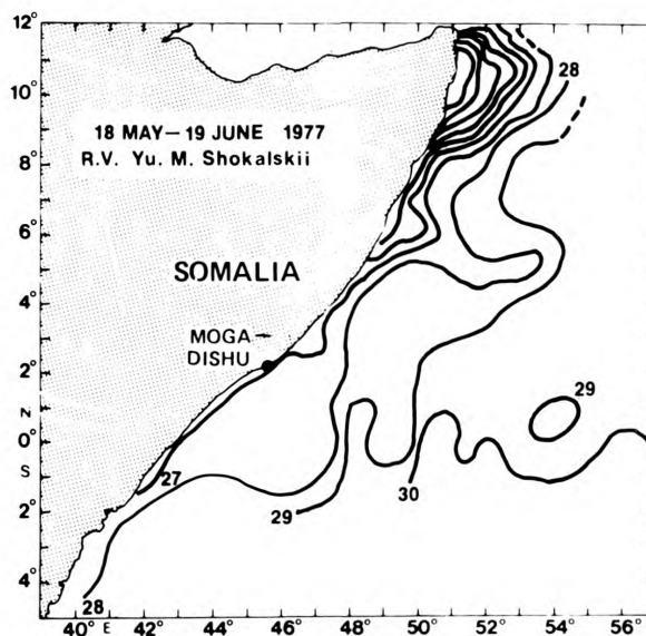
Figure 16. Surface temperature map derived from measurements made onboard the R/V Shokalskii during May-June, 1977 off Somalia. (from Evans and Brown, 1981, courtesy Dr. D. Johnson).
