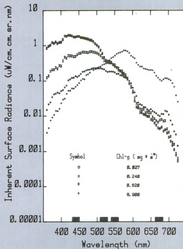
Figure 3. Upwelled light spectral sensitivity to suspended materials (from Gordon and Clark, 1980). 47
