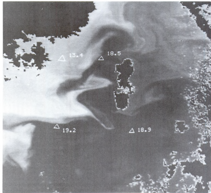
Figure 6. An electronic expansion of the vicinity of Korea Strait from the previous 8 November overpass. This subscene includes Korean coast to the northwest, Tsushima Islands in the center, and clouds plus other Japanese islands to the southeast. Sea-surface temperature patterns show Tsushima Warm Current waters interleaved with the cold waters of the coastal region.
