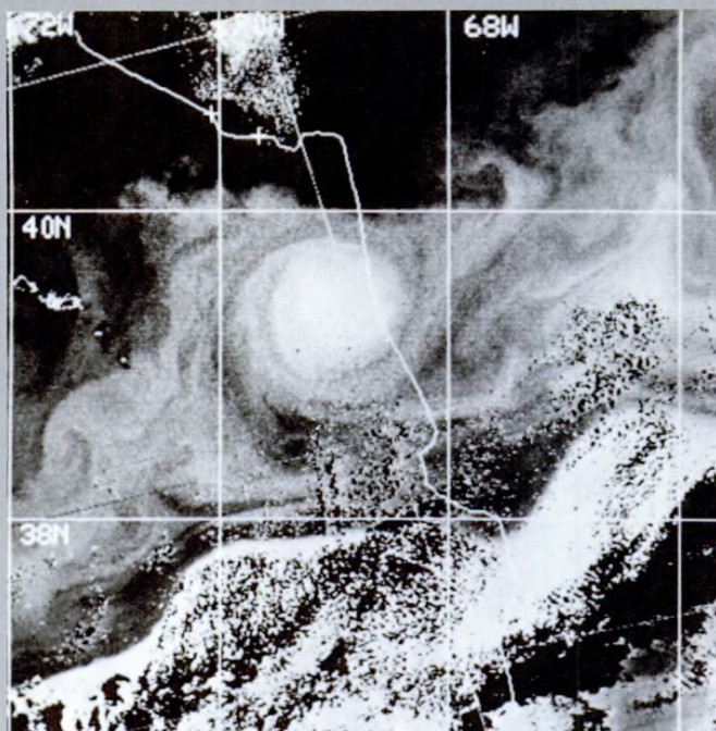
Figure 10. 15 June 1979 CZCS-derived chlorophyll image magnified about a warm core ring found at 39° N., 69° W. Line indicates ship track.
