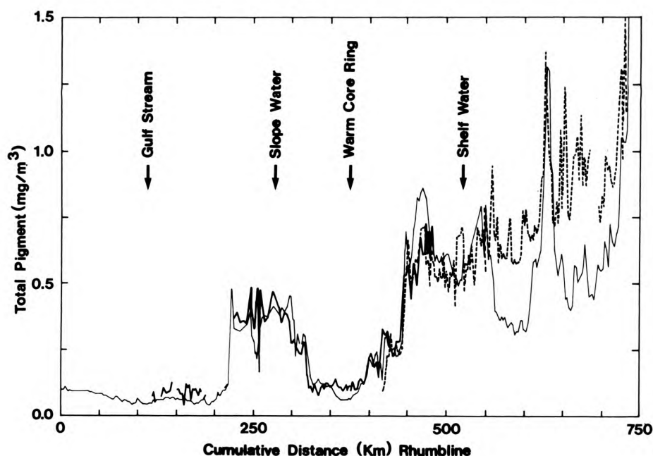
Figure 12. Comparison of ship and satellite derived surface pigment concentrations for NIMBUS-7 orbits 3157 and 3171, and R/V Athena II in-situ observations. Ship observations are denoted by the light line, satellite observations by the heavier solid and dashed lines, orbits 3157 and 3171 respectively (from Gordon et al., 1982).
