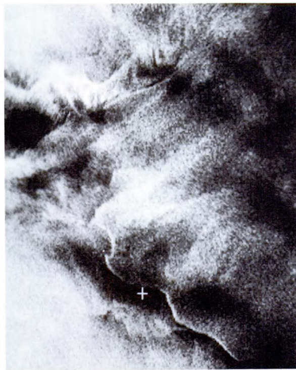
Figure 2. Magnified portion of Figure 1., showing the shear instability of a current edge shear layer.
