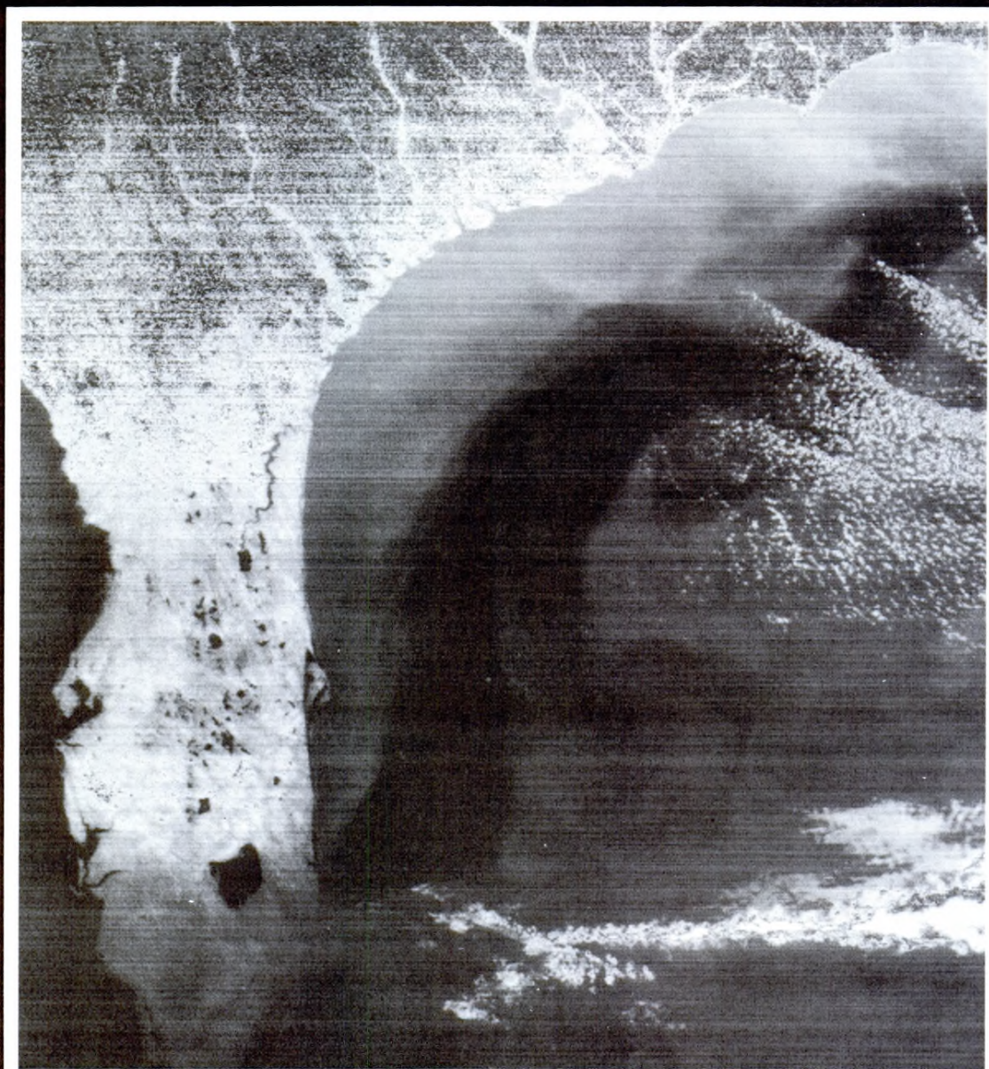
Figure 1. NOAA-4 satellite infrared image (10.5-12.5 \mu\text{m} ) of the Florida Peninsula, Gulf Stream, and shelf waters, 0100Z, 4 April 1975. At the latitude of Lake Okeechobee, a nearly cloud-free atmospheric front occurs between cooler, dry continental air to the north and warm, moist air to the south.
