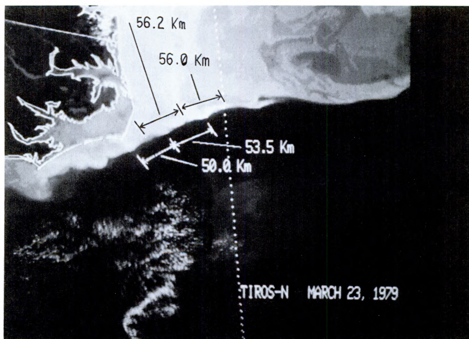
Figure 8. The edge of the Gulf Stream beyond Cape Hatteras, showing shear waves (from TIROS-N, AVHRR Data).
