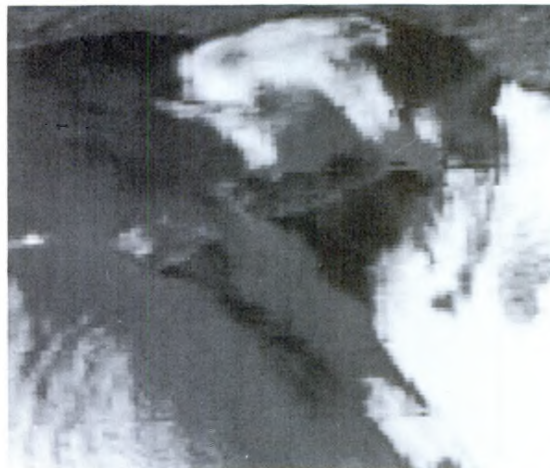
Figure 1. Anomalous Gray-Shade Features in the Wake of Santa Rosa and Santa Cruz Islands off of Santa Barbara, California as Observed by the NOAA-6 Advanced Very High Resolution Radiometer (AVHRR) on 28 September 1980.
