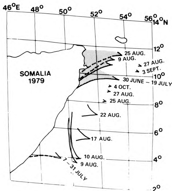
Figure 14. Time sequence of satellite observed frontal locations for northern and southern frontal wedges for year 1979. The northern wedge front is hatched (from Evans and Brown, 1981). 48
