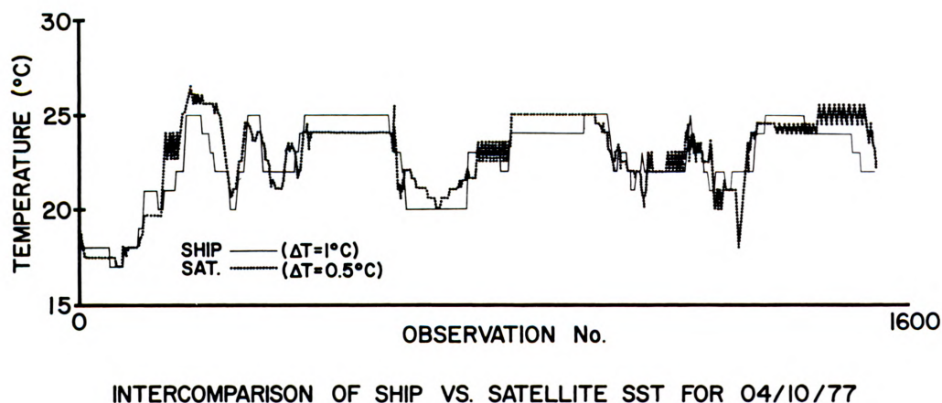
Figure 8. Satellite versus ship derived temperature intercomparison.
