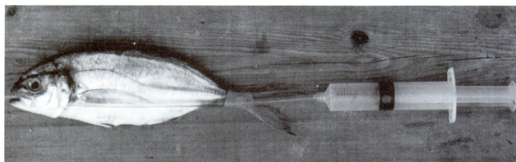
Figure 1. Feeding bioassay: a 20 cm long blue runner, Caranx crysos , is prepared as a bait by attaching a 25 ml syringe to the fish. The plastic tube extends out the bait's mouth.
