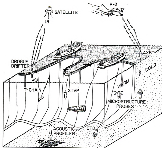
Figure 1. A schematic of the FRONTS-80 field program in the North Pacific Subtropical Front. This picture should be viewed together with Table I where the participants and techniques are identified.
