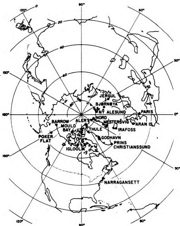
Figure 13. Sites of the Arctic Air-Sampling Network in 1980. 25
