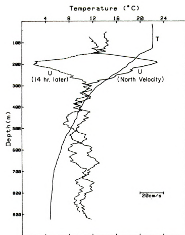
Figure 1. Profiles of temperature and velocity obtained with an Expendable Current Profiler (XCP). The temperature record shows many fluctuations in gradient over scales of meters to tens of meters. These are referred to as finestructure. The velocity structures are primarily due to low frequency internal waves, known as inertial motions. The dotted profile was taken approximately one-half an inertial period after the solid curve, showing a reversal in most of the velocity structures, which identifies them as inertial. These data were kindly supplied by T. Sanford and E. Kunze of the Applied Physics Laboratory, University of Washington.
