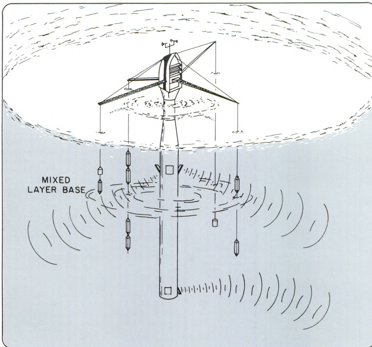
FLIP with instrument booms extended
