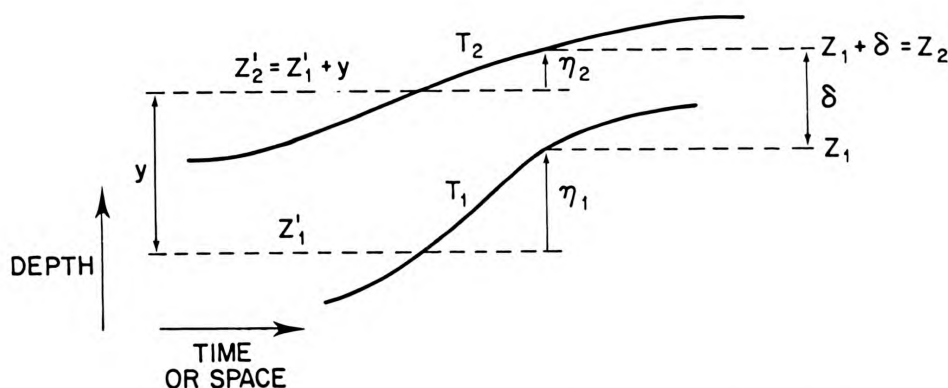
Figure 13. Schematic showing the positions of two isotherms, T_1 and T_2 . The isotherms have been displaced by \eta_1 and \eta_2 from their equilibrium positions, Z_1' and Z_2' , respectively. The instantaneous gradient measured between Z_1 and Z_2 is (T_2 - T_1)/\delta , which is greater than the average gradient, (T_2 - T_1)/y . 4
