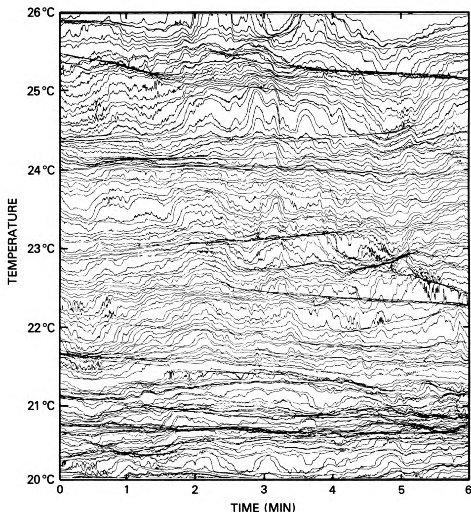
Figure 11. Temperature traces from the topmost 80 m of the Naval Research Laboratory (NRL) chain. The speed was 2.5 m/s, corresponding to 150 m/min. Regions of large gradient are shown by increased distances between traces, while low gradient sections appear with large separations. (The plot was kindly supplied by E. E. Rudd and B. S. Okawa of NRL.)
