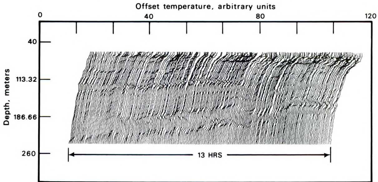
Figure 12. A 13-hour long time series of temperature profiles. Successive profiles have been offset for display. High gradient features can be seen to migrate vertically with time. The movement is upward with respect to temperature, as well as pressure, indicating that the features must be due to internal wave strain. 11
