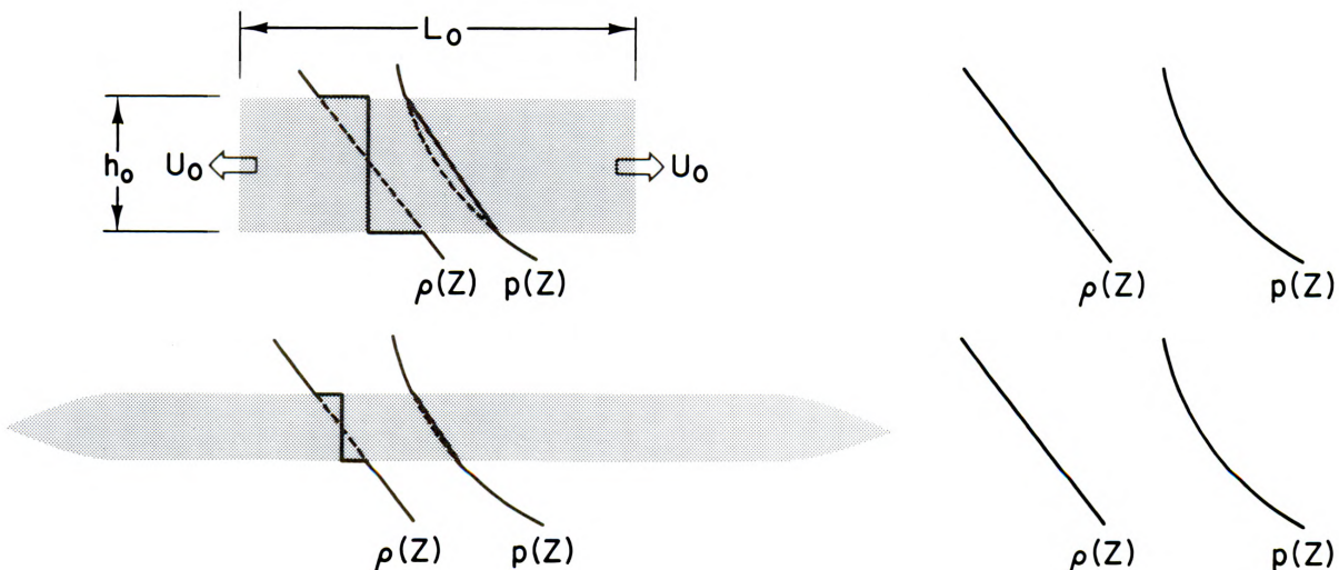
Figure 8. Schematic of the gravitational collapse of a fully mixed region in the thermocline, which is initially h_0 meters high and L_0 meters across. The initial density profile, \rho(Z) , was linear, as shown at the right. The spreading motion is driven by the horizontal pressure gradient, which results from the mixing. This gradient is shown by the separation of the dotted and solid pressure curves, p(z) , through the layer.
