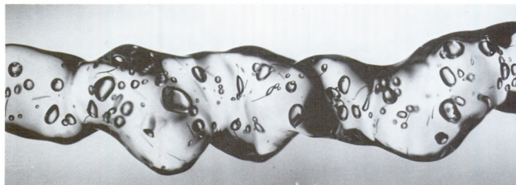
Figure 9. Enhancement of the helical phase of water jet flow.
