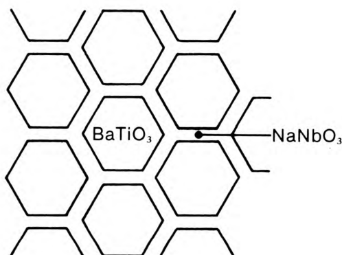
\text{BaTiO}_3 GRAINS \text{NaNbO}_3 2ND PHASE
