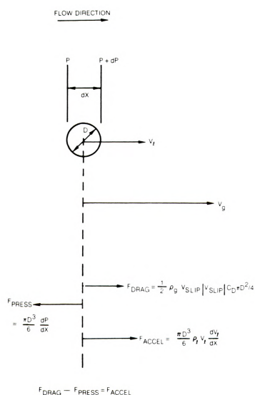
Figure 2. Force balance with drag on liquid droplet.
