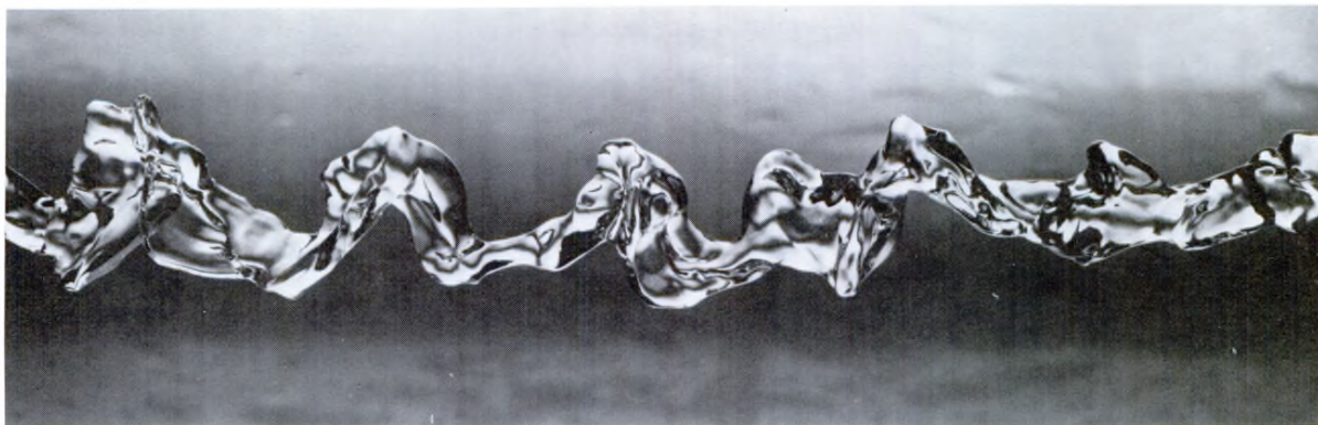
Figure 17. The helical phase becomes more exaggerated in a polymer jet, 192 diameters downstream.
