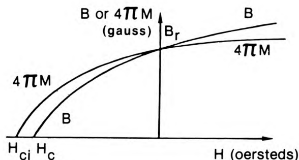
Figure 2. Schematic diagram of a section of the hysteresis loop illustrating the difference between the coercivity, H_c , and the intrinsic coercivity, H_{ci} .
