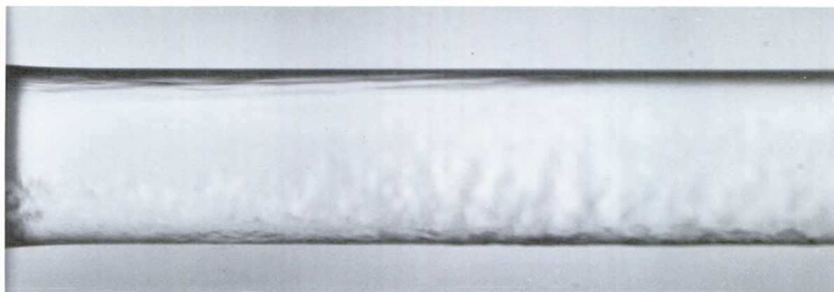
Figure 12. Water jet emerging from special design nozzle at left. The laminar flow is seen to contain growing turbulent areas inside the jet.
