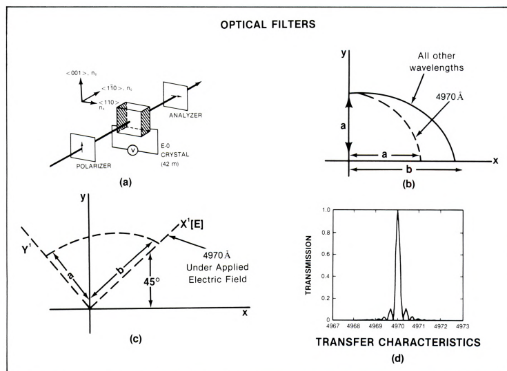
Figure 5. (a) Schematic of the optical system; (b) optical properties, isotropic a_x = a_y at 4970 Å, anisotropic a_x \neq a_y at all other wavelengths; (c) principal optic axes at 4970 Å under electric field; (d) transmission characteristics.
