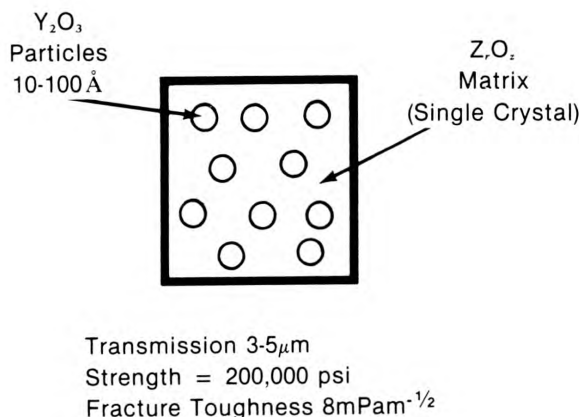
Figure 4. Schematic of Composite Optical Material, and relevant properties.
