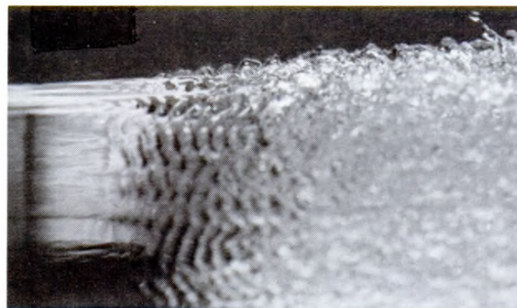
Figure 3. View of amplification of surface waves with consequent spray detachment.
