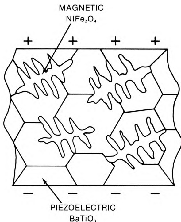
Figure 11. Composite Magnetolectric
