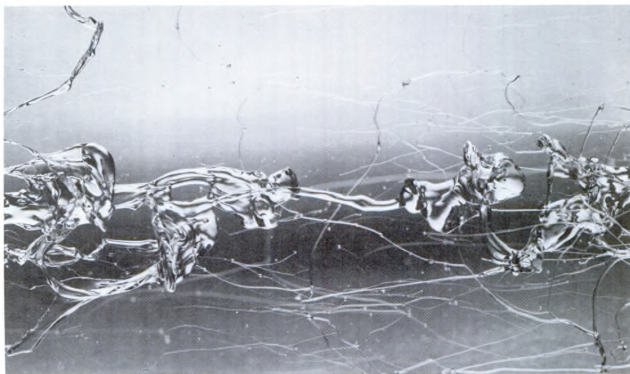
Figure 18. Breakup of polymer jet, 336 diameters downstream.
