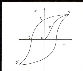
Figure 1. Schematic diagram of the hysteresis loop of a permanent magnet material illustrating the dependence of the magnetic induction B on the applied magnetic field H .
