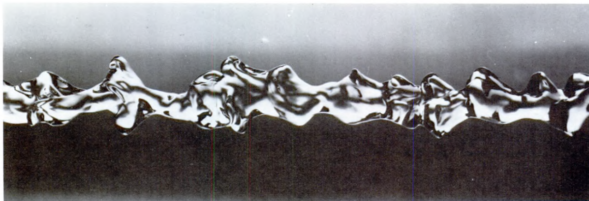
Figure 16. Helical instabilities on a 200 ppm poly(ethylene oxide) jet.
