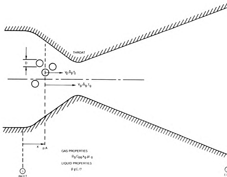
Figure 1. Governing flow parameters of two-phase nozzles.
