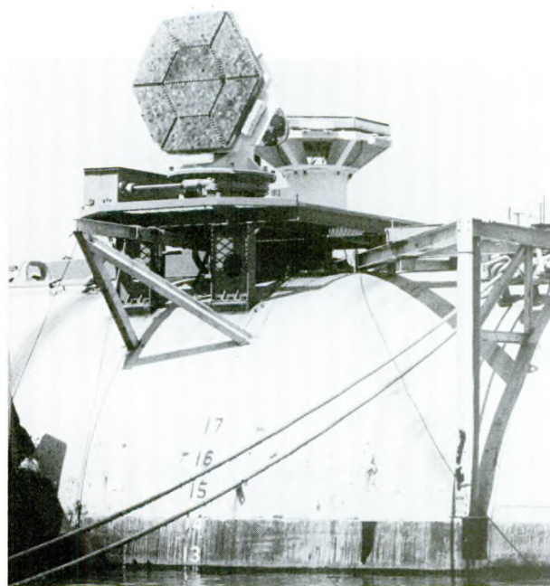
Photograph of the lower Doppler sonar installation on FLIP. When "flipped" these four sonars will be at a depth of 85 meters pointed horizontally.
