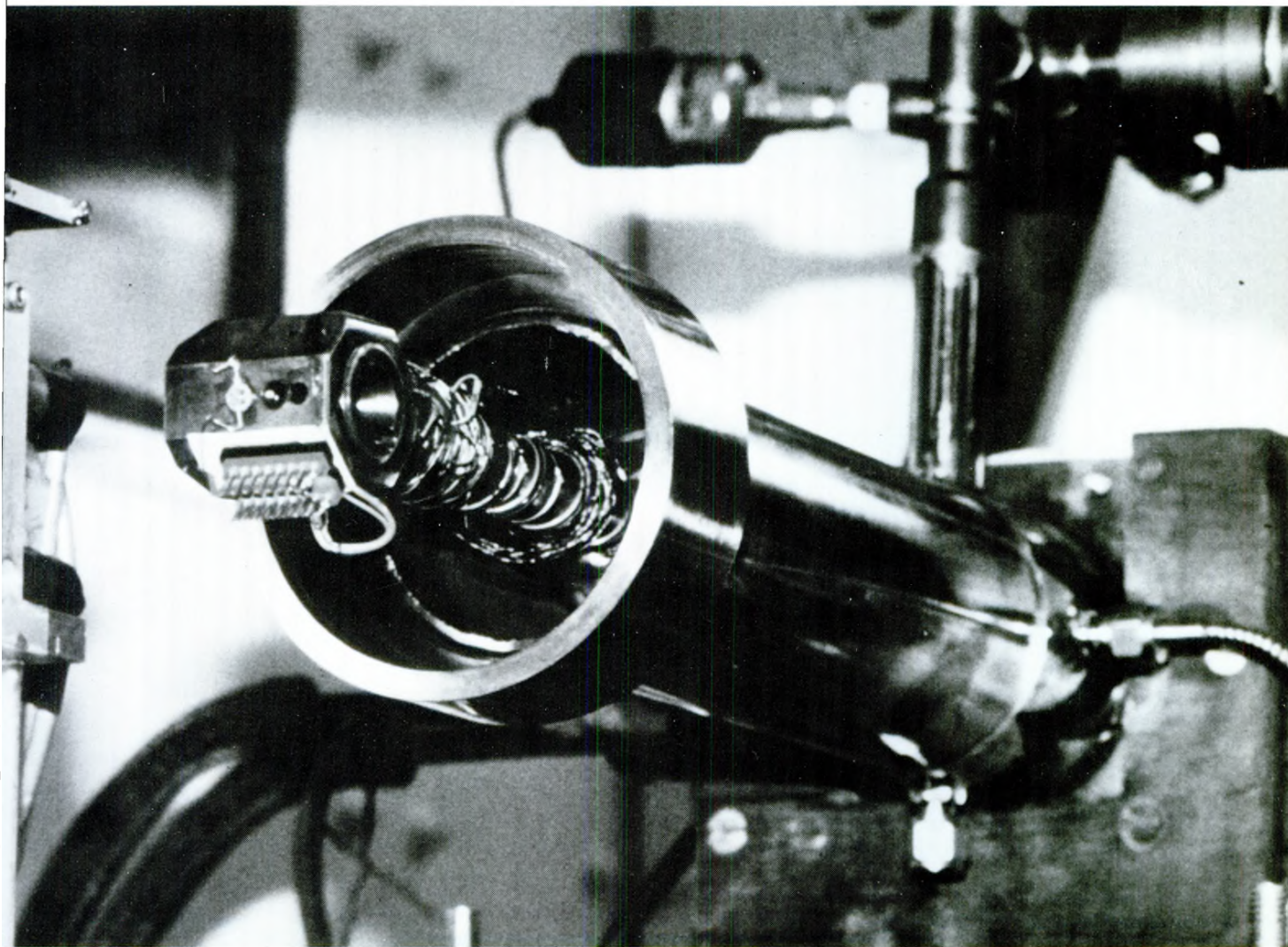
Diamond-anvil pressure cell
