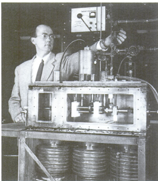
Professor Charles H. Townes is shown with the ammonia beam maser he developed in the early 1950's at Columbia University. This was the first molecular oscillator and amplifier and led to the development of the general field now called quantum electronics. This research was funded by the Office of Naval Research, the Army, and the Air Force.
