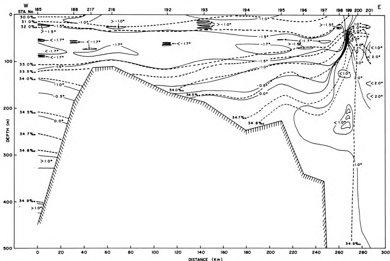
Temperature and salinity transect along 78°10'N. At this latitude and farther southward the EGPF is aligned with the upper continental slope. Warm AIW overlies much of the shelf.
