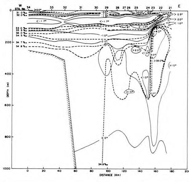
Temperature (solid line) and salinity (dashed line) transect along 79°55'N. The East Greenland Polar Front, observed by the near-vertical slope of the isotherms and isohalines, is displaced about 120 km east of the continental shelf break. The Return Atlantic Current is identified by the core of water warmer than 3°C.
