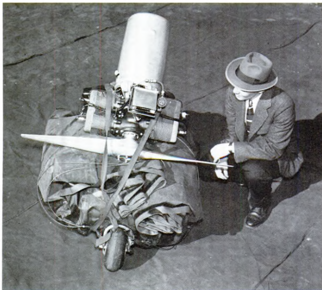
The folded up inflatoplane package
