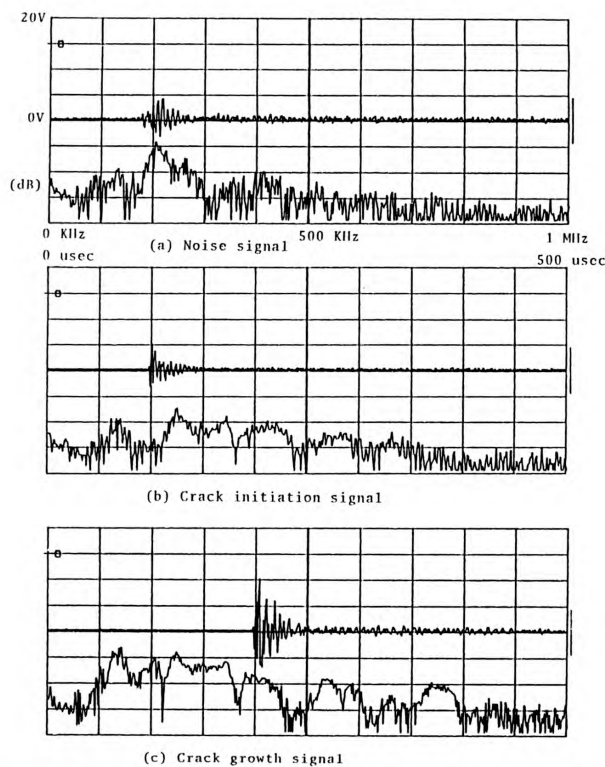
Figure V.5: DSO plots of Noise, Crack Initiation and Crack Growth
