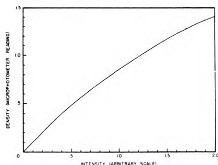
FIG. 2. Typical calibration curve for converting microphotometer readings to electron intensities.
