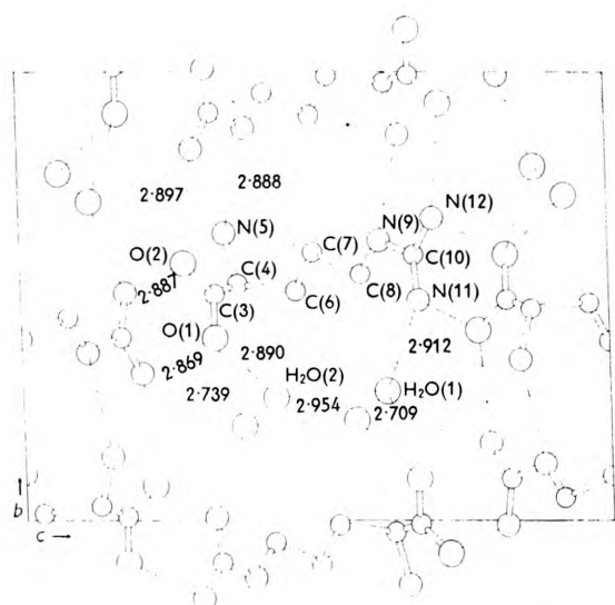
Bond Angle N(9)H(10) ··· N(5') 2·888 Å C(8)N(9) ··· N(5') 112·7° C(10)N(9) ··· N(5') 110·5 N(12)H(14) ··· O(2') 2·897 C(10)N(12) ··· O(2') 135·6 N(12)H(13) ··· O(1'') 2·869 C(10)N(12) ··· O(1'') 116·3 N(11)H(12) ··· O(2'') 2·887 C(10)N(11) ··· O(2'') 121·2 W(1)H(15) ··· O(1') 2·739 N(11) ··· W(1) ··· W(2) 101·7 N(11)H(11) ··· W(1) 2·912 N(11) ··· W(1) ··· O(1') 109·9 W(2)H(18) ··· W(1) 2·954 N(11) ··· W(1) ··· W(2') 138·0 W(1)H(16) ··· W(2') 2·709 W(2) ··· W(1) ··· O(1') 105·6 W(2)H(17) ··· O(1) 2·890 W(2) ··· W(1) ··· W(2') 78·8 W(2') ··· W(1) ··· O(1') 110·2 O(1) ··· W(2) ··· W(1) 122·4 O(1) ··· W(2) ··· W(1') 120·0 W(1) ··· W(2) ··· W(1') 116·2
