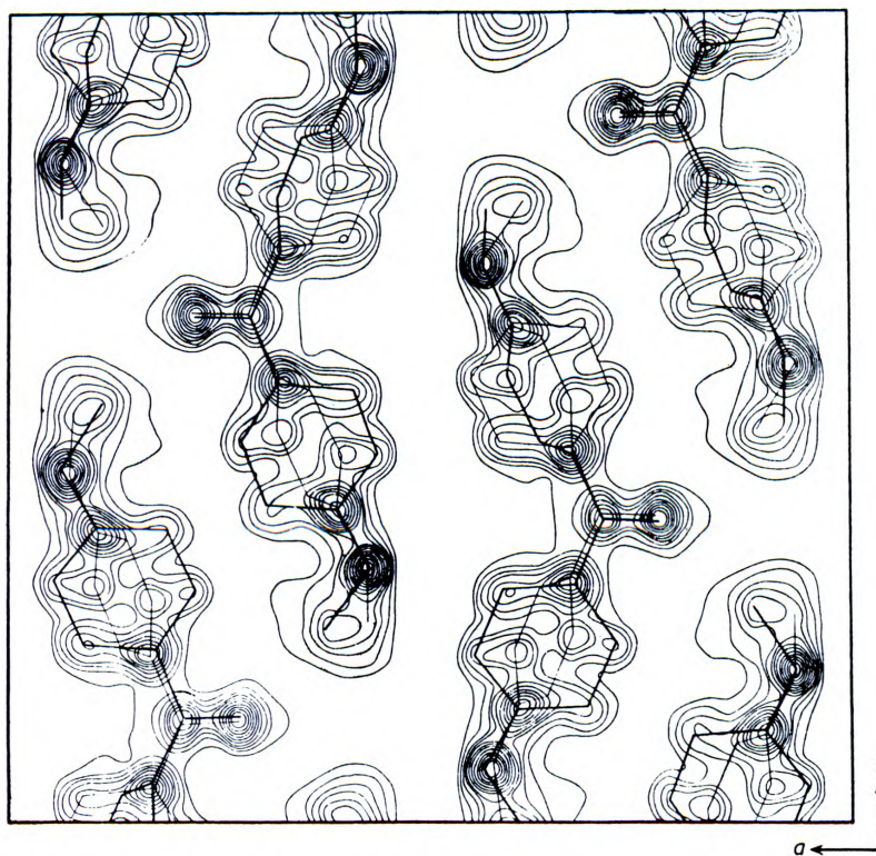
Fig. 2. Electron-density projection on (001). The pairs of superimposed molecules are separated by approximately \frac{1}{4}c . The coordinates of the line drawings were taken from the preliminary three-dimensional least-squares refinement.
