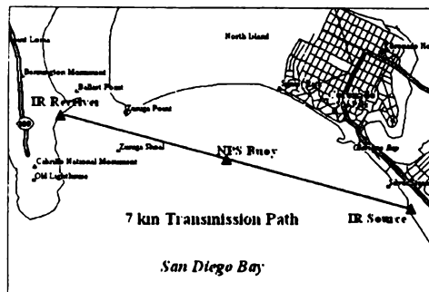
Figure 1 EOPACE experimental setup, August-September 1997.
