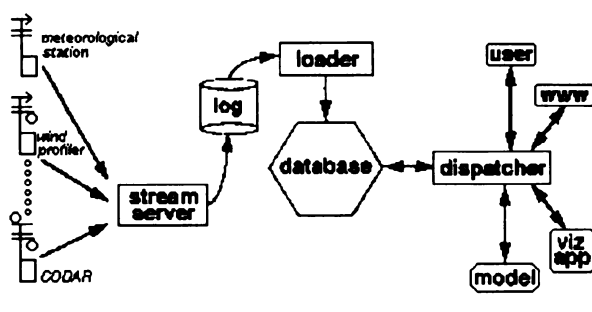
Figure 1 REINAS Logical Architecture.
