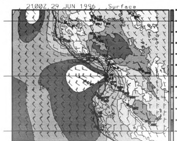
Figure 5 Mesoscale analysis for 29 June 1996 using 3D MQ with all mesonet observations.
