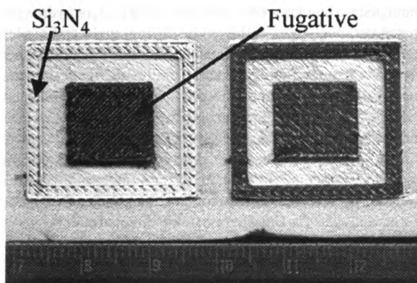
Figure 19 Multi-material structure made by direct LM (FDC) technique.
