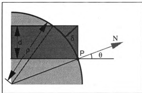
Figure 4 Circular approximation to determine layer thickness.
