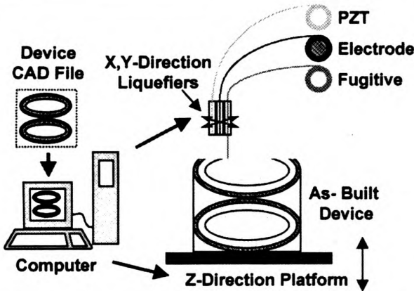
Figure 15 Schematic of multi-material LM manufacturing system.
