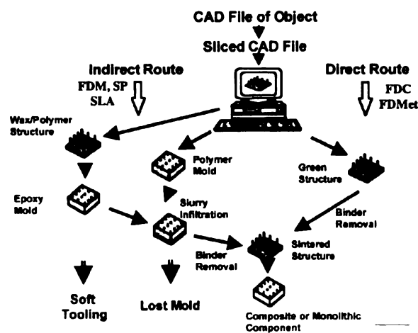
Figure 1 Schematic of direct and indirect routes of layered manufacturing.
