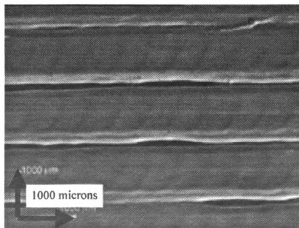
Figure 21 Optical image of the surface of a PZT sample built by the direct LM (FDC) process.
