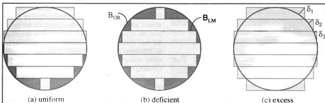
Figure 3 Different Deposition Strategies.
