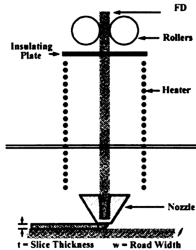
Figure 2 Schematic of the fused Deposition of Ceramics (FDC) SFF process.
