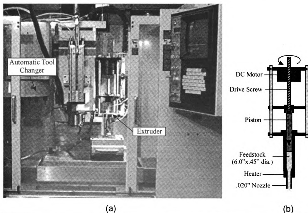
Figure 3 Integrated CNC shaping/deposition machine for SDM. (a) Fadal VMC-15 CNC milling machine with integral extruder. (b) ACR extruder.
