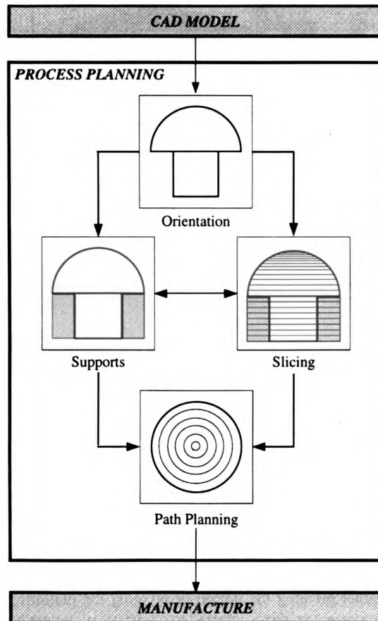
Figure 2 Process Planning for Layered Manufacturing.
