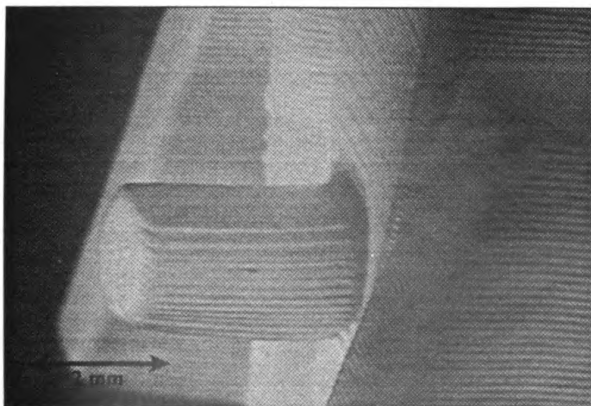
Figure 3 Close-up oblique side view of as-built UM-ONR part. Note the stairstepping effect on the center rod.
