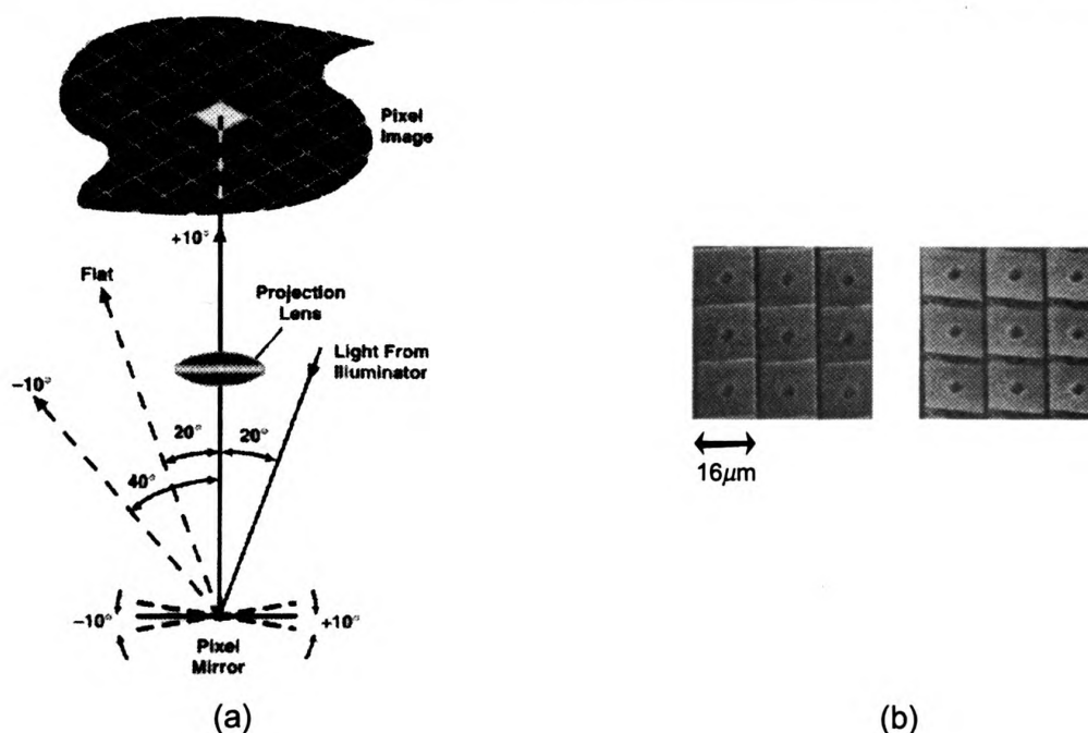
Figure 2 (a) DMD optical switching principle. (b) Operating DMD arrays.
