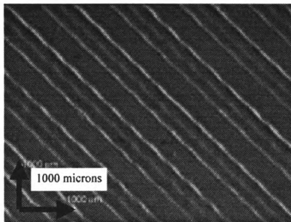
Figure 20 Optical image of the surface of a silicon nitride sample built by the direct LM (FDC) process.
