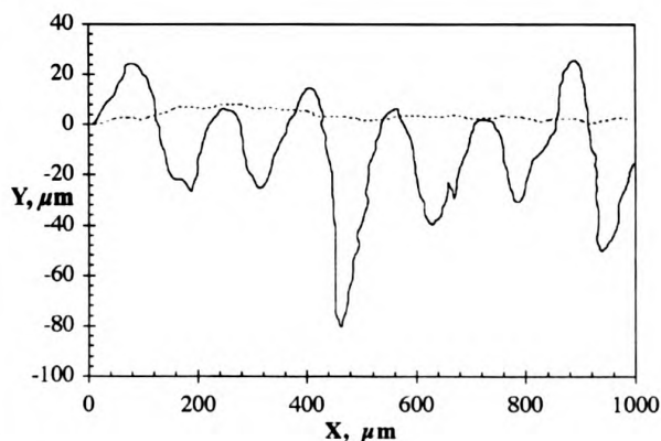
Figure 4 Profilometer scan of side and upfacing surface of an as-built part. Solid line: side scan. Dotted line: upfacing surface scan.
