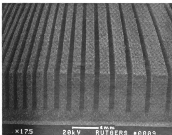
Figure 14 a) SEM micrograph of PZT structure with volume fraction gradient fabricated by indirect LM (SPI) process. b) Polymer mold, PZT part, and PZT-polymer radial composite structures fabricated by the indirect LM (SPI) process.
