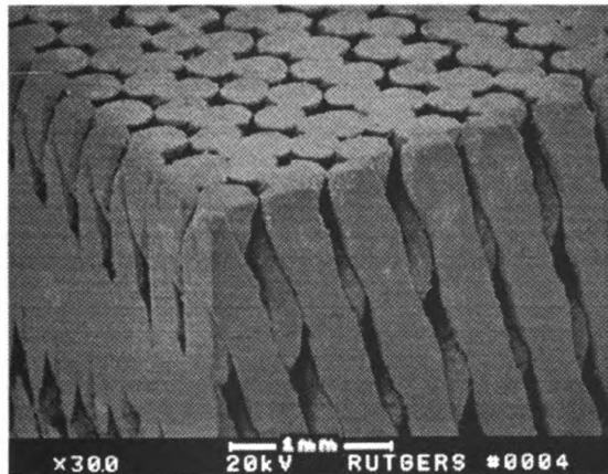
Figure 13 SEM micrograph of an oriented PZT fiber structure fabricated by direct LM (FDC) process.
