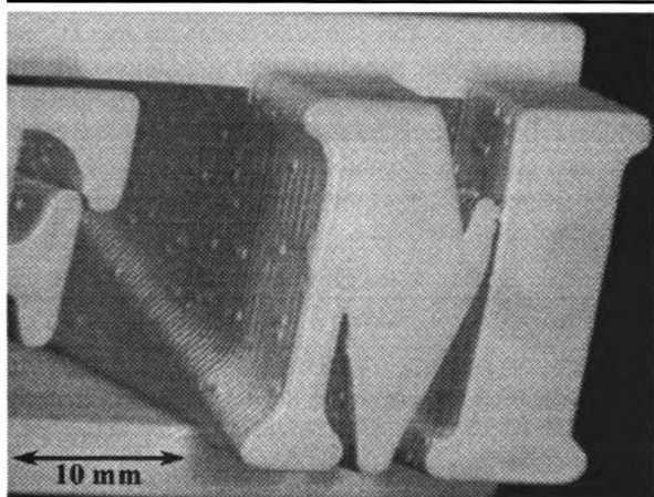
Figure 2 Close-up top view of as-built UM-ONR part. Note the smooth upfacing surface and scalloped sides.
