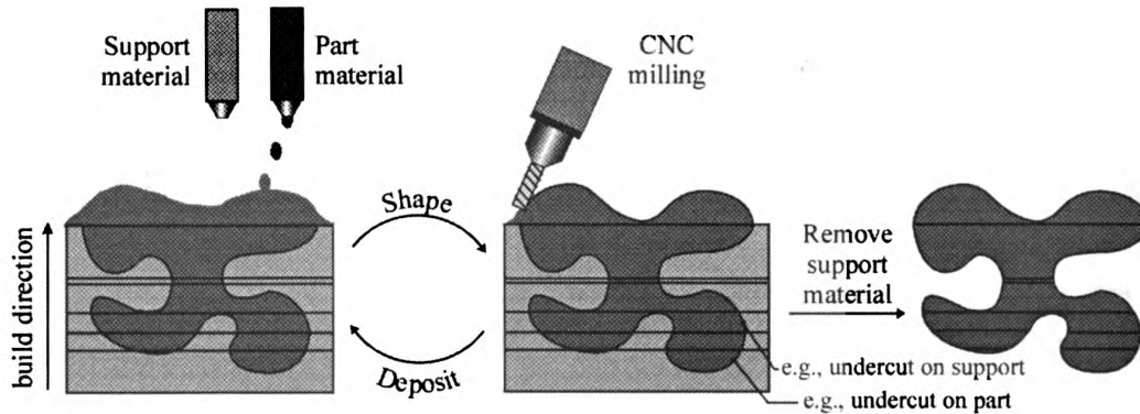
Figure 1 Shape Deposition Manufacturing.
