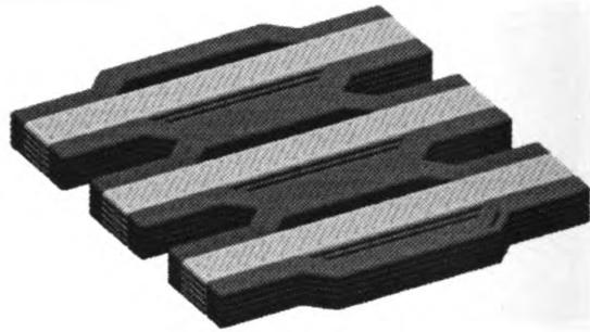
Figure 17 Virtual LM simulation of a 2-material stacked cymbal actuator structure.
