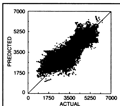
Fig. 4a - Scatter plot of damper predictions for airspeeds greater than 60 kn for the baseline data
