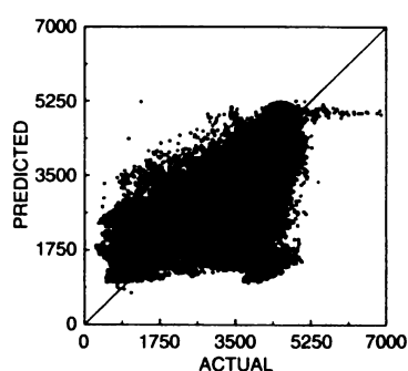
Fig. 4b - Scatter plot of damper predictions for airspeeds less than 60 kn for the baseline data
