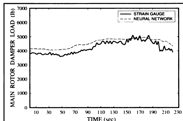
Fig. 6 - Damper load predictions for a 60° angle of bank right turn in the baseline data
