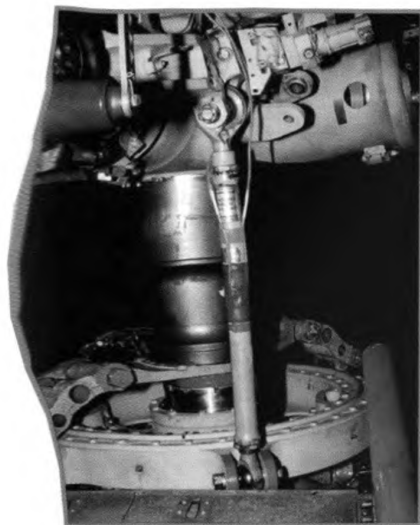
Fig. 7 - Instrumented main rotor pushrod
