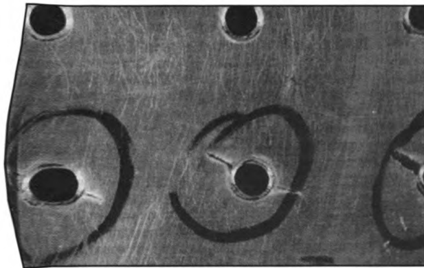
Fig. 1 - Multiple fatigue cracks found at countersunk fastener holes during a teardown inspection of a US Air Force KC-135 tanker aircraft. (The cracks can be seen extending from each of the circled holes at the 10 o'clock and 4 o'clock positions.)
