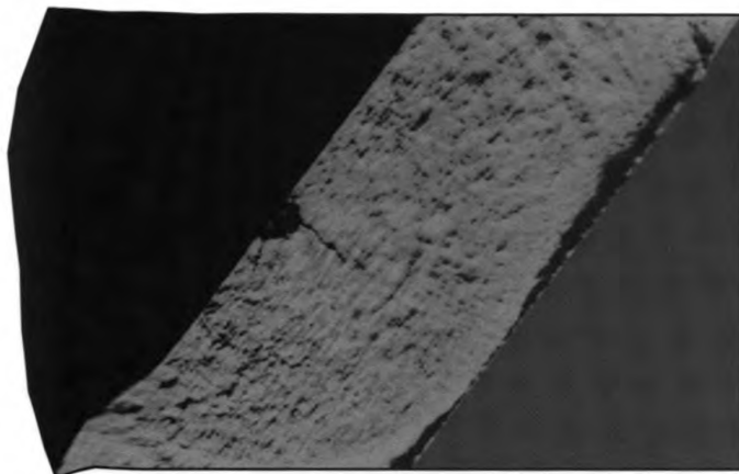
Fig. 5 - The fatigue crack that led to the failure of this component initiated at the active corrosion pit shown at the left center of the photograph
