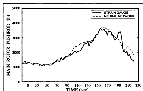
Fig. 5 - Pushrod load predictions for a 60° angle of bank right turn in the baseline data
