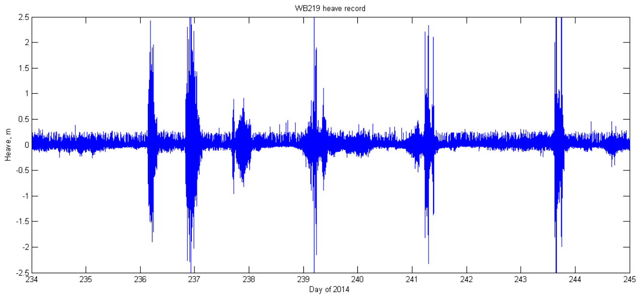
Figure 4: A more detailed view of 11 days heave record from WB219 (Cluster 1)
